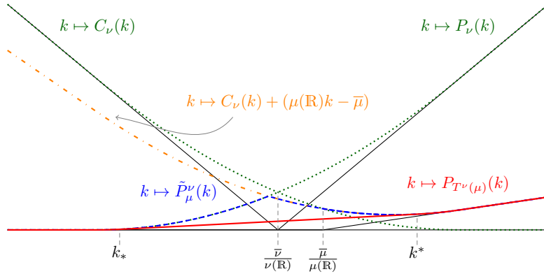
Figure 1: Construction of P_{T^\nu(\mu)} . Dotted curves correspond to the graphs of C_\nu and P_\nu , while the dash-dotted curve corresponds to k \mapsto C_\nu(k) + (\mu(\mathbb{R})k - \bar{\mu}) . The dashed curve represents \tilde{P}_\mu^\nu . Note that \tilde{P}_\mu^\nu is continuous. The solid curve below \tilde{P}_\mu^\nu corresponds to P_{T^\nu(\mu)} , the (modified) potential of the counter-shadow. Note that, on (k_*, k^*) , P_{T^\nu(\mu)} is linear and strictly below \tilde{P}_\mu^\nu , while on \mathbb{R} \setminus (k_*, k^*) it is equal to \tilde{P}_\mu^\nu .
