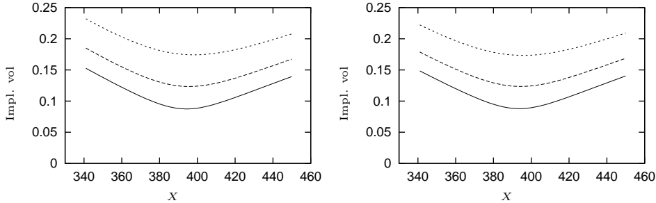
Figure 1: Black-Scholes implied volatilities calculated from options prices generated from the IG (left graph) and MIG (right) models. The three lines correspond to three different values of the parameter G or g , which increases by a factor of 2, as we move up from line to line.
