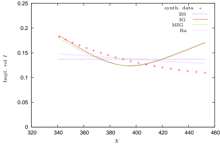
Figure 2: Synthetic implied volatility data, and the corresponding best fit model implied volatilities.
