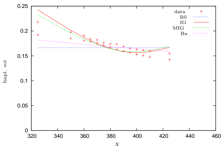
Figure 3: Implied volatilities of puts and calls on 1991/06/03 with maturity 6 months later. Also shown are the best-fit implied volatilities from the best fit Black-Scholes, Bachelier, IG and MIG models.
