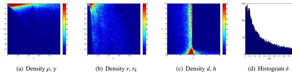
Figure 2: Parameter density distributions for Fold-Hopf bifurcation
