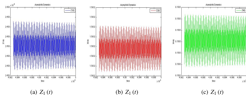
Figure 13: Asymptotic scaled dynamics
