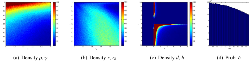
Figure 4: Parameter distributions for co-dimension two repelling frontier regions
