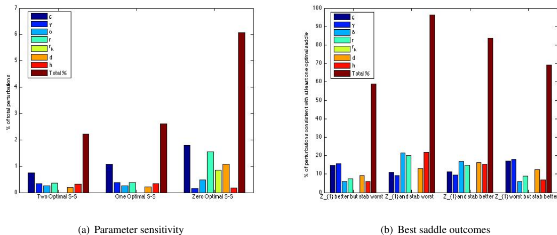
Figure 9: Saddle-saddle scenario sensitivity to parameter perturbations
