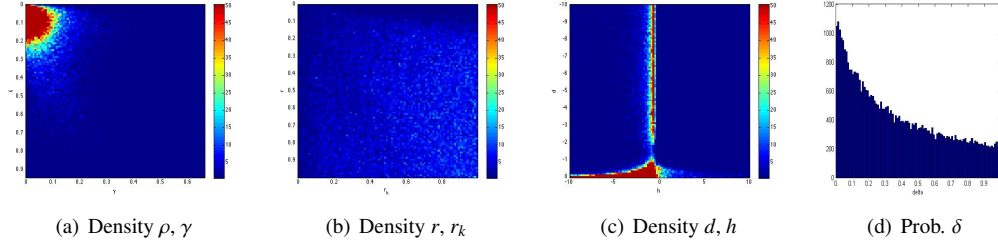
Figure 7: Parameter density distributions for saddle-saddle optimal scenarios
