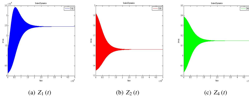
Figure 11: Scaled dynamics during transition
