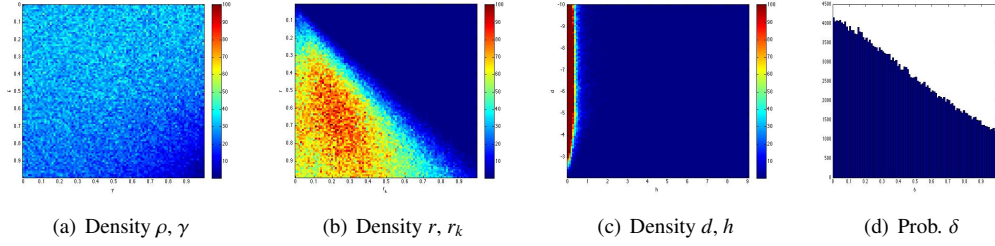
Figure 5: Parameter density distributions for repelling frontier regions
