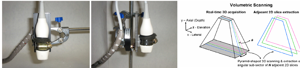
Figure 1: Close up of the motor-arm attached to the 2D phased array probe (left and middle) that accommodates acquisition of adjacent slices by angular displacement of the probe (right).
