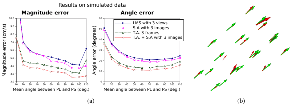
Figure 2: Magnitude and angle errors for different SNR improvement methods(a). Flow vectors reconstructed from simulated data for \alpha_p = 70 (red) and true flow (green) (b)
