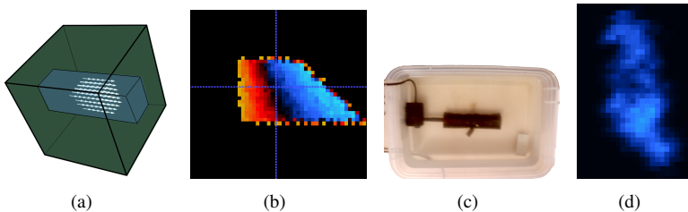
Figure 1: Simulated flow model (a) and resulting Doppler image (b). Flow phantom (c) and acquired Doppler image (d).
