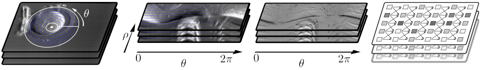
Figure 2: The stack of I_i slices (left) is transformed to J_i slices in polar coordinates around the candidate center c_i , then an energy value E_i (third illustration) is computed for each pixel and a graph is built for each focal plane (right). A single global graph is then obtained by linking a single source and sink node to the left and, respectively, right pixels of each focal plane. The minimum-cost path on such graph simultaneously summarizes contour information, and identifies the depth of the structure.
