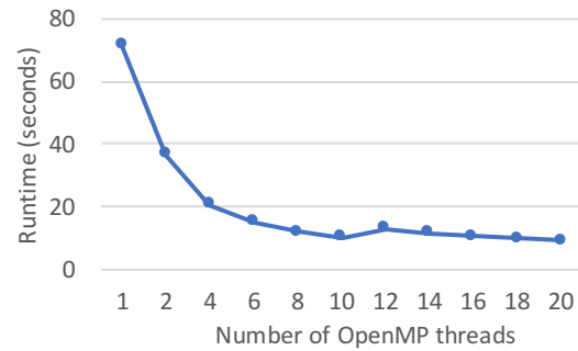
Fig. 10: Performance of CloverLeaf 2D with a 6144^3 mesh with different numbers of OpenMP threads
