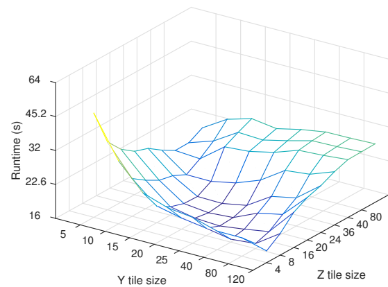
Fig. 5: Performance of OPS on CloverLeaf 3D with a 330^3 mesh over 10 iterations
