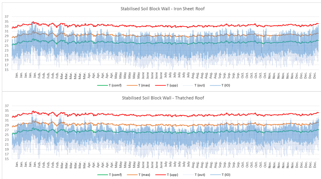
Figure 7: Thermal comfort condition for stabilised soil block walls with iron sheet (top) and thatched roofs (bottom).
