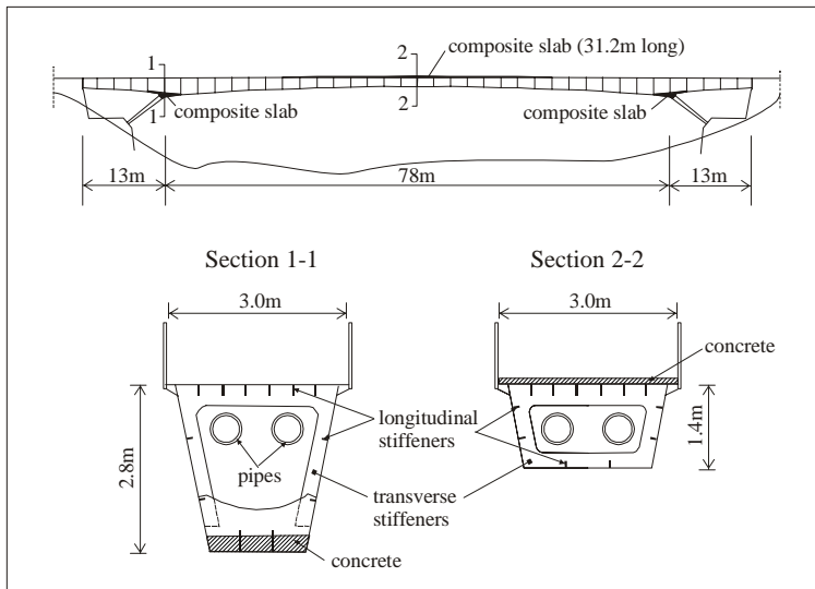
Figure 2: General arrangement drawing (not to scale) of Podgorica footbridge.
