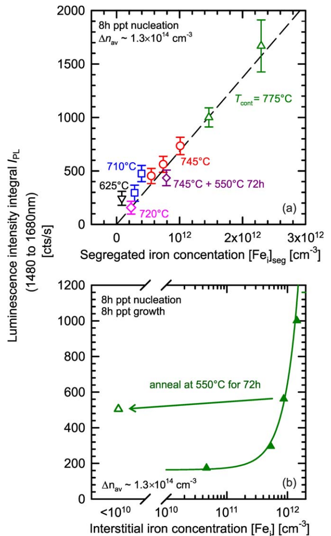
Figure 4. (a) Broadband sub-bandgap luminescence as a function of the iron concentration segregated to oxygen precipitates. (b) Impact of prolonged 550 °C anneal on broadband sub-bandgap luminescence and interstitial iron concentration.
