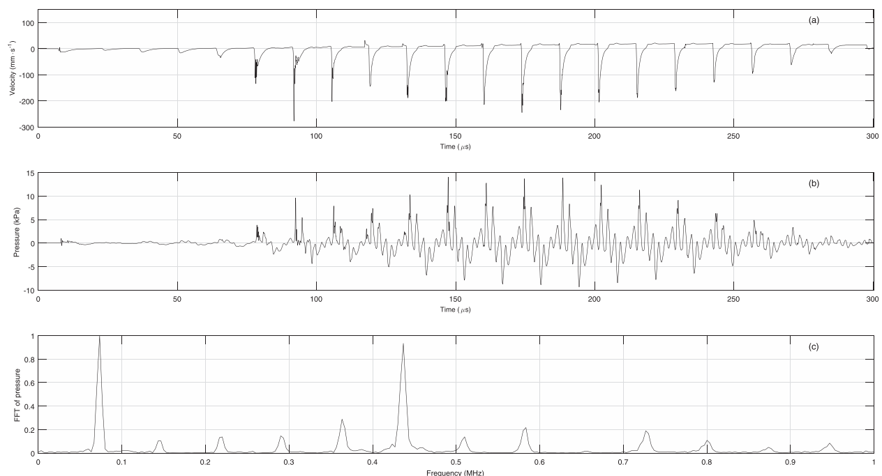
FIG. 8. (a) Axial component of the velocity at the pole of the final sphere of the granular chain, in contact with the cylindrical layer of vitreous carbon. (b) Acoustic pressure predicted with FEA 1 mm from the fluid/structure interface on the axis of symmetry. (c) Normalized FFT of acoustic pressure waveform in (b).
