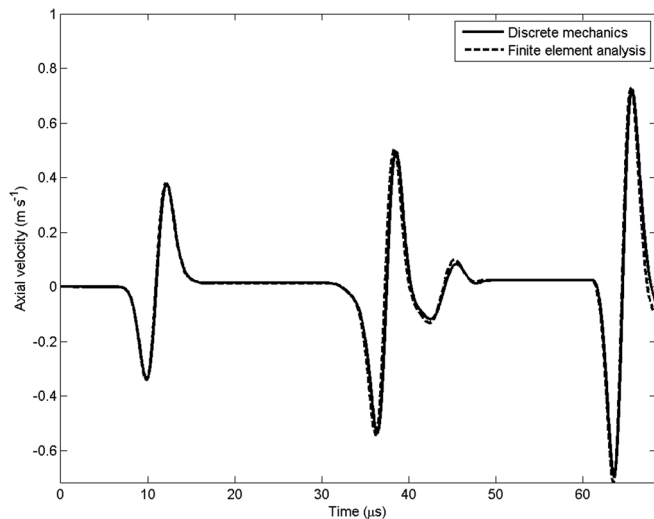
FIG. 5. Axial component of the velocity at the center of the final sphere of the granular chain terminated with a rigid support. Comparison of FEA and discrete mechanics solution.
