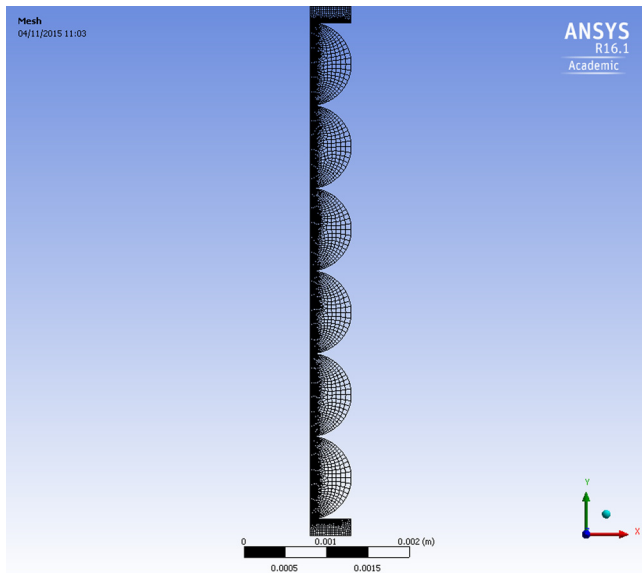
FIG. 3. (Color online) Mesh used for axisymmetric FEA of six-bead granular chain. The top-most sphere is excited by a rigidly vibrating cylindrical piston. The bottom-most sphere is in contact with a rigid support. 3038 contact elements and 7477 solid elements were used.
