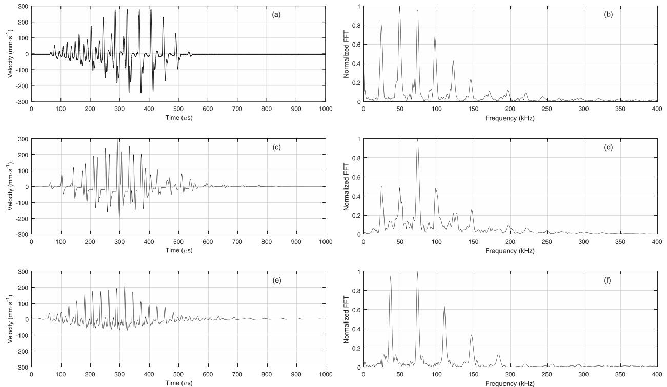
FIG. 6. Axial component of the velocity at the pole of the final sphere of the granular chain (a) measured using a laser vibrometer, (c) predicted with FEA using velocity proportional damping coefficients and with an excitation displacement corresponding to the waveform in (a) scaled by 0.5, and (e) predicted with FEA using a nonlinear damping coefficients based on the formulation by Kuwabara and Kono (Ref. 22) and with an excitation displacement corresponding to the waveform in (a) scaled by 1.5. (b), (d), and (f) correspond to the normalized FFTs of the waveforms in (a), (c), and (e), respectively.
