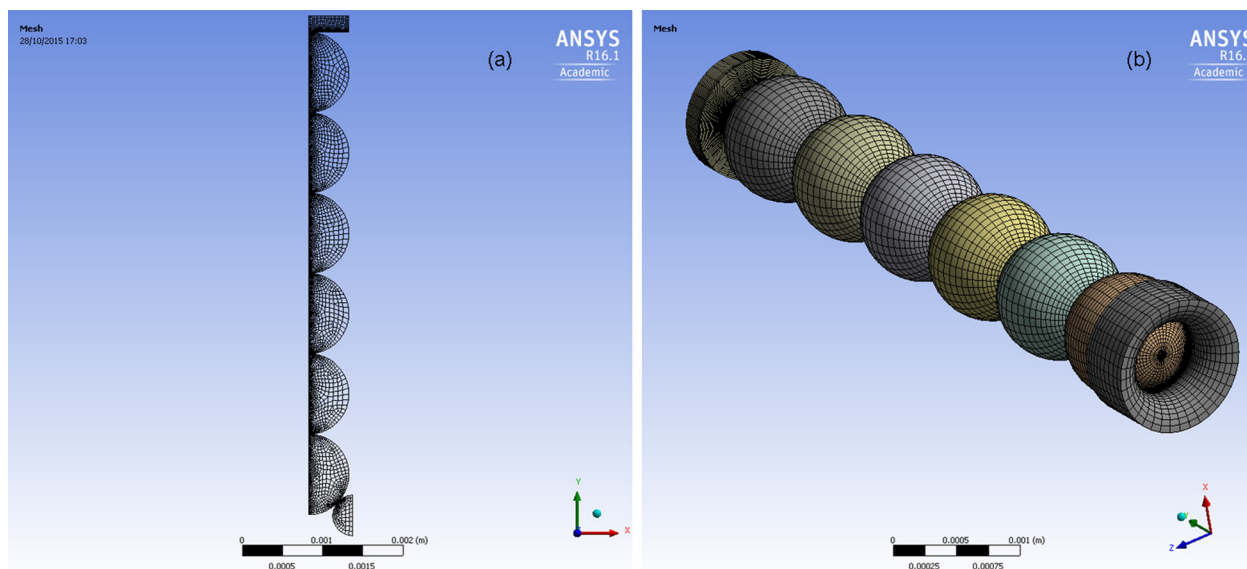
FIG. 4. (a) (Color online) Mesh used for axisymmetric FEA of six-bead granular chain. The top-most sphere is excited by a rigidly vibrating cylindrical piston. The bottom-most sphere is in contact with an annular liquid photopolymer resin support, clamped at its outer diameter. 2267 contact elements; and 5397 solid elements were used. (b) Three-dimensional visualization of mesh used for axisymmetric FEA of six-bead granular chain, cylindrical piston and annular support.
