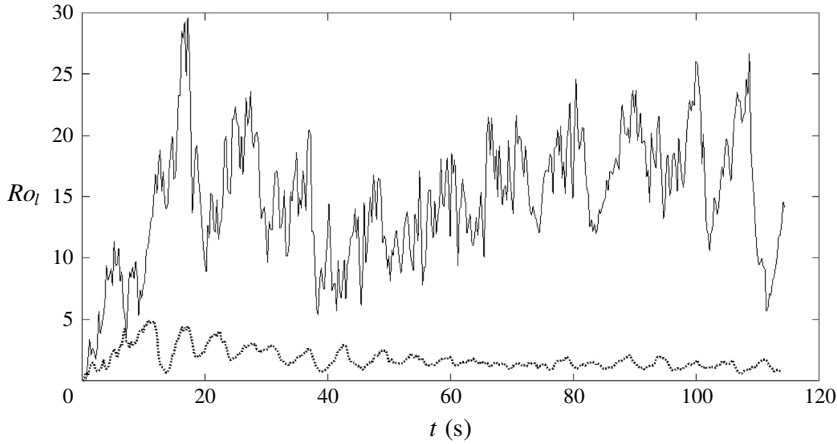
FIGURE 22. Variation of Ro_l with time, near the source at z/d = 0.5 , for a jet with Re_0 = 16\,000 : \cdots\cdots , Ro_0 = 653 , \Omega = 0.42 \text{ rad s}^{-1} ; —, Ro_0 = 1055 , \Omega = 0.73 \text{ rad s}^{-1} .
