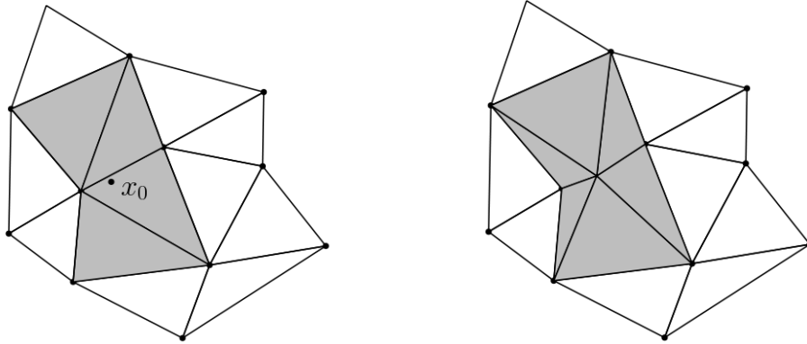
(a) T_{x_0, \omega}^- = \text{Del}_3(\omega) \setminus \text{Del}_3(\omega \cup x_0) (b) T_{x_0, \omega}^+ = \text{Del}_3(\omega \cup x_0) \setminus \text{Del}_3(\omega)
