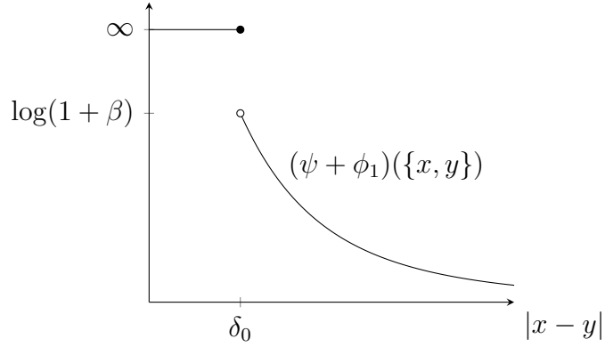
Figure 2.3: A graph of \psi + \phi_1 .
