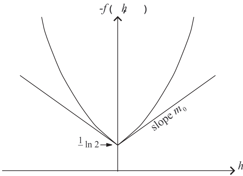
Figure 7: \nu > 1
