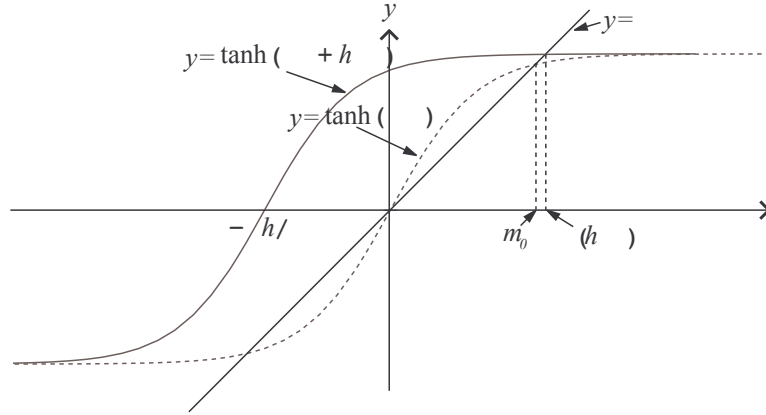
Figure 5: h > 0, \nu > 1
