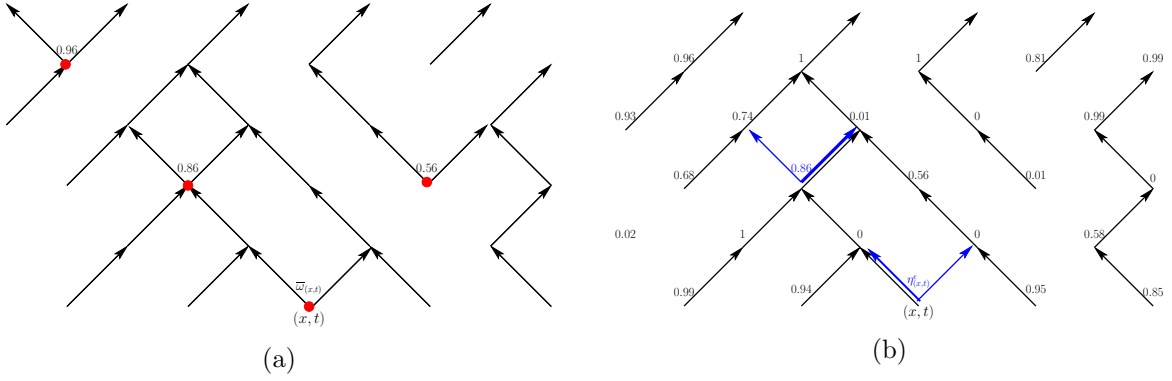
Figure 13: Representation of the random environment (\omega_z^\varepsilon)_{z \in \mathbb{Z}_{\text{even}}^2} in terms of: (a) a marked discrete net (N^\varepsilon, \bar{\omega}^\varepsilon) ; (b) a marked discrete web (W^\varepsilon, \eta^\varepsilon) .
