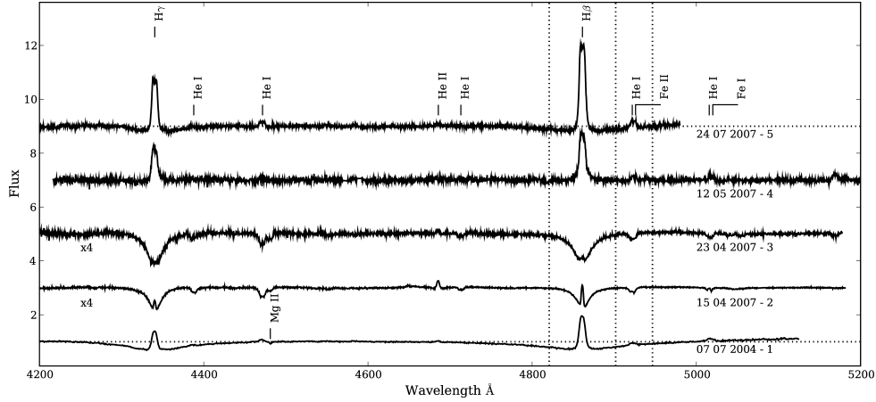
Figure 2. Comparison of average representative normalized spectra of GW Lib sampling the spectral evolution before and during the 2007 super-outburst. The April 2007 spectra have been multiplied by a factor of 4 to magnify the spectral features and allow for a better comparison. The vertical dotted lines annotate the \pm 2500 \text{ km s}^{-1} window for the Balmer lines and the \pm 1500 \text{ km s}^{-1} band for helium lines while the horizontal dotted lines the normalized continuum flux.
