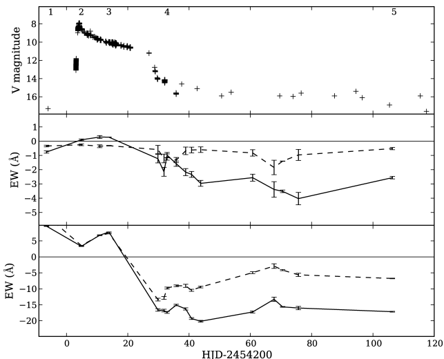
Figure 1. Time evolution of the EW of the principal spectral lines. The 2004 July quiescent epoch is plotted at an arbitrary negative HJD for comparison. In the bottom frame: solid line for H\beta and dashed line for H\gamma . In the middle panel: solid line for He\ I\ 4921\ \text{\AA} represents the general evolution of the He\ I lines and dashed line for He\ II\ 4685\ \text{\AA} . The top panel shows the V magnitude of the outburst, as provided by the AASVO where the numbers indicate position of the spectra from Fig. 2 which are discussed epochs in Section 3.1.
