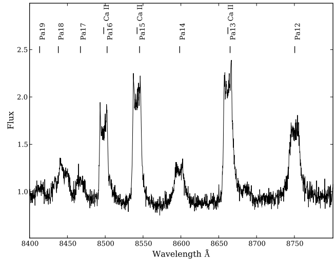
Figure 5. The average normalized I -band spectrum of GW Lib on 2007 July 24 showing the Paschen series and the double-peaked Ca\ II lines.
