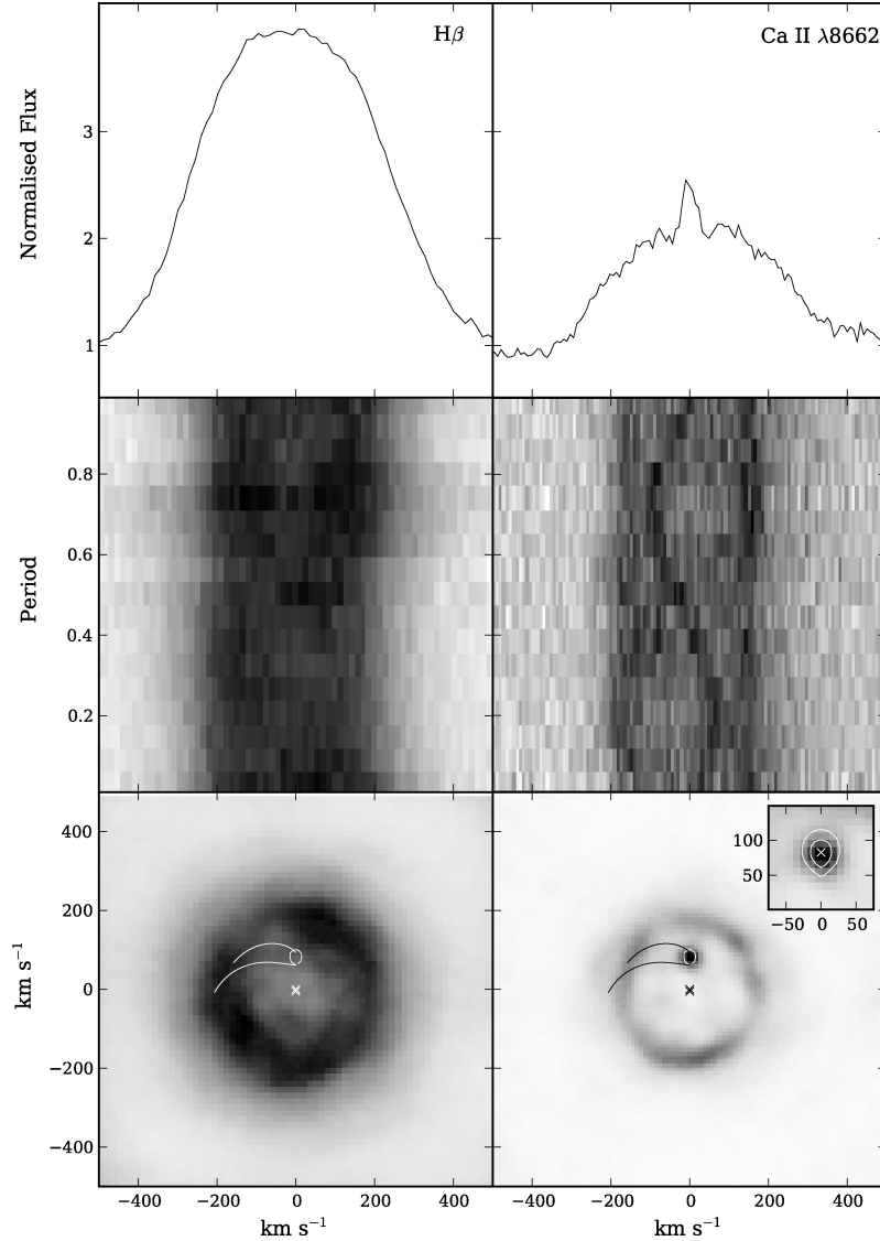
Figure 6. Comparison of the dynamics of the Balmer lines ( H\beta ; left-hand column) versus \text{Ca II} (8662 Å; right column). The top row show average profiles in the reference frame of the donor star S-wave. The sharp donor component stands out in \text{Ca II} but the H\beta profile is smooth. The middle row shows the phase-binned trailed spectrograms. The S-wave can be traced in between the disc peaks in \text{Ca II} only. The bottom row plots the Doppler tomograms showing the superior sensitivity and sharpness in the \text{Ca II} lines. The S-wave is mapped to a sharp spot consistent with donor star emission. Overlaying the Doppler tomograms are the positions of the WD, the Roche Lobe of the donor star and the streams for a model with q = 0.062 . The inset in the \text{Ca II} Doppler map shows the Roche Lobe on the Donor star in more detail for both a q = 0.062 and 0.23 solutions.
