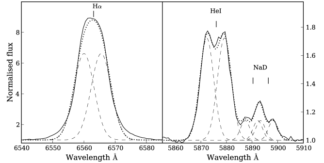
Figure 3. Normalized emission-line profiles of H \alpha (left) and the He I – sodium doublet (right). The solid line represents in both cases the average profile over one orbital period. The dashed lines are the various Gaussian profiles fits and the dotted line is the sum of all single Gaussians. As is clear from these fits, the sodium doublet has, most likely, a very similar origin as the H \alpha and the He I lines.
