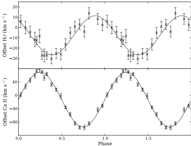
Figure 7. Top panel shows the radial velocity curve of the H\beta emission. The bottom panel shows rotational velocity curve from the \text{Ca II} 8662 Å S-wave emission component. Both are from the phase-binned 2007 June 24 data, showing two orbital cycles.
