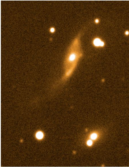
INT 2009-12-10
