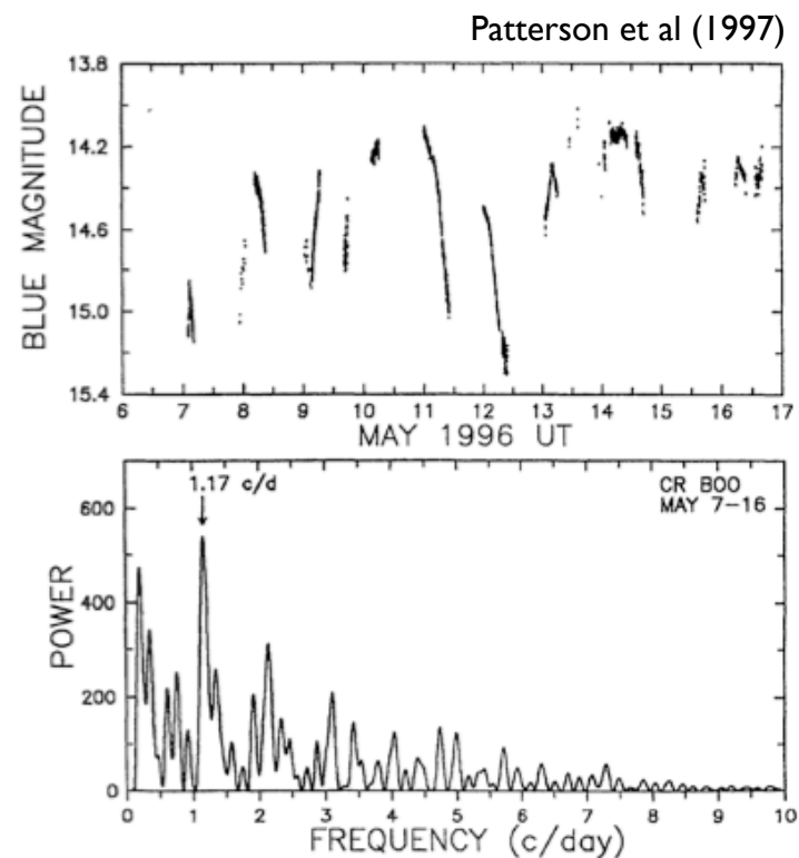
FIG. 3—Upper frame: expanded view of the first 10 d of the 1996 campaign, showing rapid cycling with P \leq 1 d. Lower frame: power spectrum of this light curve, showing a signal at 1.17 \pm 0.04 c/d.
