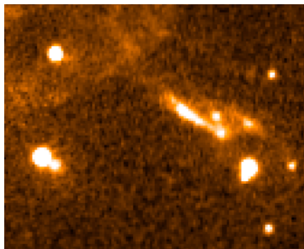
Outburst State
