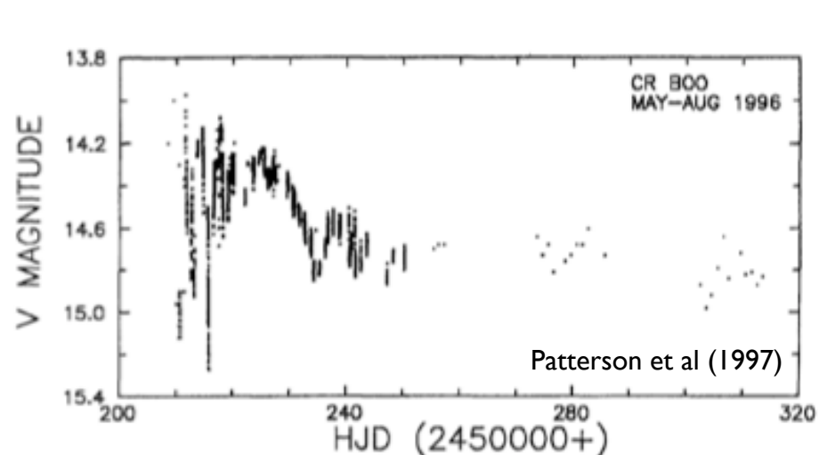
FIG. 2—Light curve of CR Boo in 1996. The star cycled between magnitude 15 and 14 for the first 10 d, followed by a “high state” lasting > 80 d (assuming no downward excursions in light during gaps in the observational record).
