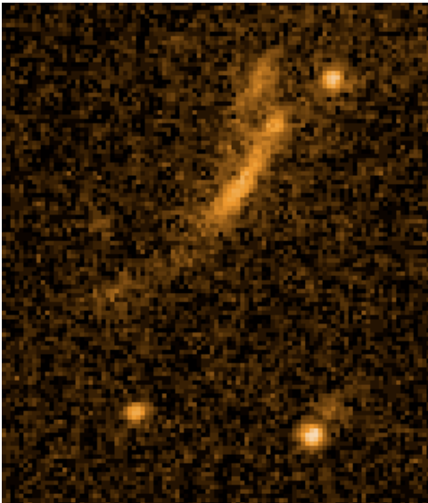
Swift UV 2009-11-26
