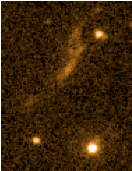
Swift UV 2009-12-10
