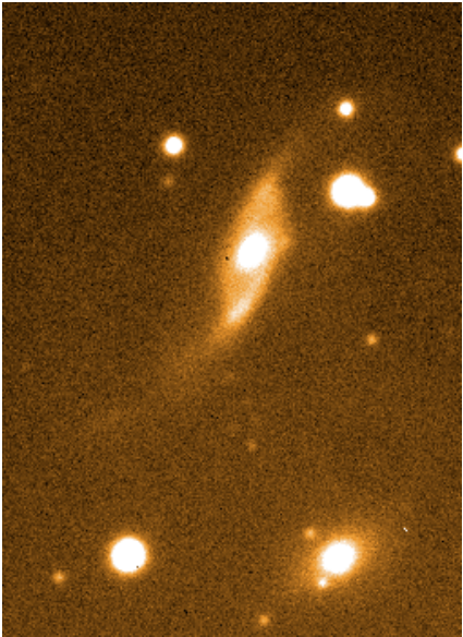
NOT 2009-11-25
