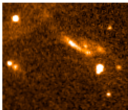
Low State
