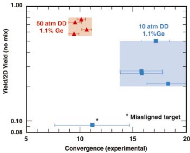
FIG. 7-24. (Color) Measured neutron yield normalized to yield calculated in 2D without mix and including intrinsic hohlraum asymmetry with perfect power balance and pointing accuracy vs experimental convergence for doped, low- (red) and high- (blue) convergence targets.
