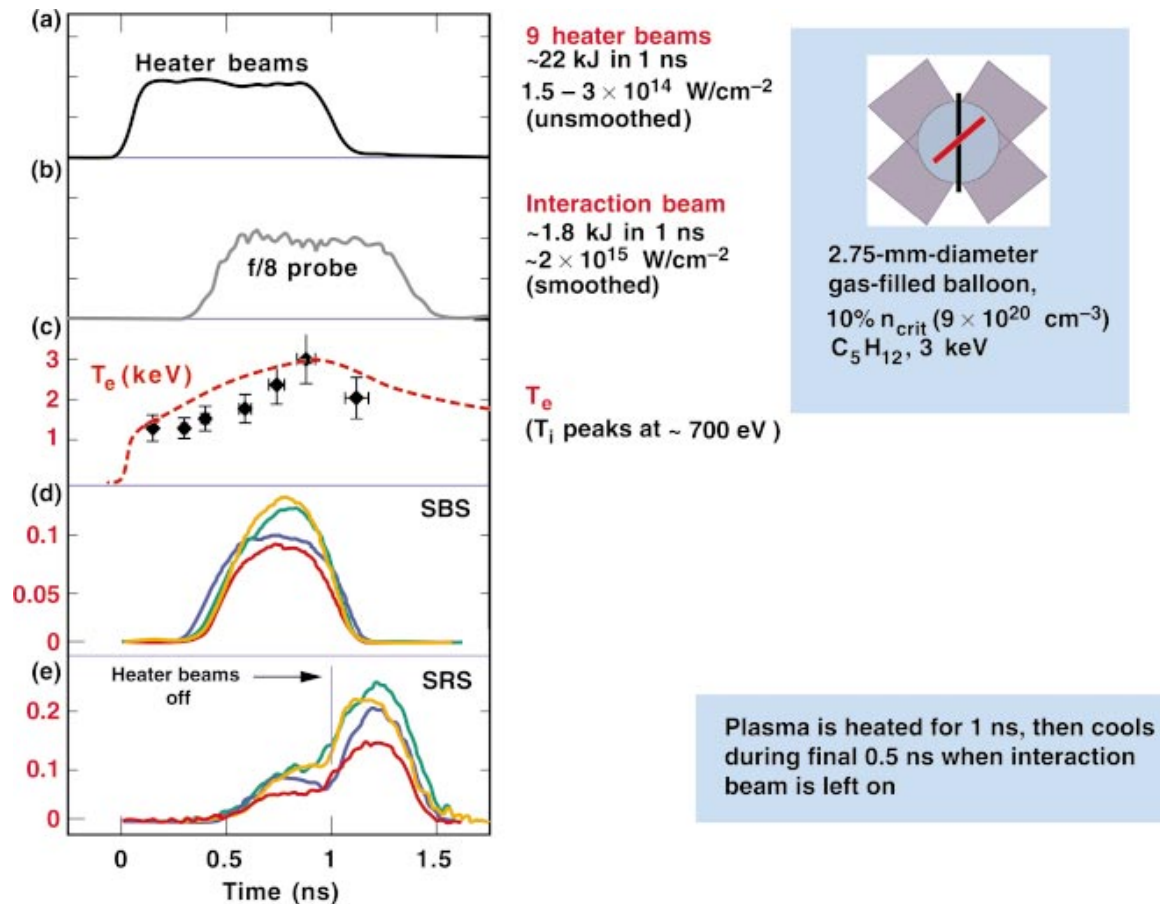
FIG. 3-16. (Color) Gasbag plasmas were developed to approximate the NIF inner beam plasma conditions. Shown are (a) the typical pulse shape of the heater beam power, (b) the f/8 probe incident power, (c) the computed and Thomson scattering measurement of the electron temperature, (d) the fractional SBS reflected power, and (e) the fractional SRS reflected power. The multiple curves in (d) and (e) are the scattering levels from different shots and indicate typical shot-to-shot scatter [S. H. Glenzer et al. , Phys. Rev. E 55 , 927 (1997)].
