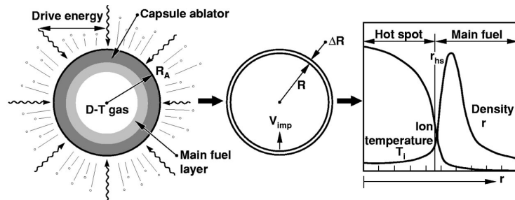
FIG. 1-6. Physics specifications on current ICF ignition targets include constraints on drive intensity, symmetry, stability, and ignition.
