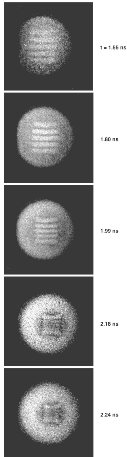
FIG. 6-20. Radiographs of a capsule with \lambda_0 = 70 \mu\text{m} perturbations, at t = 1.55, 1.80, 1.99, 2.18, and 2.24 ns.
