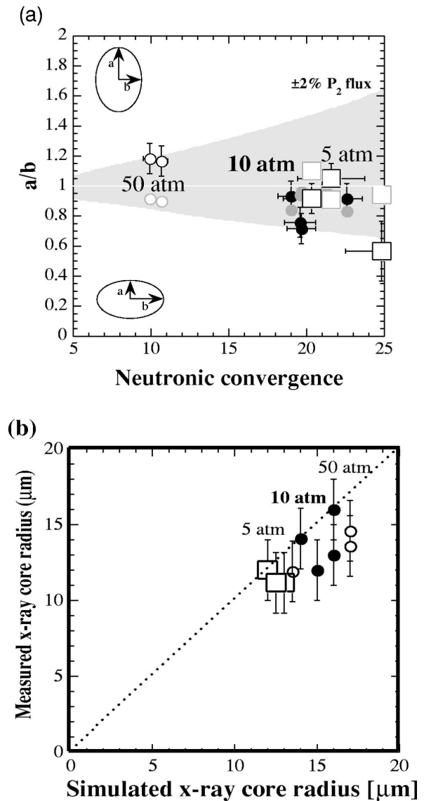
FIG. 7-34. (a) Measured and simulated “ a/b ” distortion of 50% x-ray self-emission contour vs inferred fuel convergence for 5 atm D 2 -filled capsules (open squares), 10 atm D 2 -filled capsules (filled circles), and 50 atm D 2 -filled capsules (open circles); simulation points are indicated in gray; (b) measured vs simulated average radius of 50% x-ray self-emission contour.
