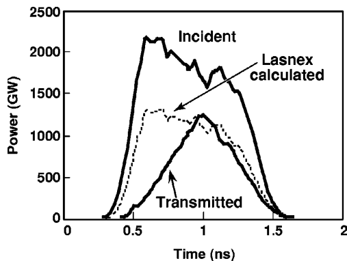
FIG. 3-23. The incident laser power, measured transmitted power (solid) and the calculated transmitted power (dashed) are shown for high laser intensity ( I=2 \times 10^{15} W/cm ^2 ) [J. D. Moody et al. , Phys. Plasmas 7, 3388 (2000)].
