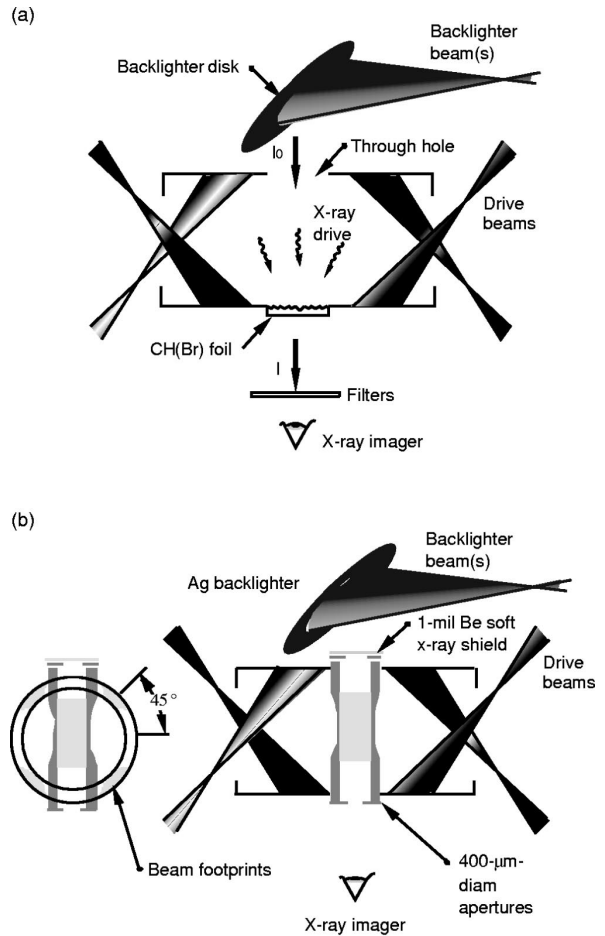
FIG. 6-5. (a) Modulated planar CH(Br) foils or modulated CH(Ge) capsules were mounted on the hohlraum wall. (b) The cylindrically convergent experiment was mounted perpendicular to the hohlraum axis.
