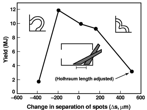
FIG. 2-18. Integrated calculations are being used to confirm acceptable sensitivity to pointing. Laser ring separation controls P_4 . The pointing sensitivity is large enough that we can use it to control P_4 , but small enough for the specified pointing accuracy.
