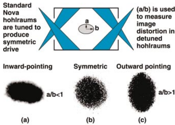
FIG. 5-15. (Color) Nova experiments have extensively used x-ray imaging of imploding capsules to test the modeling of hohlraum drive asymmetries. Observed x-ray image shapes confirm the calculated variation of the implosion shape with beam pointing: (a) inward-pointing shifts produce waist-high fluxes or “sausaged” images; (b) symmetric; (c) outward-pointing shifts produce pole-high fluxes or “pancake” images. The tilted axis in (a) shows the effects of beam imbalance and pointing errors prior to the Precision Nova improvements.
