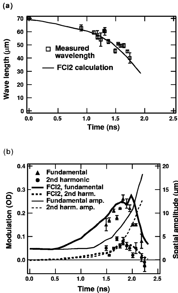
FIG. 6-21. (a) Wavelength determined from the images in Fig. 6-18 as a function of time. (b) Modulation amplitude of the fundamental and first harmonic for the radiographs and simulated radiographs, and simulated modulation at the ablation front.
