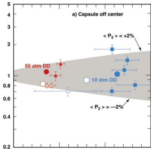
FIG. 7-22. (Color) The 50% gated-x-ray image distortions ( a/b ) vs neutronically inferred convergence for doped (solid) and undoped (open), low- (red) and high- (blue) convergence targets. Simulations are represented by circles. Gray shading indicates time- averaged P_2 asymmetry of < 2\% .
