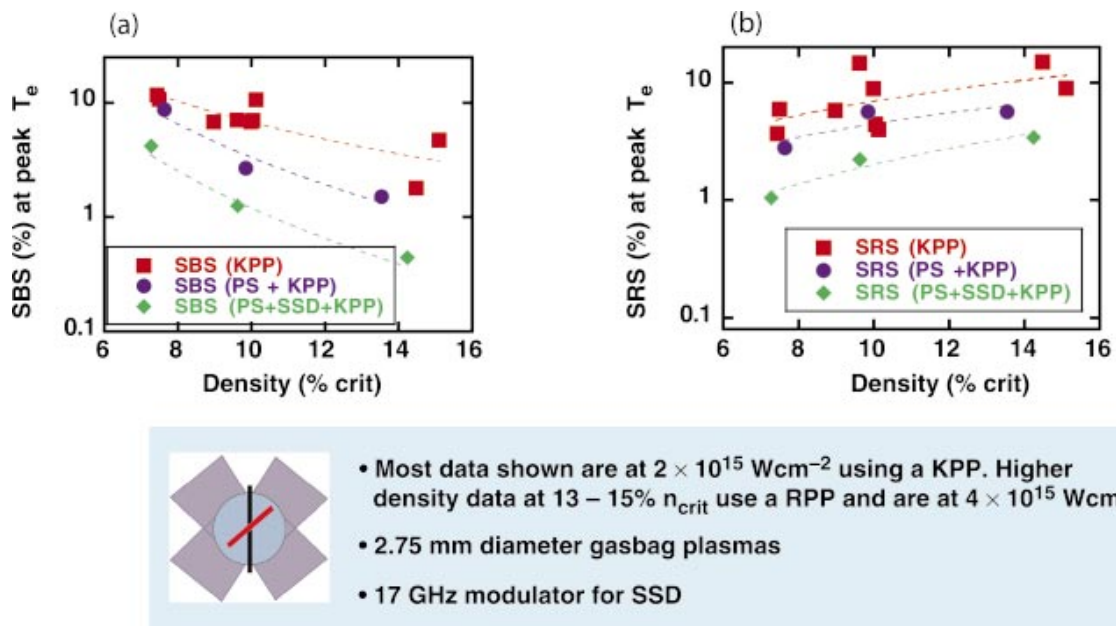
FIG. 3-20. (Color) Gasbag experiments using a KPP and 17 GHz SSD for beam smoothing show that SBS (a) and SRS (b) from gasbags filled with mixtures of \text{C}_5\text{H}_{12} and \text{C}_3\text{H}_8 are consistent with experiments using an RPP and 3 GHz SSD (see Fig. 3-19).
