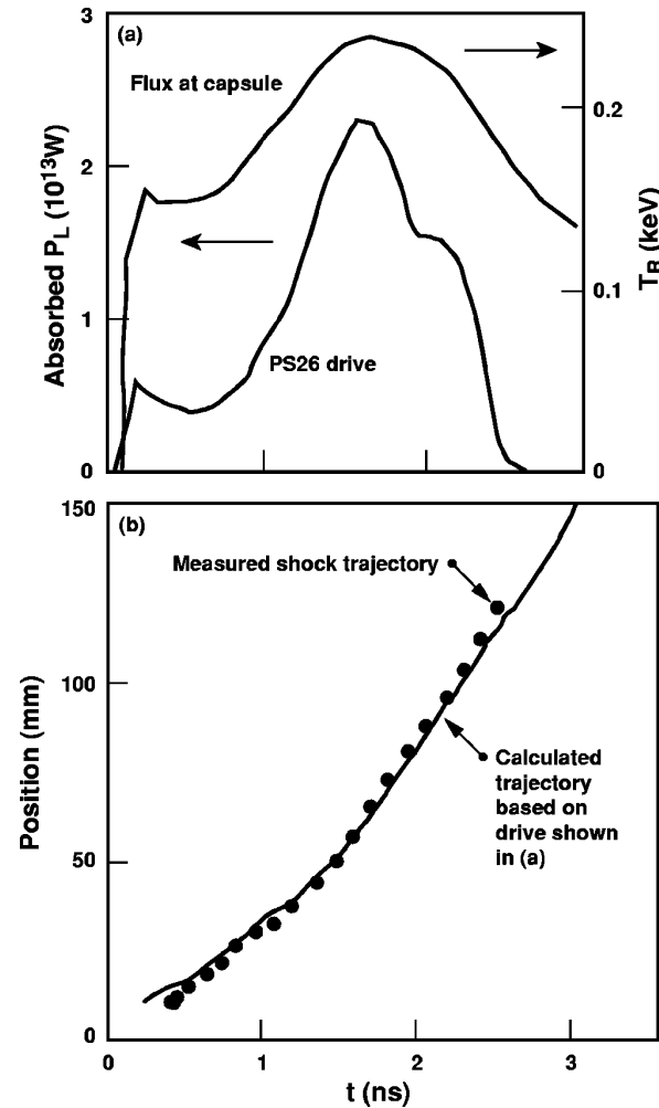
FIG. 7-11. (a) Measured absorbed laser power and measured soft x-ray flux (plotted as a blackbody flux temperature) for the Nova HEP4 experiments from absolutely calibrated filtered diode array (Dante). (b) Measured shock trajectory in Al wedge and corresponding predicted trajectory based on the x-ray drive in (a).
