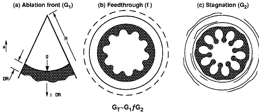
FIG. 6-1. Schematic showing how RT perturbation growth affects an implosion. The designations G_T , G_1 , f , and G_2 correspond to the total growth factor, growth factor at the outer surface during acceleration, feedthrough to the inner surface, and growth factor at the inner surface during deceleration.
