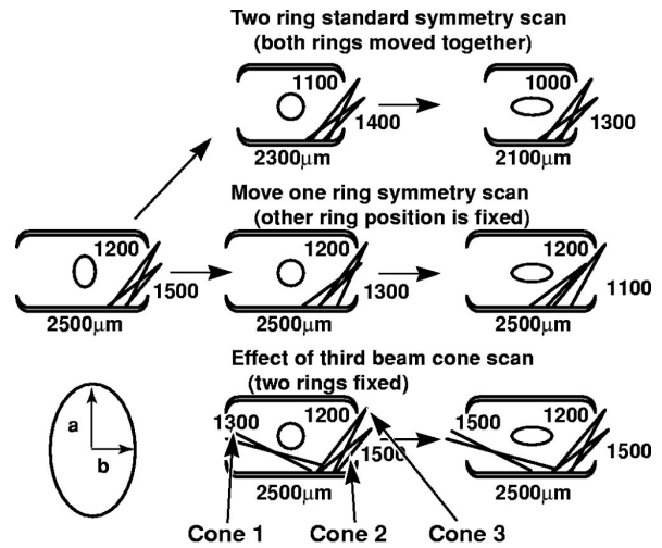
FIG. 5-25. Forty of Omega's 60 beams can be arranged in three rings per side with five, five, and 10 beams per ring at incidence angles of 21.4°, 42°, and 59°, respectively. Schematic shows the three types of symmetry scans tried and the expected effect on the imploded core.
