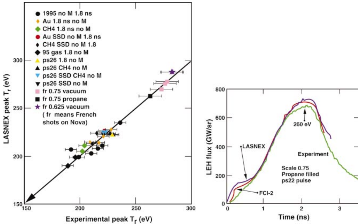
FIG. 4-17. (Color) Drive in a wide variety of ignition-relevant hohlraums agrees with detailed modeling for drive measured through the LEH.
