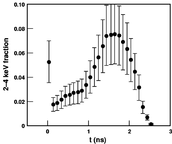
FIG. 7-12. Estimated 2–4 keV flux on the Nova HEP4 capsule as a fraction of total x-ray power. Error bars represent only the uncertainty in Dante calibration and spectral unfold; additional uncertainty in the angular distribution could result in another factor-of-2 uncertainty. Capsule preheat largely arises from photons in this region of the x-ray spectrum which come from Au M-lines.
