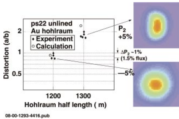
FIG. 5-16. (Color) Precision Nova implosions have shown excellent reproducibility of symmetry.
