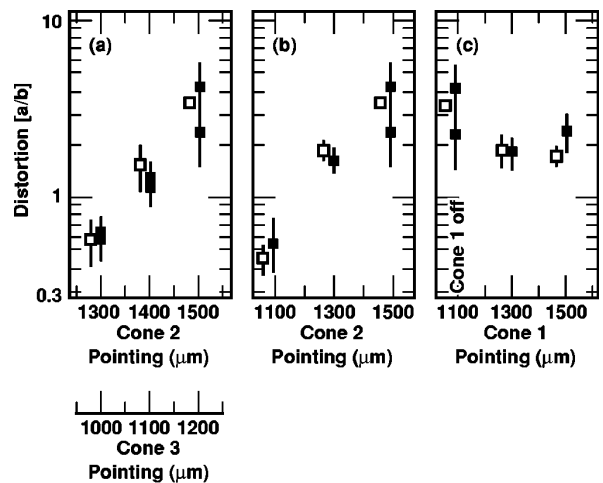
FIG. 5-26. Distortion as a function of beam pointing for the experiment (a) in which beam cones 2 and 3 formed a single ring on each side of the hohlraum, (b) in which the pointing of cone 2 was varied while that of cone 3 remained fixed at 1200 \mu\text{m} , and (c) in which cone 1 was added while cones 2 and 3 remained fixed at 1500 and 1200 \mu\text{m} , respectively. The uncertainty in the data (solid symbols) is determined by analyzing multiple images and contours on the same experiment, and that from simulations (open symbols, offset to the left for clarity) represents the range of calculations obtained from the LLNL and LANL versions of LASNEX.
