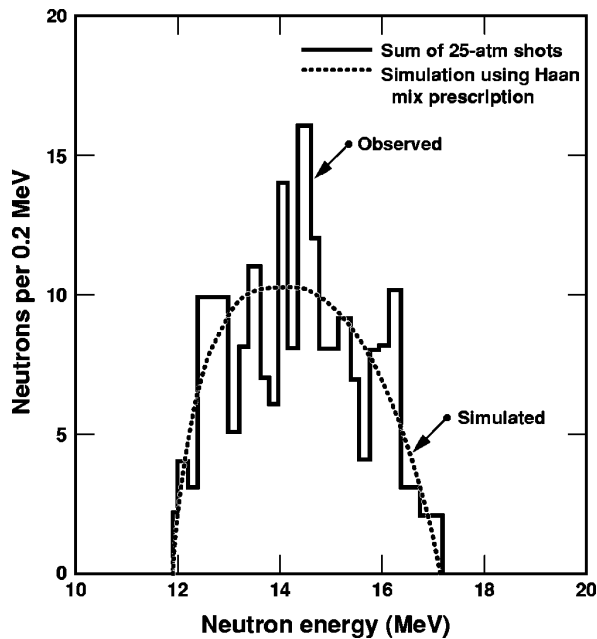
FIG. 7-3. Secondary-neutron energy spectrum measured with array of neutron time-of-flight detectors (LaNSA). Observed is sum of spectra from all 25 atm HEP1 capsules. The shape of the neutron spectrum is well-matched with the Haan mix model.
