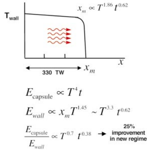
FIG. 2-23. (Color) At longer pulses, NIF is capable of delivering more laser energy and the longer pulses result in improved capsule coupling efficiency because of higher hohlraum wall albedo.
