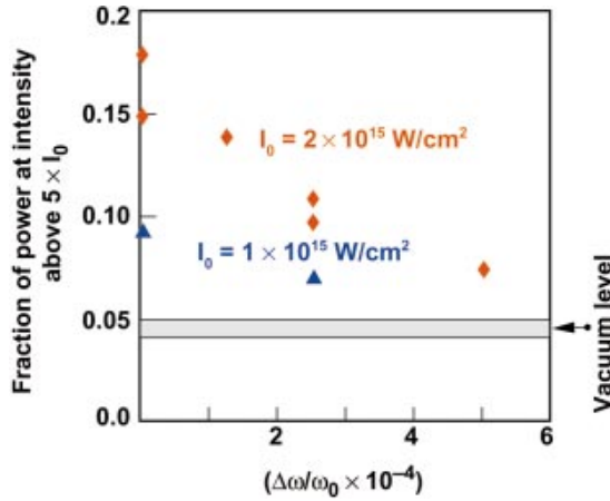
FIG. 3-7. (Color) The reduction of self-focusing by SSD smoothing is shown as a function of the laser bandwidth as a percentage of the laser frequency. The reduction is characterized by plotting the fraction of the laser power above five times the mean intensity ( 0.04 in vacuum) after self-focusing in the plasma for the mean intensities, I_0 , as indicated. Simulation parameters: T_e = 3 keV, n_e = 0.1n_c , I_0 = 2 \times 10^{15} W/cm ^2 , \lambda_0 = 351 nm in a C _5 H _{12} plasma.
