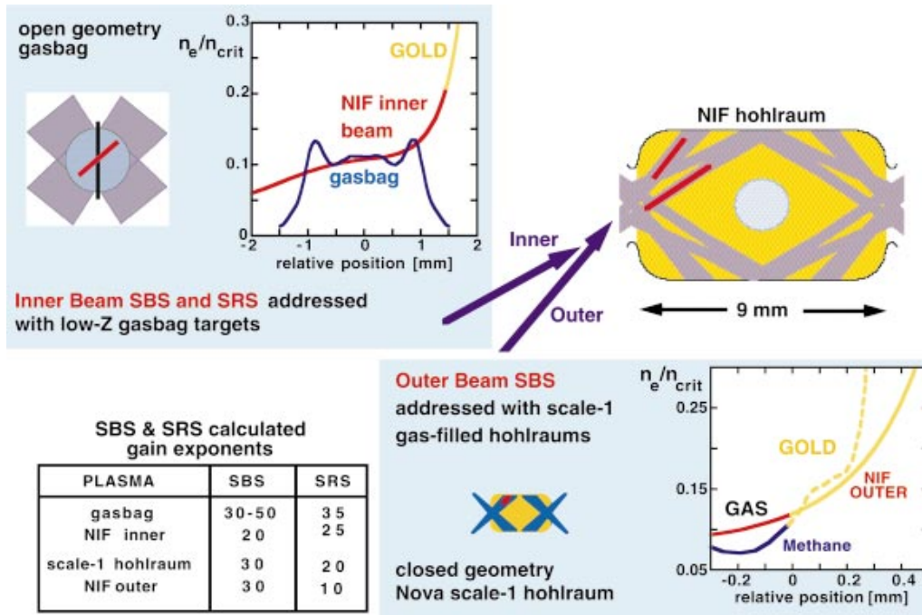
FIG. 3-10. (Color) Nova gasbags and scale-1 hohlraums develop plasma conditions and linear LPI gains (calculated by the postprocessor LIP with LASNEX plasma conditions) similar to NIF plasma conditions for the most unstable regions of the inner beams and outer beams, respectively. The interface between the low-Z fill and the gold blowoff is indicated by change in color to yellow from blue or red. The red bars along the beam paths on the NIF hohlraum schematic show what part of the NIF laser plasma interaction is simulated either by the gasbag or by the scale-1 hohlraum.
