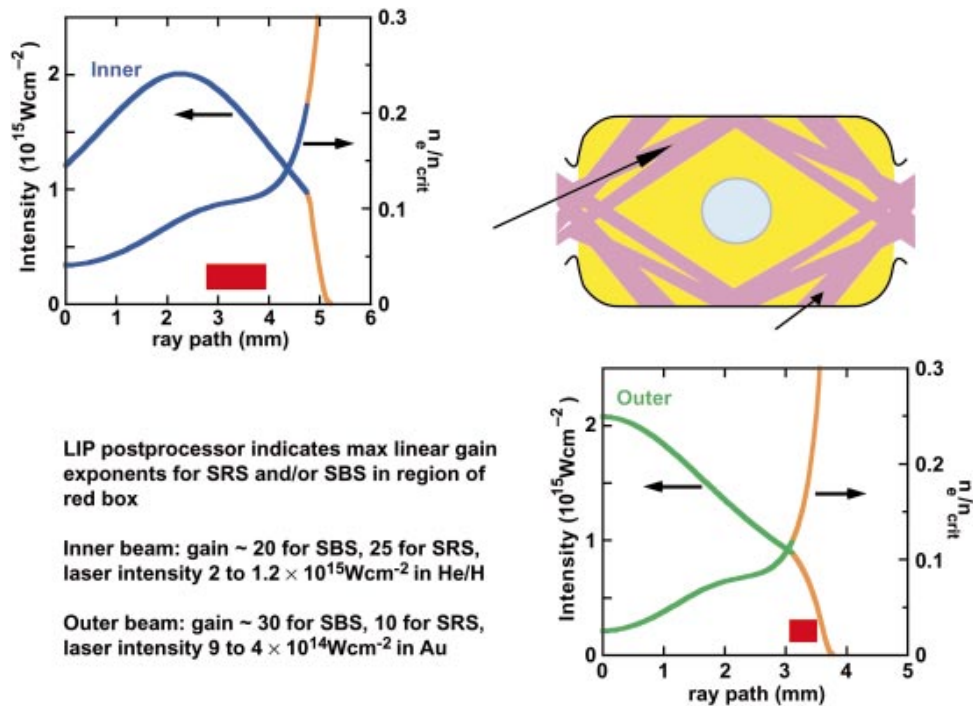
FIG. 3-2. (Color) A schematic of a NIF hohlraum with a capsule and an inner (blue) and an outer (green) ring of beams are shown. Also shown are the electron density and laser intensity along the path of the outer and inner beams. The f/8 inner and outer NIF beam quads interact with NIF plasmas at average irradiances of < 2 \times 10^{15} \text{Wcm}^{-2} . The linear gain for stimulated Raman scattering is maximum in the low-Z interior for the NIF inner beams while gain for the outer beams is maximum for stimulated Brillouin scattering in the high-Z hohlraum blowoff. The interface between the low-Z fill and the gold blowoff is indicated by change in line color to yellow from blue or green.
