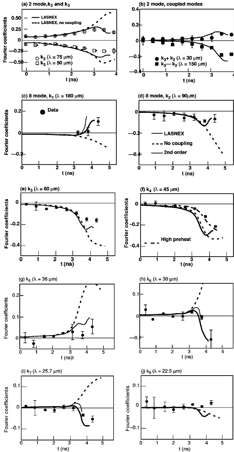
FIG. 6-12. The time dependence for the two- and eight-mode data. (a) The open circles represent k_2 (the \lambda = 75 \mu\text{m} component of the pre-existing perturbation), and the open squares correspond to k_3 (the \lambda = 50 \mu\text{m} component of the perturbation) for the 2-mode foil. (b) The solid circles correspond to the k_3+k_2 , \lambda = 30 \mu\text{m} coupled term, and the solid squares to the k_3-k_2 , \lambda = 150 \mu\text{m} coupled term. The smooth solid curves are the results of 2D LASNEX simulations for this two-mode foil, and the dashed curves correspond to assuming that only one of the two initial perturbations was present at a time. In (c)–(j), the growth of modes \lambda_n = (180 \mu\text{m})/n is shown vs time, where n = 1 to 8. The thin curves for modes k_1 , k_6 , and k_7 correspond to the results of a weakly nonlinear, second-order perturbation theory. The long dashed curve for mode k_4 corresponds to a simulation with assumed enhanced preheat in the foot of the drive.
