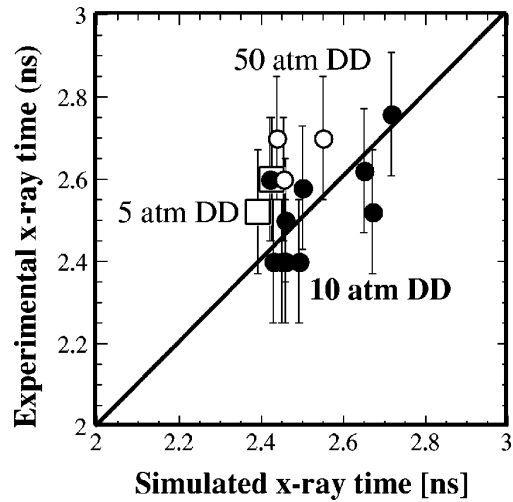
FIG. 7-32. Measured vs simulated instant of peak x-ray self-emission for 5 atm D 2 -filled capsules (open squares), 10 atm D 2 -filled capsules (filled circles), and 50 atm D 2 -filled capsules (open circles).
