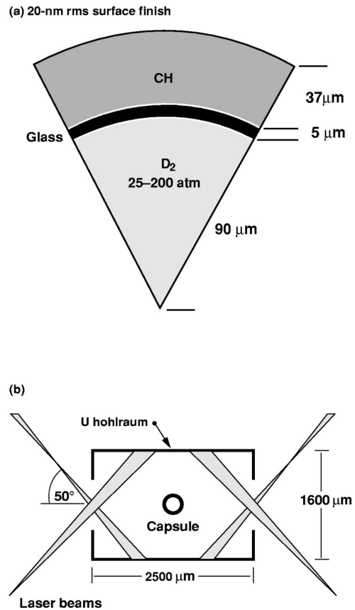
FIG. 7-1. (a) Capsule and (b) hohlraum geometry used for HEP1.
