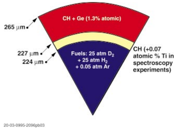
FIG. 7-9. (Color) Cross section of a typical capsule design for the HEP4 campaign. For spectroscopy experiments, the inner CH shell had a Ti dopant. The \text{D}_2 fuel was diluted with \text{H}_2 to limit the yield in order to avoid saturation of the LANSAN neutron detector array.
