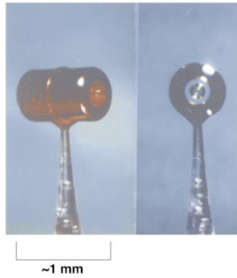
FIG. 1-4. (Color) Nova implosion target illustrating beam geometry. Five Nova beams irradiate each side of the hohlraum. The beams are uniformly distributed around the rim of a 100° cone.
