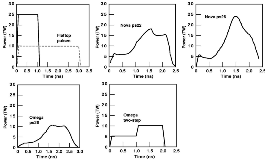
FIG. 4-2. The Nova and Omega hohlraums have been heated by a variety of pulse shapes.
