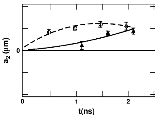
FIG. 5-31. Results from Nova split-ring symmetry experiments. Foam ball second P_2 order Legendre distortions for phased (triangles) and unphased (open circles) drive. Curves are fits to the data.
