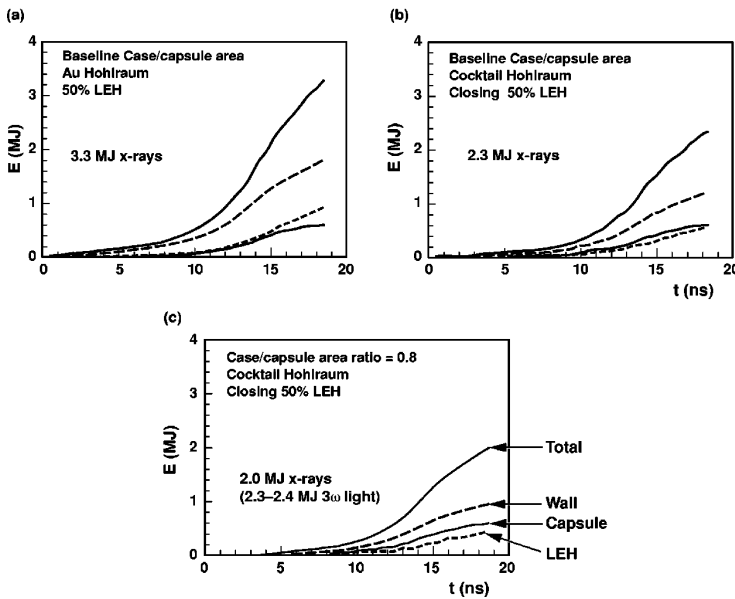
FIG. 2-25. Use of cocktails, LEH reduction, and smaller case-to-capsule area ratio leads to reduced radiation requirements, which might make a 600 kJ absorbed-energy capsule feasible on NIF.
