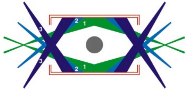
FIG. 7-20. (Color) Shown is the HEP4 hohlraum geometry with multicone irradiation used on the Omega laser. Cone 1 enters hohlraum at 22^\circ , cone 2 at 42^\circ , and cone 3 at 58^\circ .
