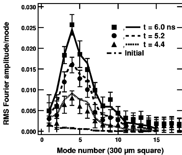
FIG. 6-17. Fourier spectra of \ln(\text{exposure}) vs time for the 3D multimode foil. The curves are from the HYDRA 3D simulations and include the effect of finite instrumental resolution. The symbols are results from analyzing the experimental radiograph.
