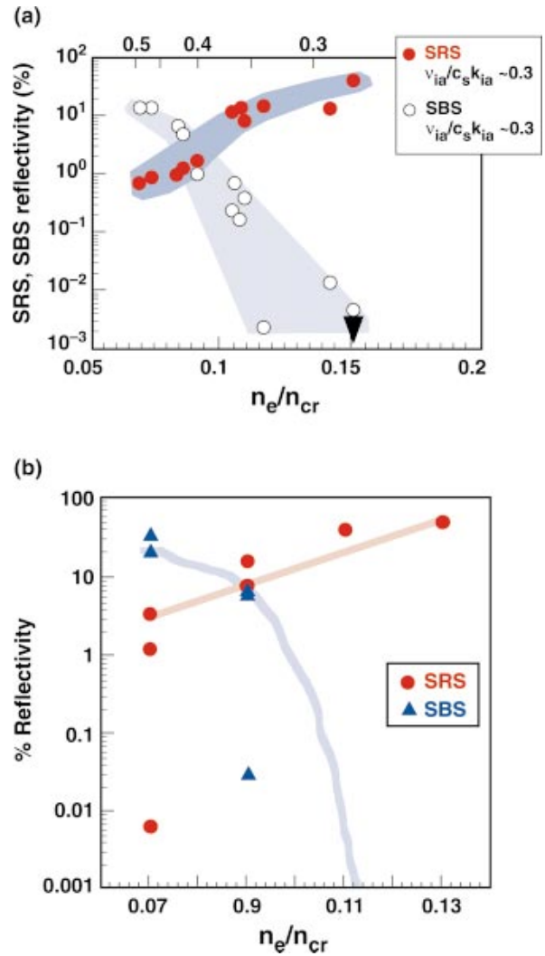
FIG. 3-21. (Color) Data (a) [D. S. Montgomery et al. , Phys. Plasmas 5, 1973 (1998)] and F3D simulations (b) show an anticorrelation of the SRS and SBS reflectivity as a function of electron density. The SBS and SRS reflectivity for a given density was varied in the simulations by changing the ion wave damping which affects the linear SBS gain and the SRS and SBS saturation. For each density, a higher SBS reflectivity is paired with a lower SRS reflectivity.
