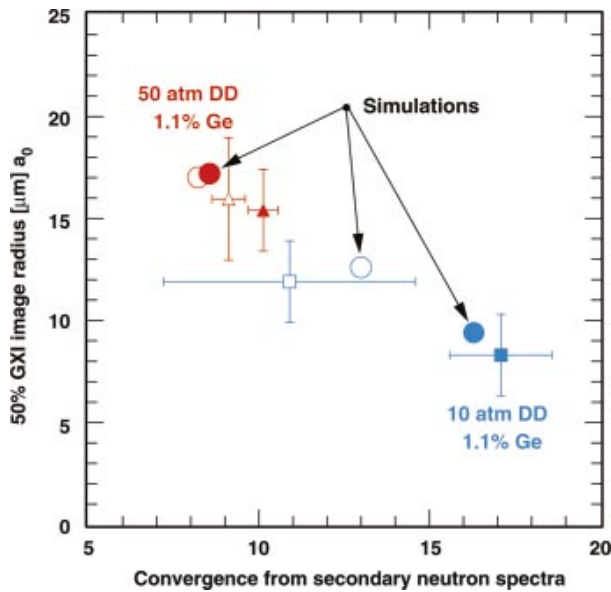
FIG. 7-21. (Color) The 50% gated-x-ray image sizes vs neutronically inferred convergence for doped (solid) and undoped (open), low- (red) and high- (blue) convergence targets. Simulations are represented by circles.
