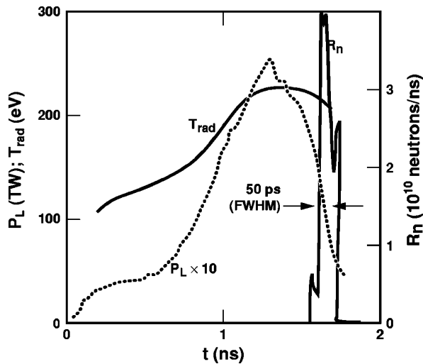
FIG. 7-2. Observed laser power P_L , hohlraum temperature T_r , and neutron production rate R_n for 100 atm DT-filled HEP1 capsules.
