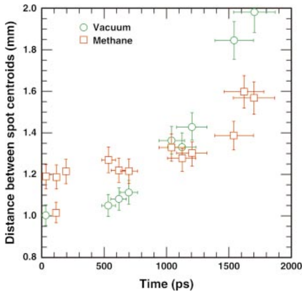
FIG. 5-9. (Color) Because of inward motion of the hohlraum wall, the separation of the two rings of laser spots in the Nova hohlraums increases with time. Circles and squares represent data from vacuum and 1 atm methane-filled Nova hohlraums, respectively.
