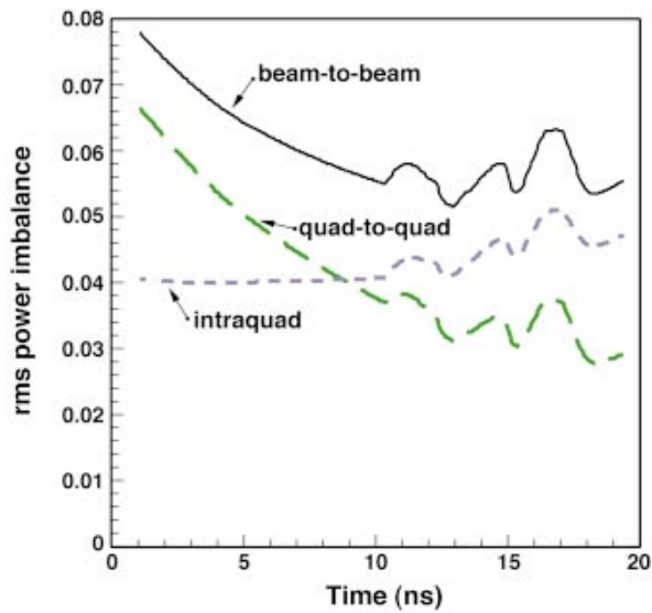
FIG. 2-19. (Color) The calculated total rms power imbalance vs time on NIF for a 1.8 MJ scale of the PT pulse meets the power balance functional requirements specified in Table II-1.
