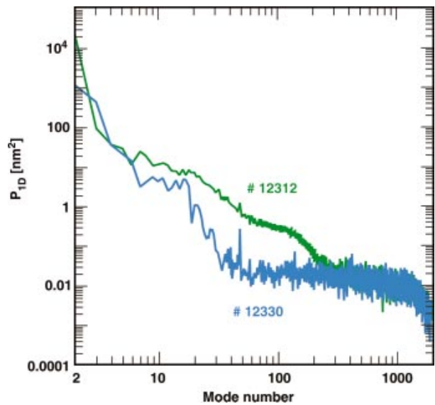
FIG. 7-25. (Color) Measured 1D Fourier power spectrum of surface roughness for two targets: (a) "Rough" is identified with target #12312 (green). (b) "Smooth" with target #12330 (cyan).
