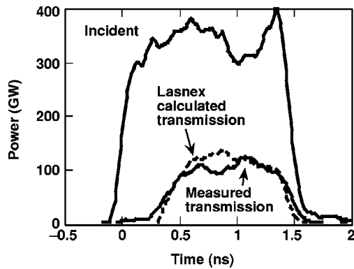
FIG. 3-22. The incident laser power, measured transmitted power (solid), and the calculated transmitted power (dashed) are shown for low laser intensity ( I=10^{14} W/cm ^2 ) [J. D. Moody et al. , Phys. Plasmas 7, 3388 (2000)].
