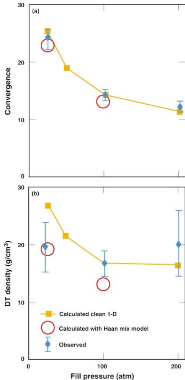
FIG. 7-4. (Color) Observed and calculated (a) convergence and (b) density vs capsule fill pressure for the HEP1 experiments. The experimental measurements and calculations of convergence are in good agreement. Density, expressed as equivalent DT fill even when the capsule has a pure \text{D}_2 fill, is proportional to the cube of the convergence ratio and is highly sensitive to errors in the measurement.
