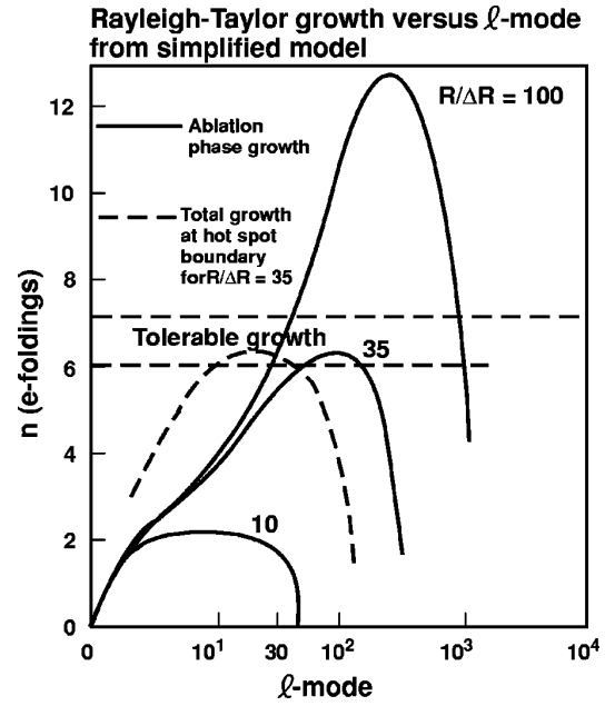
FIG. 6-3. The ratio of capsule radius to shell thickness, the capsule aspect ratio, largely determines hydrodynamic instability growth. Simple analytic models can be used to estimate the amplification of perturbations as a function of mode number.
