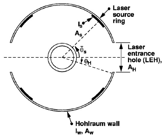
FIG. 5-3. A simplified spherical hohlraum is used to analyze hohlraum symmetry.
