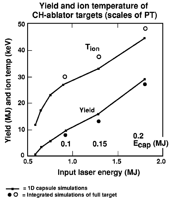
FIG. 2-11. Scales of the PT point design ignite in 1D above about 0.7 MJ. For the 1D capsule simulations, capsule dimensions and times are scaled by s , and the effective laser energy is given by E_{\text{eff}}(\text{MJ}) = 1.35s^3 , where s = 1 is the PT design. For the integrated hohlraum and capsule simulations, dimensions and times are proportional to s , and powers are proportional to s^2 .
