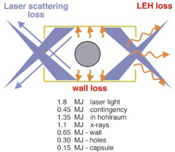
FIG. 2-22. (Color) The NIF “point design” achieves a calculated coupling efficiency to the fuel capsule of 8.3% relative to 1.8 MJ of laser output or 11% relative to a calculated 1.3 MJ of absorbed energy. Recent advances in target physics project coupling efficiencies of 20% to 30%. These calculations rely on material mixtures to reduce hohlraum-wall losses and improved understanding of hohlraum symmetry to reduce case-to-capsule area ratios and LEH areas.
