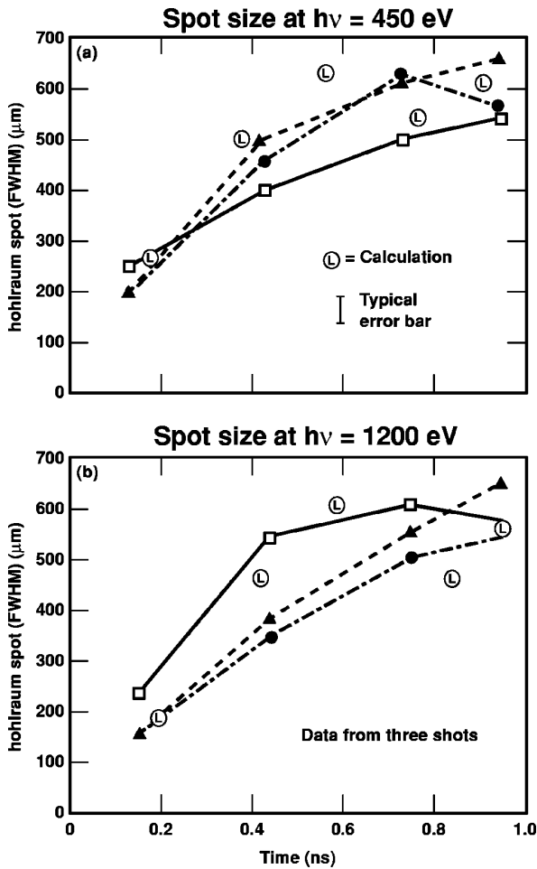
FIG. 4-10. Data and postprocessed calculations (circled L) indicate that x-ray source size in hohlraums increases with time: (a) spot size at 450 eV; (b) spot size at 1200 eV.
