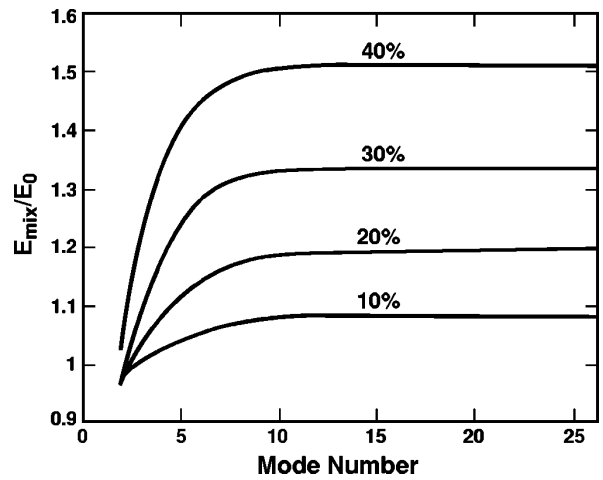
FIG. 2-7. The increase in the required driver energy vs the perturbation mode number for perturbation amplitudes as a fraction of the hot-spot radius of 10%, 20%, 30%, and 40% at peak compression (Kishony, 2001).
