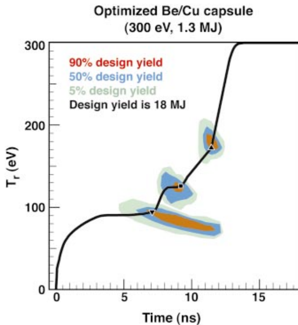
FIG. 2-4. (Color) Sensitivity of NIF ignition targets to pulse shape: the color scale shows yield variation as the drive profile is varied by moving the "peg-points" indicated by the small triangles. A wide range of pulse shapes provides good performance, but for a given pulse shape, the shocks generated must be accurate to 2%.
