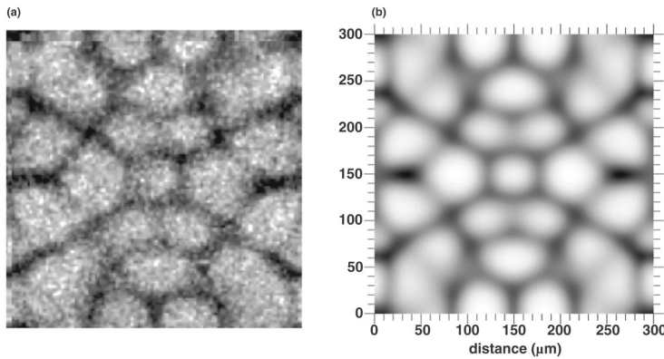
FIG. 6-16. (a) Experimental radiograph of the 3D multimode foil at 6.0 ns. Darkest regions correspond to greatest foil thickness (spikes). (b) Simulated radiograph at 6.0 ns, which includes the diagnostic resolution. Gray scales for (a) and (b) cover the same change in optical depth.
