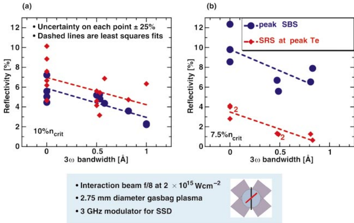
FIG. 3-19. (Color) Experiments using gasbag plasmas with the interaction beam outfitted with RPPs and 3 GHz SSD showed the benefit of SSD in reducing scattering. The SRS (◆) and SBS (●) reflectivity vs SSD bandwidth are shown for (a) 10% critical and (b) 7.5% critical gasbags filled with mixtures of \text{C}_5\text{H}_{12} and \text{C}_3\text{H}_8 .
