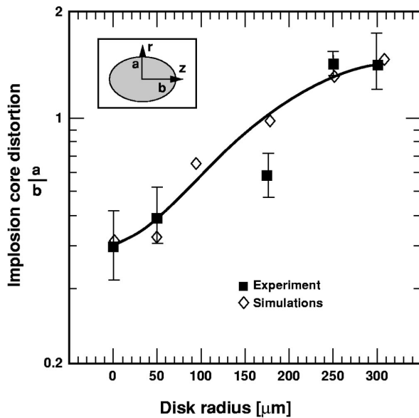
FIG. 5-22. Implosion core distortion vs disc radius for hohlraums of the type shown in Fig. 5-21.
