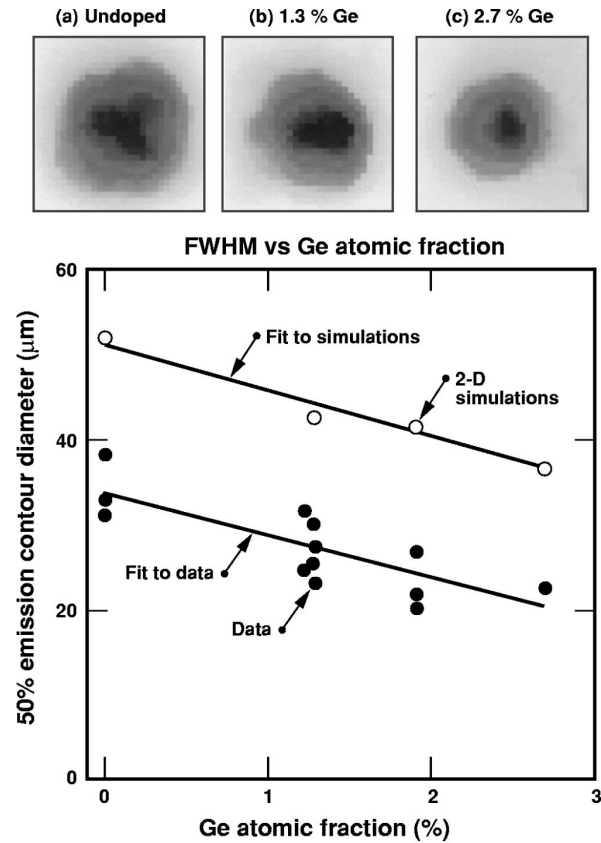
FIG. 7-14. X-ray images at 4 keV of imploded cores from smooth capsules at peak emission time for (a) no doping, (b) 1.3 at. % Ge, and (c) 2.7 at. % Ge. (d) Measured (solid circles) and calculated (open circles) azimuthally averaged diameters of 50% x-ray emission contours vs Ge doping. Solid lines are linear fits to data and simulations. The predicted smaller size of the x-ray emitting region as doping increases is consistent with the observations, although the absolute size of the emitting cores is smaller than calculated.
