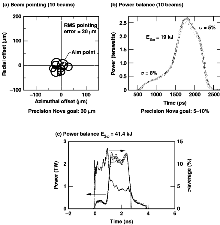
FIG. 1-5. The Nova laser power balance and beam pointing were improved a factor of 2 to 3 in the Precision Nova Project. These improvements were required for high-precision symmetry experiments and high-convergence implosions.
