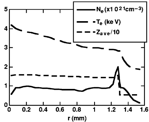
FIG. 3-25. The calculated electron density, temperature, and average ionization state at t=0.9 ns for a gasbag target containing 90% Xe and 10% C 5 H 12 . These conditions were insensitive to the percent of C 5 H 12 content, which was varied from 0% to 30% [R. K. Kirkwood et al. , Phys. Rev. Lett. 77, 2706 (1996)].
