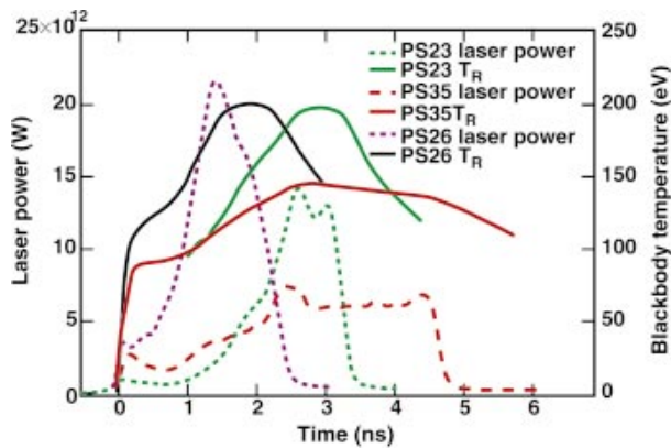
FIG. 6-7. (Color) Drive history for the three laser pulse shapes used in these experiments. The total laser power as a function of time for the drive beams is shown (left axis) in each case (the backlighter power history is not shown). The corresponding x-ray blackbody temperature is also shown for each pulse (right axis).
