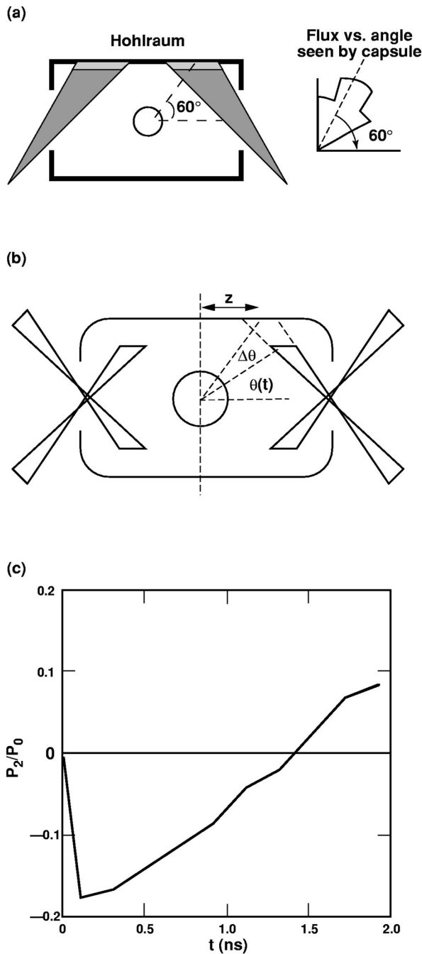
FIG. 5-5. (a) Schematic of a cylindrically shaped, Nova-like hohlraum that produces a collimated source flux vs angle approximately as shown in the flux vs polar-angle plot. (b) Schematic of laser-driven cylindrical hohlraum environment. As time evolves, the hohlraum wall blows in, intercepting the beam ring at smaller polar angle \theta . In addition, the unirradiated wall emissivity increases and the capsule radius decreases. (c) Predicted P_2 pressure asymmetry variation at capsule for a standard single Nova ring/side illumination hohlraum (1.6 mm diam \times 2.4 mm long with 1.2 mm diam LEHs, driven by a 20 TW peak power, 2.2 ns long, 3:1 contrast pulse [PS22]).
