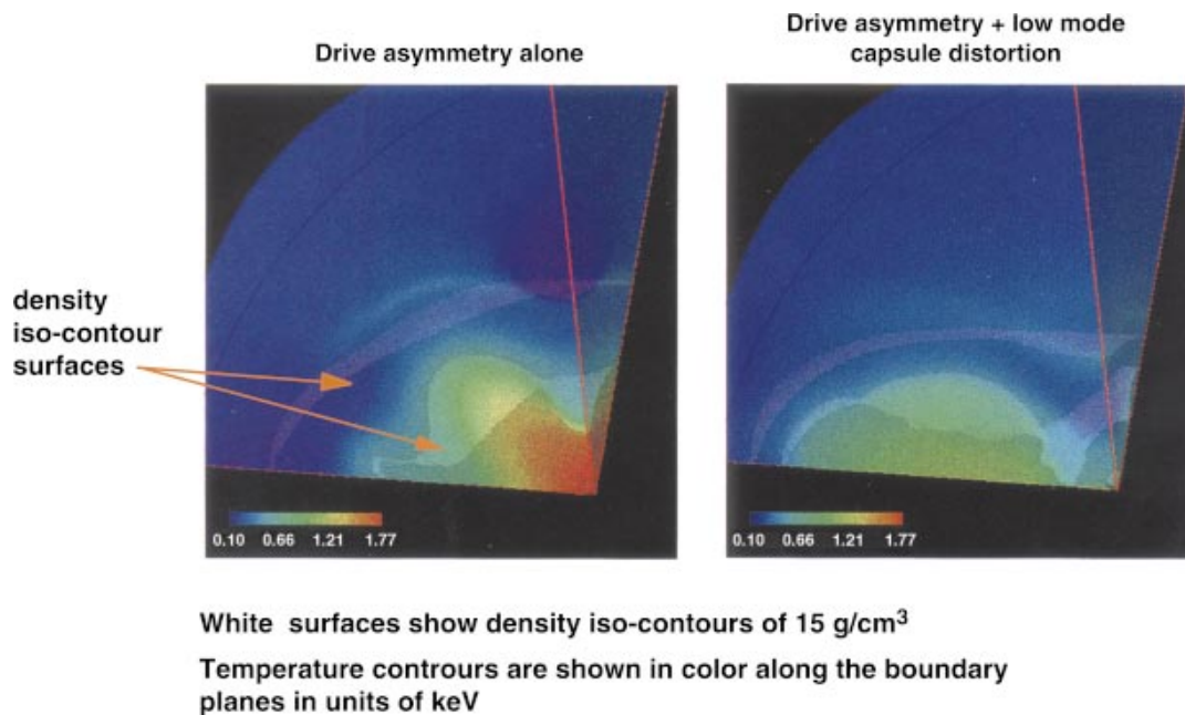
FIG. 7-17. (Color) 3D calculations of the HEP4 capsule implosions on Nova: (a) The distortion of an implosion due to Nova's intrinsic hohlraum radiation asymmetry. Nova's fivefold radiation pattern can be calculated with the 36° slice shown. Although the distortions shown are significant, the yield degradation from an unperturbed calculation is only about 30%. (b) The enhanced distortion which results from including a 2 \mu\text{m} offset between the inner and outer plastic shell surfaces, which was typical in the targets used in the HEP4 experiments, provides enough additional distortion that the temperatures are significantly lowered and the yield is reduced by about an additional factor of 2. With this level of degradation, the calculated and observed yields for smooth capsules are in agreement.
