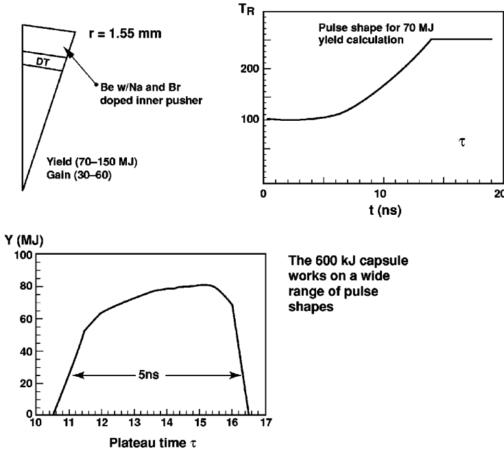
FIG. 2-24. With improved hohlraum coupling efficiency, it may be possible to drive a 250 eV Be design with ~100 MJ yield on NIF.
