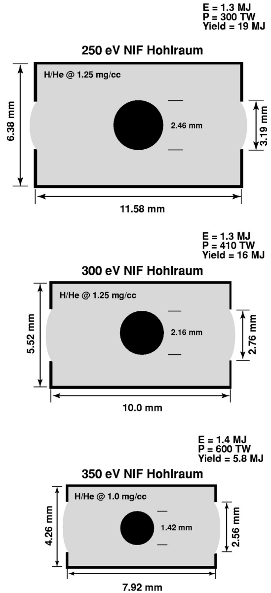
FIG. 2-17. Hohlräum designs have been developed for drive temperatures ranging from 250 eV to 350 eV. LASNEX 2D calculations have adequate symmetry for all three designs shown.
