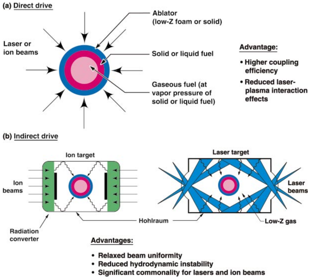
FIG. 1-1. (Color) ICF uses either (a) direct-drive (electron conduction) or (b) indirect-drive (x rays) to produce a high shell-ablation pressure to drive an implosion.
