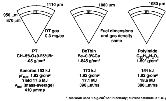
FIG. 2-3. We are evaluating CH, Be, and polyimide as possible ablator materials. These three designs have similar fuel implosion characteristics and could be driven in identical 300 eV hohlraums with nearly identical pulse shapes (1.3 MJ and 400 TW absorbed).
