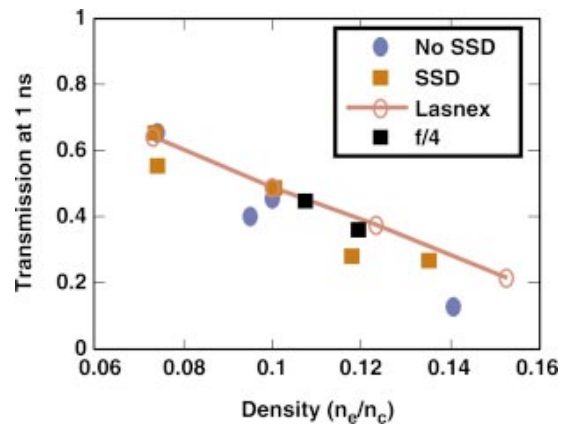
FIG. 3-24. (Color) The transmitted power fraction at 1 ns is compared to the LASNEX calculated fraction as a function of electron density for f/8 focusing with and without SSD and for f/4 focusing. The agreement is better for f/4 and SSD, both of which reduce filamentation [J. D. Moody et al. , Phys. Plasmas 7, 3388 (2000)].
