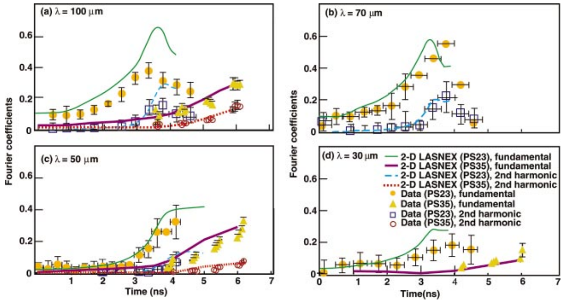
FIG. 6-10. (Color) Results of the wavelength scaling experiments (single mode). (a) \lambda = 100 \mu\text{m} , (b) \lambda = 70 \mu\text{m} (for the PS23 drive only), (c) \lambda = 50 \mu\text{m} , and (d) \lambda = 30 \mu\text{m} .
