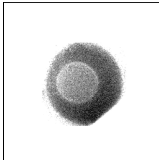
FIG. 5-12. Image of a 0.3 \text{ g}/\text{cm}^3 \text{SiO}_2 foam ball, backlit by 4.7 keV x rays on Nova.
