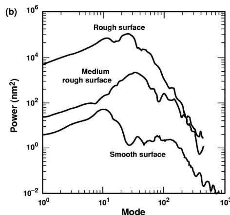
FIG. 7-6. (a) Scanning electron microscope (SEM) image of “bumpy-ball” target with a target surface \sigma = 1.7 \mu\text{m} . (b) The 2D (spherical surface) power spectra characterizing the outer surface of three representative HEP3 capsules with rms=0.03, 0.31, and 1.70 μm.
