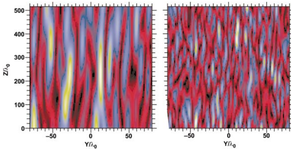
FIG. 3-4. (Color) Near “best focus,” the field of a random phase-plate beam consists of long, narrow speckles whose size depends on lens f number and laser wavelength. A simulated f/8 far field is shown on the left-hand side, an f/4 on the right-hand side. The transverse width of the speckles is linearly proportional to the f number while the axial length is quadratic in the f number.
