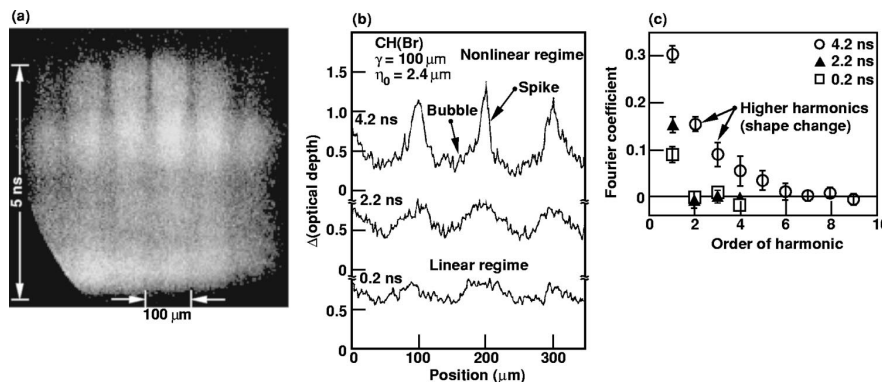
FIG. 6-9. Various representations are shown for the single-mode face-on data for a \lambda = 100 \mu\text{m} , \eta_0 = 2.4 \mu\text{m} perturbation imposed on a 48 \mu\text{m} thick CH(Br) foil. (a) The “raw” streaked image is shown as film density. The film response is removed using a calibrated exposure across a precision “P20” optical density wedge. (b) Profiles of \Delta (optical depth) \approx \Delta \ln(\text{exposure}) are shown at 0.2 ns, 2.2 ns, and 4.2 ns. (c) The real components of the Fourier transforms are given for the three profiles shown in (b). Note that at late time, the perturbation enters the nonlinear regime, and up to the fifth harmonic of the perturbation Fourier composition is observed.
