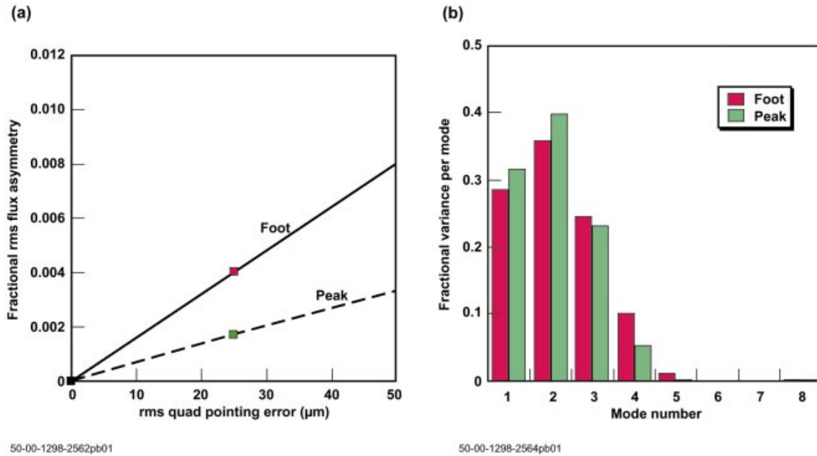
FIG. 2-21. (Color) (a) The rms capsule-flux asymmetry as a function of quad-to-quad pointing errors. The red and green squares indicate the estimated quad-to-quad pointing error for NIF. (b) Fractional contribution of each Legendre mode to total variance of the capsule flux due to beam pointing errors.
