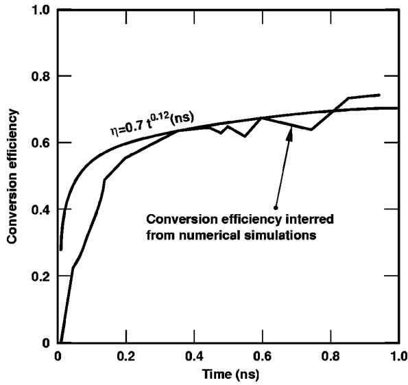
FIG. 4-5. Detailed numerical calculations of hohlraums with a 1 ns pulse predict an x-ray conversion efficiency that increases with time. A conversion efficiency given by \eta=0.7t^{0.12} is shown for comparison.
