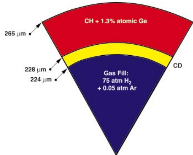
FIG. 7-18. (Color) Cross section of a typical deuterated-shell capsule design. Since the gas fill is inert, all the yield arises from conduction to the deuterated layer making these capsules more sensitive to mix at the fuel–pusher boundary than capsules whose yield comes from the gas fill.
