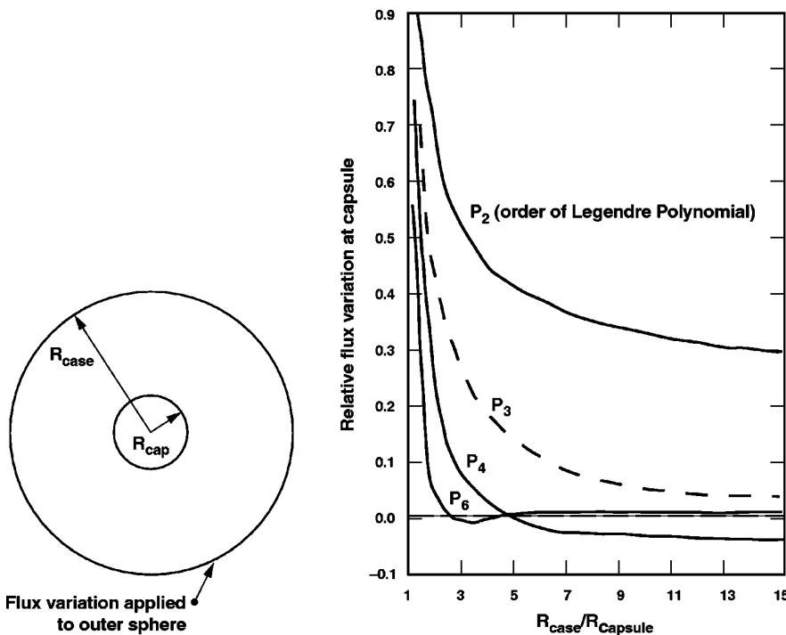
FIG. 5-1. Fraction of flux variation at wall that is imprinted at capsule as a function of ratio of case-to-capsule radius for various Legendre asymmetry modes. Hohlraums with R_{\text{case}}/R_{\text{capsule}} from about 3 to 5 effectively smooth all but the P_2 Legendre polynomial flux variations.
