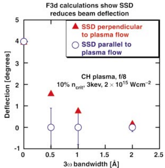
FIG. 3-9. (Color) SSD will be used to reduce beam deflection in flowing plasma. The current NIF baseline has SSD perpendicular to plasma flow in the hohlraum in order to minimize the focal spot smearing in the short direction of the elliptical NIF focal spot. Either orientation of SSD relative to the plasma flow will reduce beam deflection with modest bandwidth. Either orientation will be available on NIF with minimal setup requirements.
