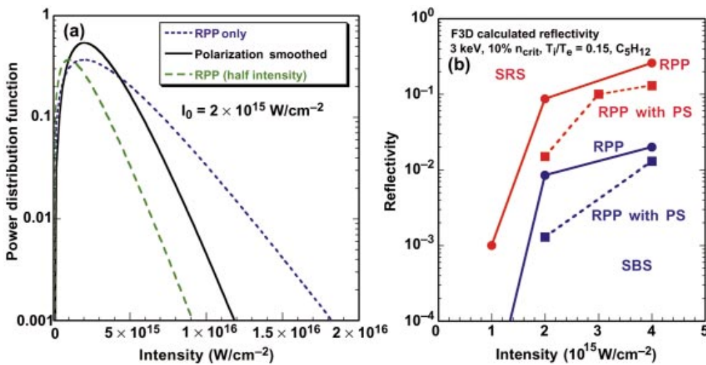
FIG. 3-8. (Color) Polarization smoothing (PS) reduces the fraction of the laser beam power at high intensity and hence reduces backscatter. (a) The distribution of laser power at the focal spot is shown vs intensity for one polarization (RPP), for two independent polarizations (PS) and for one polarization with half the total power. PS reduces the number of high-intensity hot spots, and narrows the distribution about the mean intensity. (b) In F3D calculations, PS reduces SRS and SBS backscatter.
