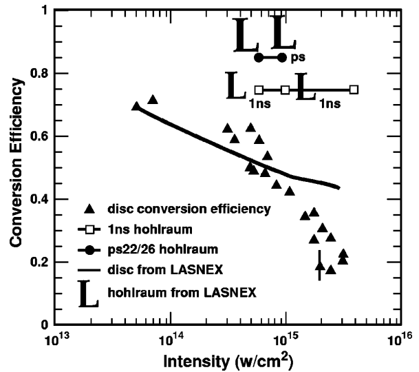
FIG. 4-9. Conversion efficiency of laser light into x rays for disks and hohlraums. Experimental number for hohlraums are inferred from wall loss data and measured temperatures.
