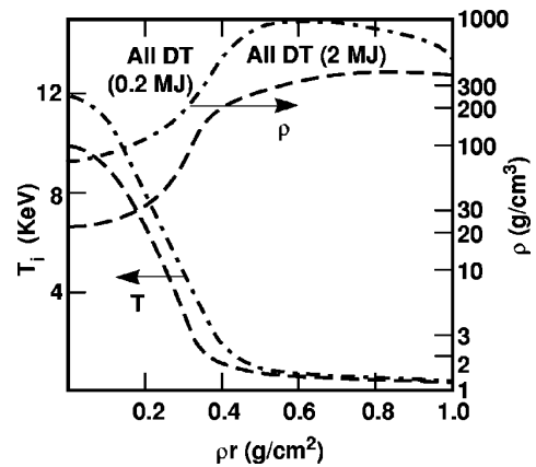
FIG. 1-8. Laboratory ignition and high-gain capsules have very similar ignition conditions. Hot-spot temperature profiles and \rho r are nearly independent of size at ignition. Smaller capsules must have higher density to achieve the required hot spot \rho r \approx 0.3 g/cm 2 .
