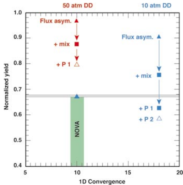
FIG. 7-29. (Color) Calculated normalized yield for the initial Omega indirect drive implosion series vs neutronic convergence for doped, low- (red) and high- (blue) convergence target. Range of HEP4 Nova data is shown in green. Horizontal blue line is calculated normalized yield for the high-convergence target subject to 1/3 mix penetration fraction of fuel. The baseline NIF ignition capsules fail to ignite with mix above this level. Solid diamonds represent cumulative (multiplicative) effect of simulated intrinsic flux asymmetry and random laser power imbalance. Multiplicative effects of capsule P1 , P2 distortions and surface roughness are as indicated.
