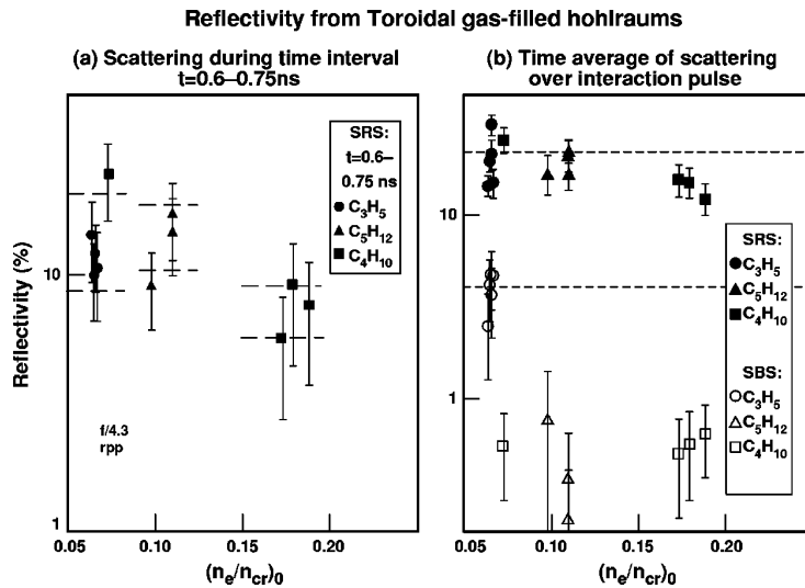
FIG. 3-34. (a) Instantaneous R_{SRS} at time= 0.675 \pm 0.075 ns based on the measured light leaving the hohlraum are plotted vs initial n_e/n_c of the gas fill. A range equal to one standard deviation above and below the average reflectivity for each density is indicated. (b) Similar plot of the time-averaged R_{SRS} and R_{SBS} . For all these shots, the laser intensity at the hohlraum laser entrance hole is 2 to 3 \times 10^{15} W/cm 2 [J. C. Fernandez et al. , Phys Plasmas 7, 3743 (2000)].
