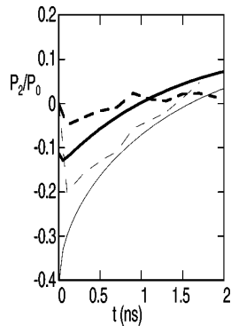
FIG. 5-28. Time dependence of P_2/P_0 pressure asymmetry at a foam ball calculated by the simplified analytical model (dashed curves) and by 2D Lasnex simulations (solid curves). The lower and upper curves are for an initial beam ring position from the hohlraum midplane of z=430 \mu\text{m} and 530 \mu\text{m} , respectively.
