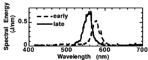
FIG. 3-26. Time-integrated SRS spectra from a Xe-filled gasbag with a 5.5% C 5 H 12 content for the “early phase” from 0.5 to 1.0 ns while the heater beams are on, and from the “late phase” from 1.0 to 1.5 ns after the heater beams have turned off. The frequency shift after the heater beams turns off is consistent with cooling of the plasma [R. K. Kirkwood et al. , Phys. Rev. Lett. 77, 2706 (1996)].
