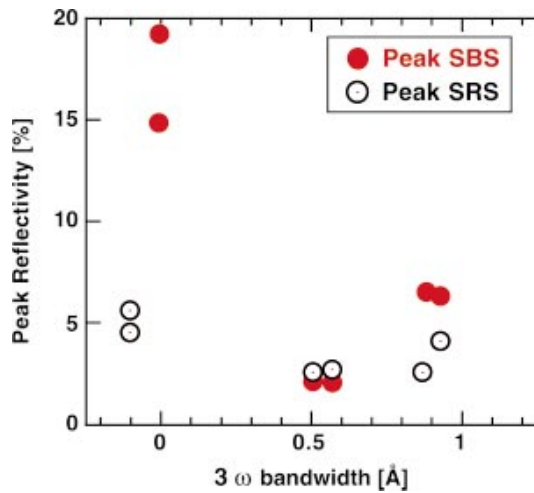
FIG. 3-38. (Color) Nova scale-1 hohlraums simulating the NIF outer beam plasma, SSD beam smoothing reduces backscatter significantly. SBS and SRS backscatter data from scale-1, methane-filled hohlraums with a Au-shelf plasma are similar to those encountered by the NIF outer beams. The reflectivity shown is the peak in time (averaged over the 50 ps diagnostic resolution) corresponding to the time of peak incident intensity ( 2.5 \times 10^{15} W/cm 2 ). In these experiments, the interaction beam was smoothed using a 3 GHz SSD and an RPP [S. H. Glenzer et al. , Phys. Plasmas 8 , 1692 (2001)].
