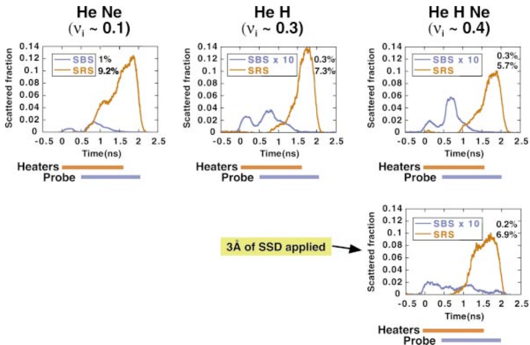
FIG. 3-29. (Color) Time histories of SRS and SBS in HeH ( v_i=0.3 ), HeNe ( v_i=0.1 ), and HeHNe ( v_i=0.4 ) gasbag plasmas are similar to those in gasbags with hydrocarbon fills. The time-integrated reflectivity is also given on each figure. The peak scattering only depends weakly on the ion damping for these low-Z NIF-like gas fills [J. D. Moody et al. , “First measurement of backscatter dependence on ion acoustic damping in a low-Z, high density laser-plasma,” Phys. Plasmas (to be submitted)].
