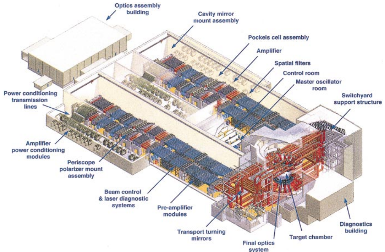
FIG. 1-11. (Color) The NIF is being designed with the energy, power, and precision required to demonstrate ignition and propagating burn in ICF.
