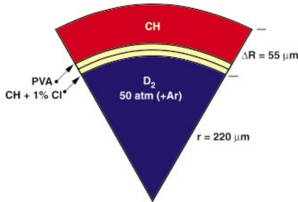
FIG. 7-5. (Color) Schematic of the capsules used in the HEP3 experiments.
