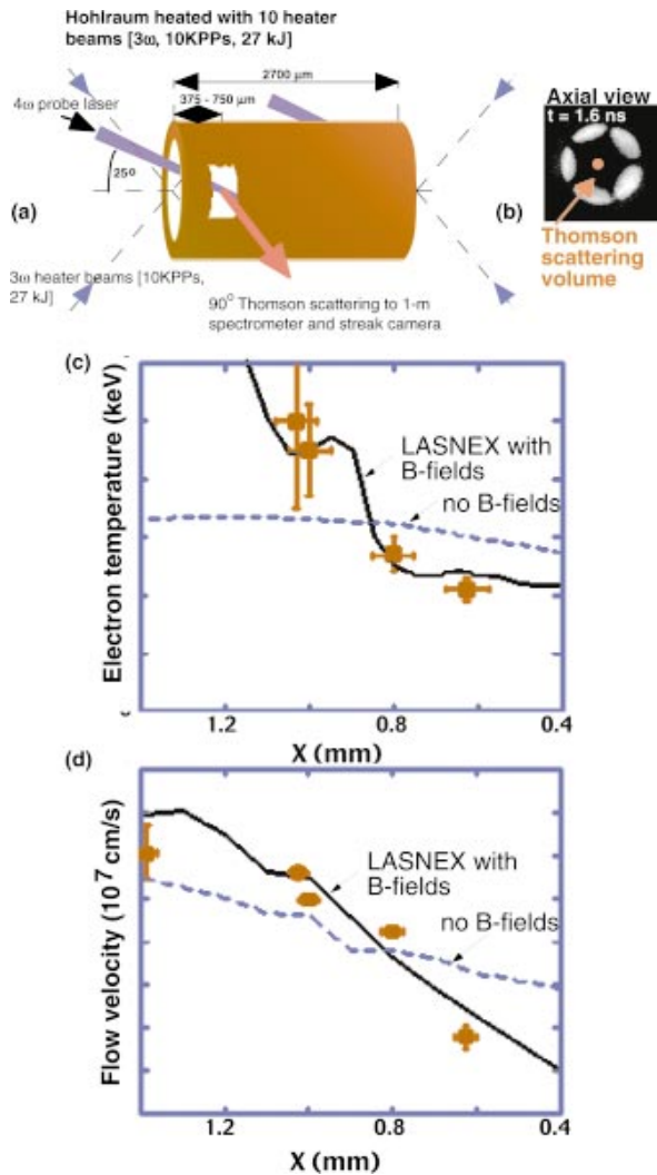
FIG. 3-35. (Color) (a) The 2.4 ns f/4 351 nm laser beams used to heat the scale-1 Nova gas-filled hohlraum and the Thomson scattering configuration are shown schematically. The interaction beam had the same pulse shape and duration as the heater beams. (b) An axial view in x-ray emission. The electron temperature (c) and the flow velocity component along the hohlraum axis (d) measured with Thomson scatter, are shown in the bottom two figures. Only with magnetic fields in LASNEX are the measurements simulated correctly [S. H. Glenzer et al. , Phys. Plasmas 6 , 2117 (1999)].
