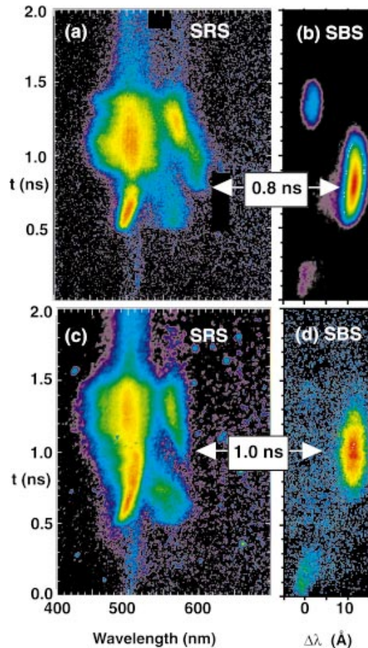
FIG. 3-33. (Color) The time history of the SRS spectrum (a) and the SBS spectrum (b) in propane-filled (C3H8) hohlraums for the standard toroidal hohlraum length shows an earlier onset of SBS and disruption of SRS than that of the SRS spectrum (c) and SBS spectrum (d) of a toroidal hohlraum whose length was increased by 0.25 mm [J. C. Fernandez et al. , Phys Plasmas 7, 3743 (2000)].
