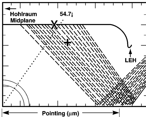
FIG. 5-18. Cutaway at t=0 from a 2D simulation of a hohlraum containing a pure plastic capsule with a realistic representation of Nova's beams. The calculation is cylindrically symmetric around the horizontal axis and left-right symmetric across the midplane. The beams enter through LEH's at the ends of the hohlraum. "Pointing" is the distance between the midplane and where the beams "cross" (i.e., the reflection off the horizontal, rotational axis of symmetry), generally chosen to be in the plane of the LEH.
