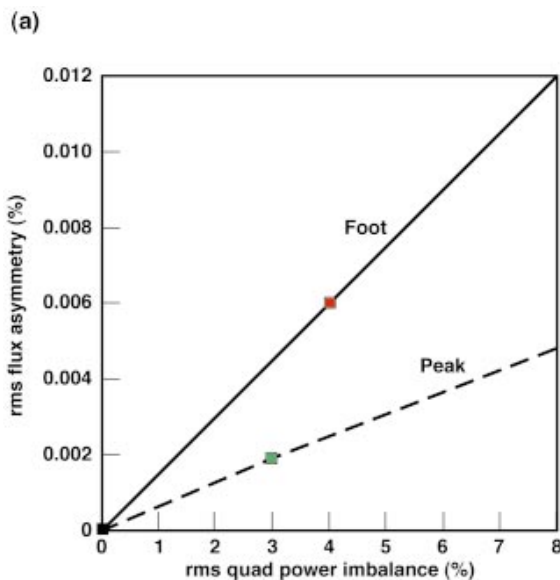
FIG. 2-20. (Color) (a) The rms capsule-flux asymmetry as a function of amount of quad-to-quad power imbalance. The red and green squares indicate the rms quad power imbalance estimated for NIF from Fig. 2-19. (b) Fractional contribution of each Legendre mode to total variance of the capsule flux due to power imbalance.
