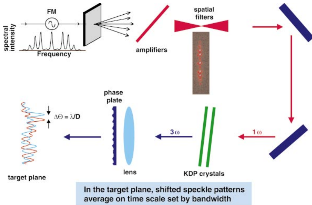
FIG. 3-13. (Color) SSD on Nova is applied by frequency modulating and dispersing the pulse (FM SSD) prior to amplification and conversion to 3\omega .
