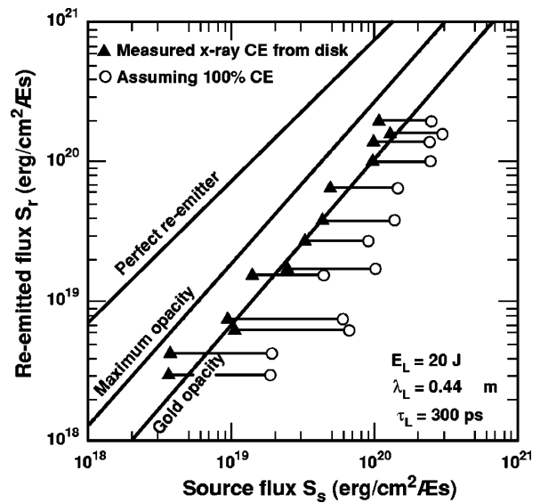
FIG. 4-11. Experiments at Garching with low energy and short pulses do not see significant enhancement of x-ray production in hohlraums compared to open-geometry measurements.
