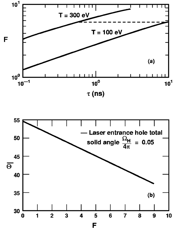
FIG. 5-4. (a) The hohlraum smoothing factor F versus pulse length. F is the ratio of the x-ray flux from the hohlraum wall to the flux from the laser hot spots. (b) The required laser source angular location \theta to zero P_2 versus hohlraum smoothing parameter F . As the hohlraum wall flux increases, the laser spot must be closer to the laser entrance hole to compensate for the deficit in flux from the LEH.
