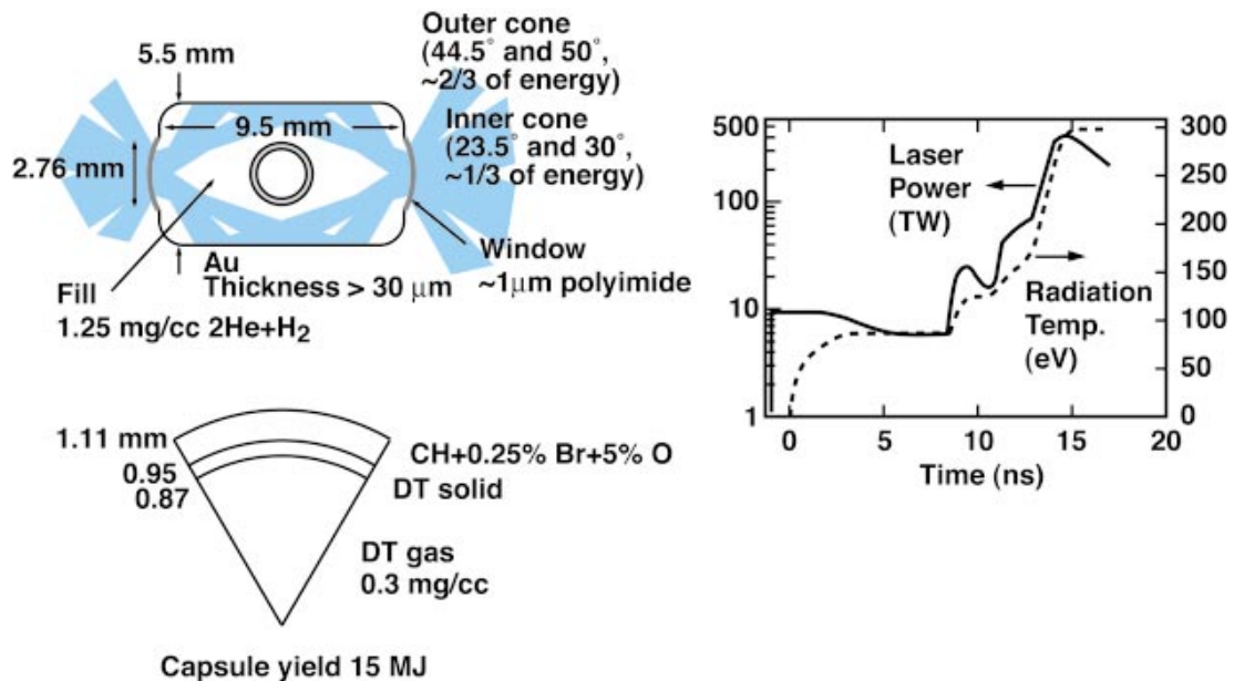
FIG. 2-1. (Color) The most extensive modeling of ignition has concentrated on this target, called the point-design target (PT), that absorbs about 1.3 MJ of light.
