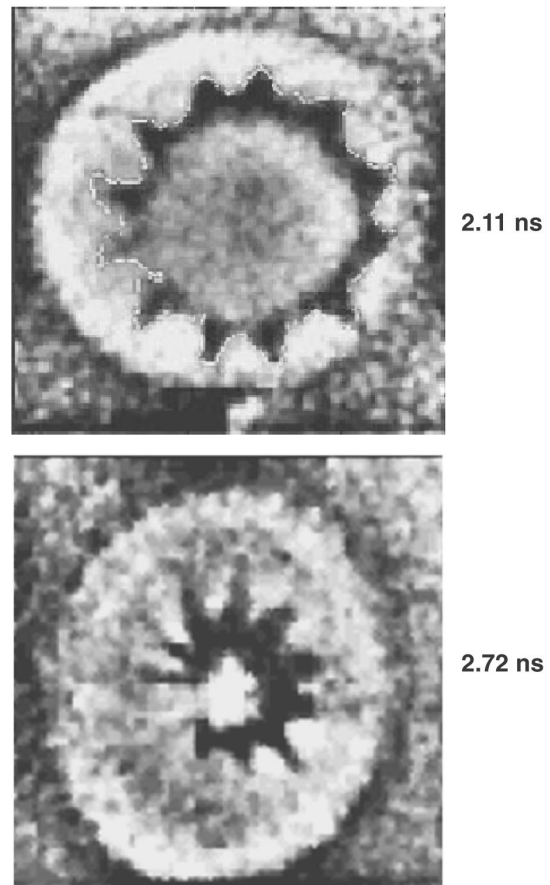
FIG. 6-18. (a) An outer contour of the cylindrical implosion experiment taken at 50% peak exposure, superposed over an x-ray image taken at 2.11 ns. (b) Cylinder at 2.72 ns.
