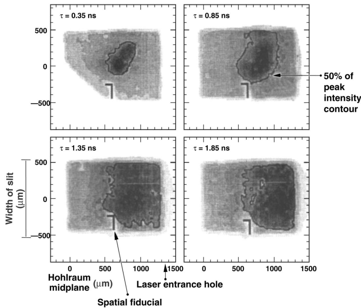
FIG. 5-6. A well-defined soft x-ray spot that moves toward the LEH is observed. Data are obtained by looking at soft x-ray emission through a 1 mm wide slot cut in the hohlraum wall.
