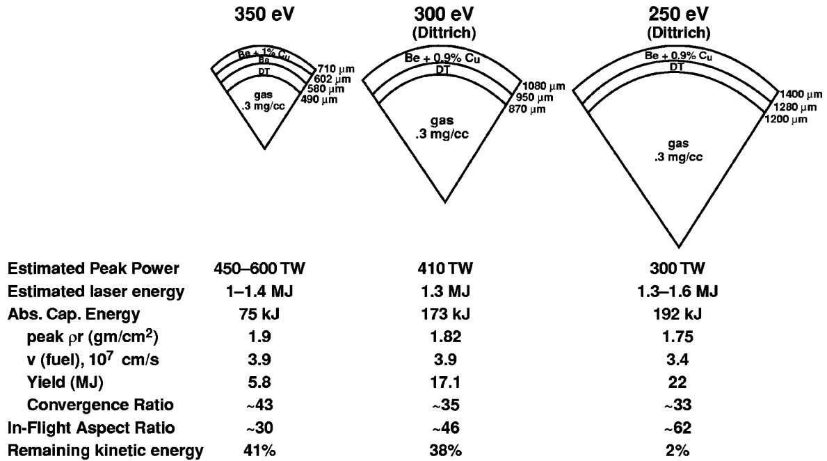
FIG. 2-12. Capsules being designed for NIF span a range of temperatures from 250 eV to 350 eV.
