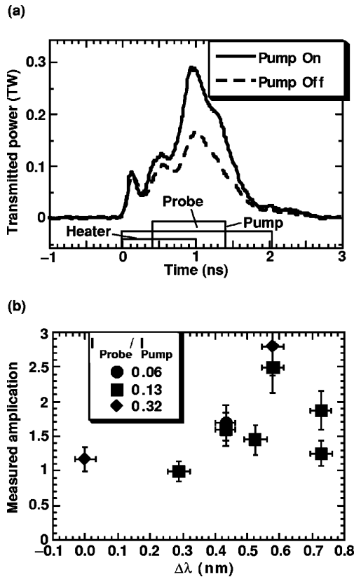
FIG. 3-41. (a) Measurement of the probe-beam power transmitted through the plasma for the case \Delta\lambda = 0.45 nm and I_{\text{probe}}/I_{\text{pump}} = 0.06 . In the “pump on” case, a 2 \times 10^{15} W/cm 2 pump beam intersects the probe between 0.4 and 1.4 ns, causing the probe to be amplified by a factor of 1.7 above the “pump off” case. (b) A series of experiments measured the amplification of the probe beam as a function of the wavelength separation of the two beams. The amplification is greatest when the frequency separation is in the vicinity of the prediction for the unshifted ion wave resonance, \Delta\lambda = 0.45 \pm 0.04 nm [R. K. Kirkwood et al. , Phys. Rev. Lett. 76 , 2065 (1996)].
