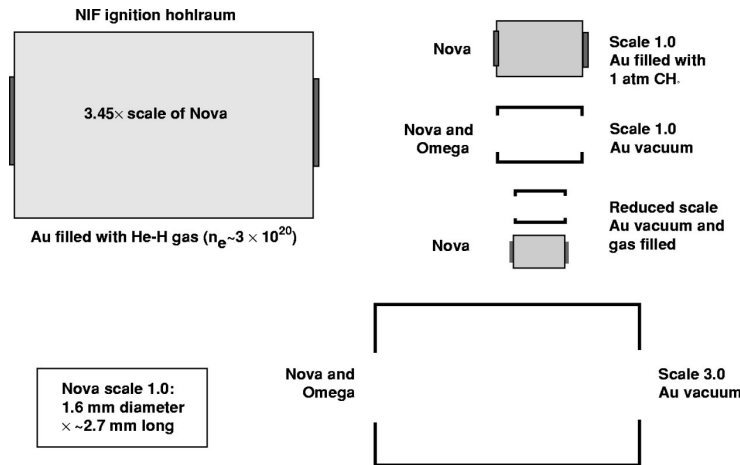
FIG. 4-1. Hohlraum x-ray drive has been studied in a wide range of hohlraums on the Nova and Omega laser.
