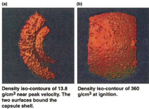
FIG. 2-9. (Color) A HYDRA simulation has resolved the full range of the most dangerous modes ( l \approx 2-100 ) that grow from surface roughness on a NIF capsule. (a) Density iso-contours of 13.8 g/cm 3 near peak velocity. The two surfaces bound the capsule shell. (b) Density iso-contour of 360 g/cm 3 at ignition.
