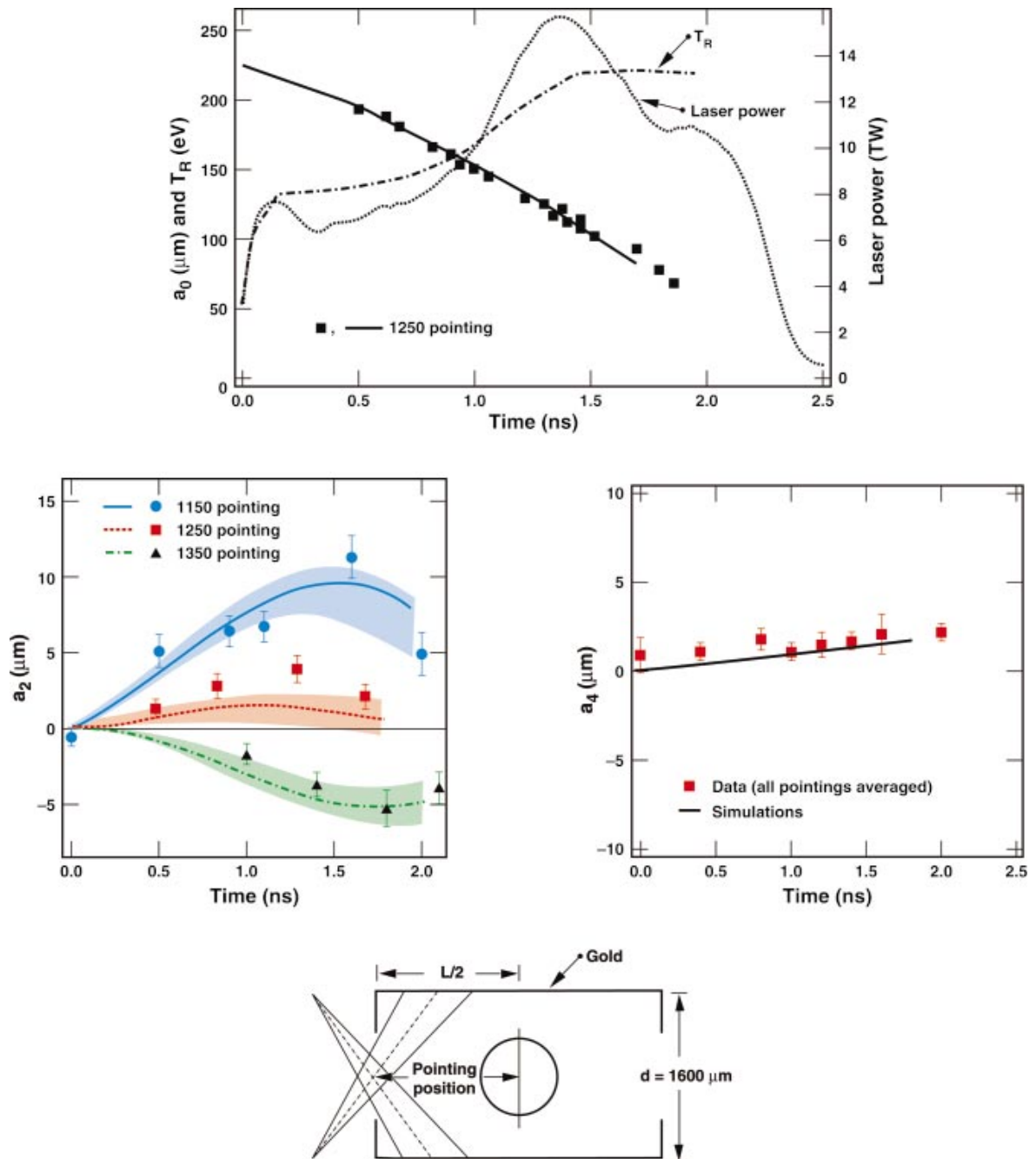
FIG. 5-13. (Color) Coefficients of zeroth, second, and fourth Legendre polynomials from the pointing scan experiment. Data are obtained from backlit foam balls of the type shown in Fig. 5-12. The laser power history and resulting radiation temperature are also shown on the a_0 plot.
