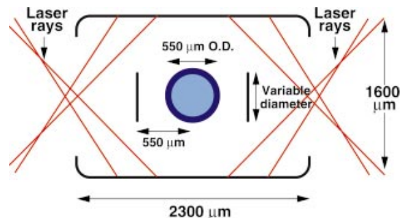
FIG. 5-21. (Color) Schematic of a Nova Au hohlraum with Au disks centered at z = \pm 550 \mu\text{m} . Capsule and hohlraum dimensions are as indicated.
