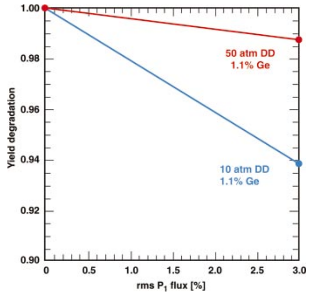
FIG. 7-28. (Color) Calculated neutron yield degradation vs rms P_1 \equiv (Y_{1,-1}^2 + Y_{1,0}^2 + Y_{1,1}^2)^{1/2} laser flux for doped, low- (red) and high- (blue) convergence targets.
