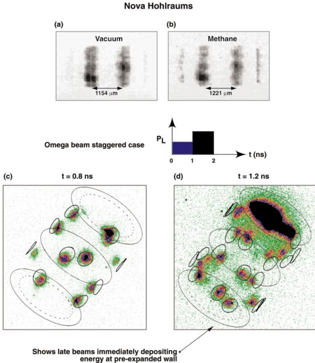
FIG. 5-8. (Color) X-ray images of laser spots from Nova and Omega hohlraums. The hohlraums have 2 \mu\text{m} thick walls and transmit x rays with h\nu > 5 \text{ keV} . (a) and (b) Images from Nova hohlraums, perpendicular to the hohlraum axis, for vacuum and 1 atm methane-filled hohlraums, respectively. (c) and (d) Images from an Omega vacuum hohlraum taken from a compound angle. Image (c) is taken at the end of the first set of beams, while (d) is taken at the beginning of the second set of beams. Open circles show expected beam positions without spot motion.
