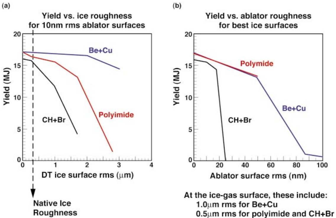
FIG. 2-10. (Color) 3D simulations with HYDRA show that at 300 eV drive, the BeCu NIF capsule can tolerate the roughest ice-gas and ablator surfaces. (a) Yield vs ice roughness for 10 nm rms ablator surfaces. (b) Yield vs ablator roughness for best ice surfaces.
