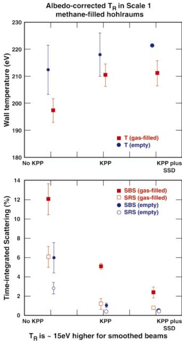
FIG. 4-13. (Color) Ten smoothed beams reduced backscatter losses and raised hohlraum temperature.
