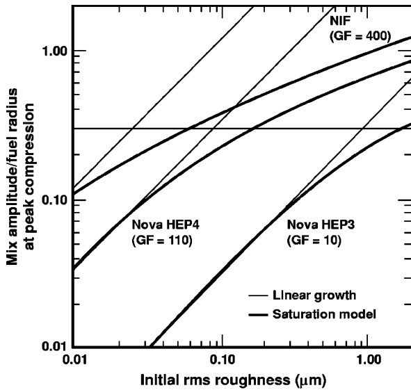
FIG. 7-8. Calculated mix amplitude (normalized to fuel radius at peak neutron emission time) vs initial surface roughness. Starting from the right, the three curves correspond to the low-growth HEP3 design, the higher-growth HEP4 design, and the NIF design. Black and gray curves correspond to calculations with and without growth saturation, respectively. The section of the NIF curve above a normalized mix amplitude of 0.33 corresponds to loss of ignition for the baseline ignition capsule discussed in Sec. II.
