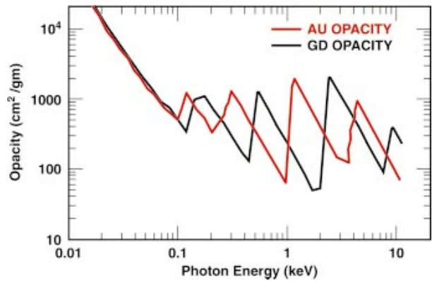
FIG. 4-7. (Color) Mixing Gd with Au results in a material (cocktail) with a higher mean opacity than pure Au. Peaks in the Gd opacity complement the windows in the Au opacity.
