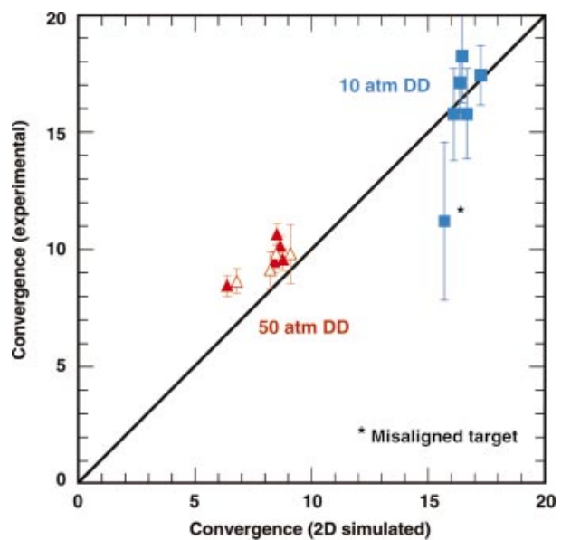
FIG. 7-23. (Color) Experimental neutron convergence vs predicted neutron convergence based on 2D simulations for doped (solid) and undoped (open), low- (red) and high- (blue) convergence targets.
