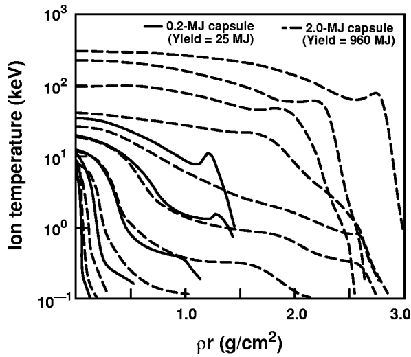
FIG. 1-9. Burn propagation in small capsules tracks that in larger capsules until decompression begins. Pairs of curves are temperature contours at a series of times as the burn wave propagates through the fuel.
