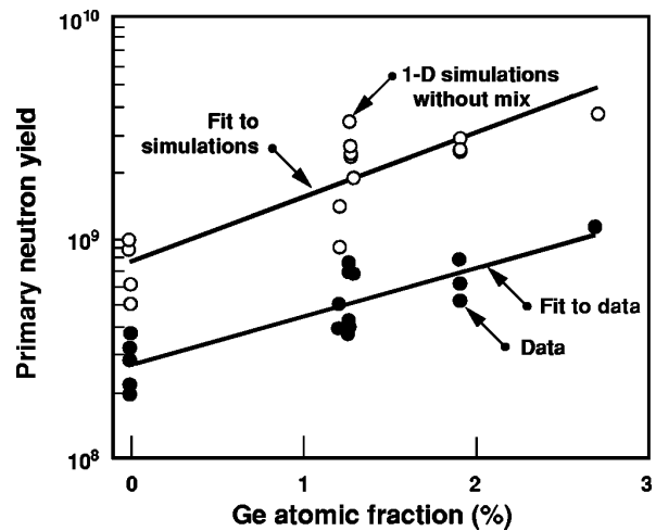
FIG. 7-13. Measured and calculated primary (DD) neutron yields from 1D simulations without mix or asymmetry vs doping for smooth capsules. Solid lines are linear fits to data and simulations. Doping the capsules to suppress radiative preheat results in denser implosions. Capsule yield increases with doping as expected but absolute yields are degraded by mix and asymmetry.
