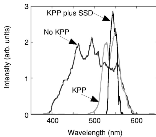
FIG. 3-37. SRS spectra from gas-filled hohlraums at 1.8 \text{ ns} < t < 2 \text{ ns} for various smoothing conditions. With improved smoothing the spectra narrow from 180 nm to 30 nm.
