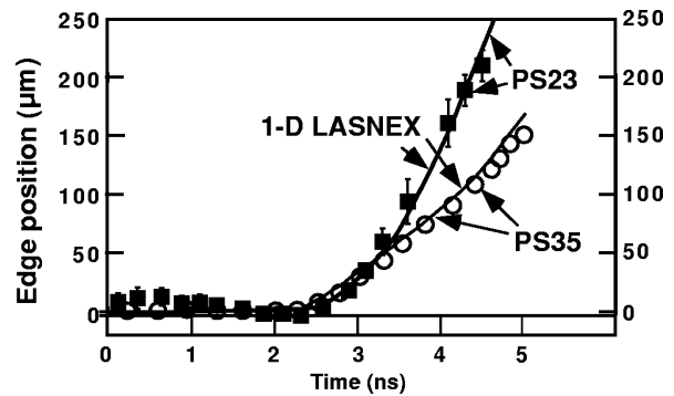
FIG. 6-8. Foil trajectory for the planar geometry experiments. The plotting symbols represent the measured position of the rear edge (side away from the x-ray drive) of the foil as a function of time. The two pulse shapes used for planar geometry experiments are represented as PS23 and PS35 (see Fig. 6-5). The error bars arise from the uncertainties in defining the edge. The solid curves are the results of 1D LASNEX simulations. Note that the rear edge of the foil does not start to move until after shock breaks out.
