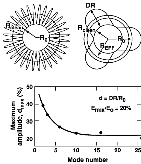
FIG. 2-6. At high l -mode numbers ( l > 10 ), the DT contained within the bubbles does not contribute to ignition—only the clean inner part of the hot spot ignites (Kishony, 2001). As the l -mode decreases below 10, the ratio of the surface area of the cold spikes to hot-spot volume decreases, allowing a larger effective radius to contribute to ignition. The case shown is for E_{mix}/E_0 = 20\% , an implosion with a 20% ignition margin (Kishony, 2001).
