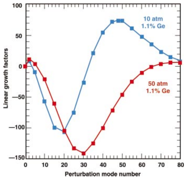
FIG. 7-26. (Color) Calculated small-amplitude growth factors vs Legendre mode number for doped, low- (red) and high- (blue) convergence targets.
