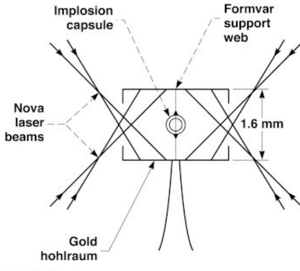
FIG. 1-4. (Color) Nova implosion target illustrating beam geometry. Five Nova beams irradiate each side of the hohlraum. The beams are uniformly distributed around the rim of a 100° cone.
