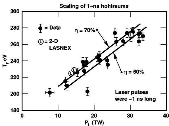
FIG. 4-3. Peak drive temperatures from Au hohlraums are in accord with 2D LASNEX simulations. The conversion efficiency inferred from hohlraum simulations for 1 ns pulses is consistent with \eta_{ce} \sim 70\% from the measured TR and wall-loss measurements.
