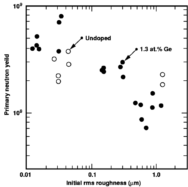
FIG. 7-15. Measured primary neutron yields for 1.3 at. % Ge-doped (solid circles) and undoped (open circles) capsules vs initial rms surface roughness. As expected, the yield of the denser more unstable doped capsules, is more sensitive to surface roughness than the undoped capsules.
