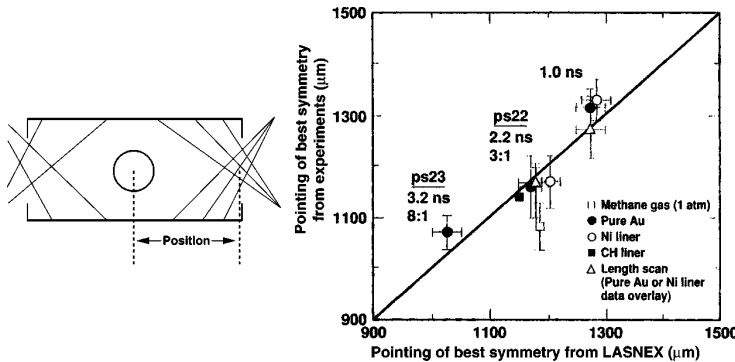
FIG. 5-20. LASNEX successfully predicts the pointing of best symmetry for almost all symmetry experiments. Beams must be moved inward for longer pulses to compensate for spot motion caused by hohlraum wall blow-off. Without beam smoothing, the experimental pointing of best symmetry is offset from the calculations by about 150 \mu\text{m} for the methane-gas-filled hohlraums.
