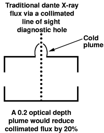
FIG. 4-14. Previous drive measurements through a diagnostic hole were often difficult to model at later times. This late-time disagreement is likely a 3D hole closure effect, which is not currently modeled in 2D hohlraum calculations.
