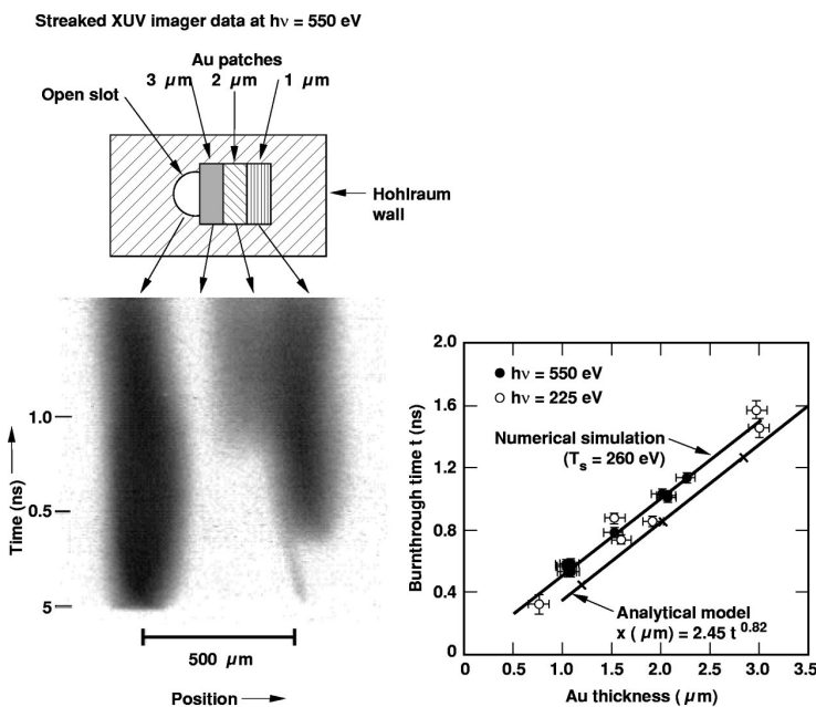
FIG. 4-6. The radiation-wave burnthrough measurements in thin Au foils agree well with numerical simulations and analytical models.
