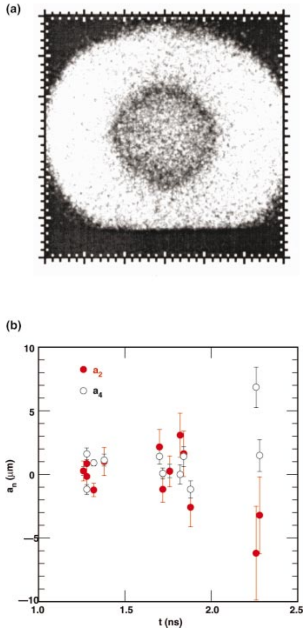
FIG. 5-14. (Color) Backlit shells also provide data on implosion symmetry. (a) A CH shell doped with 3% Ge and backlit with 4.7 keV x rays. (b) The ( a_2 ) and ( a_4 ) coefficients vs time.
