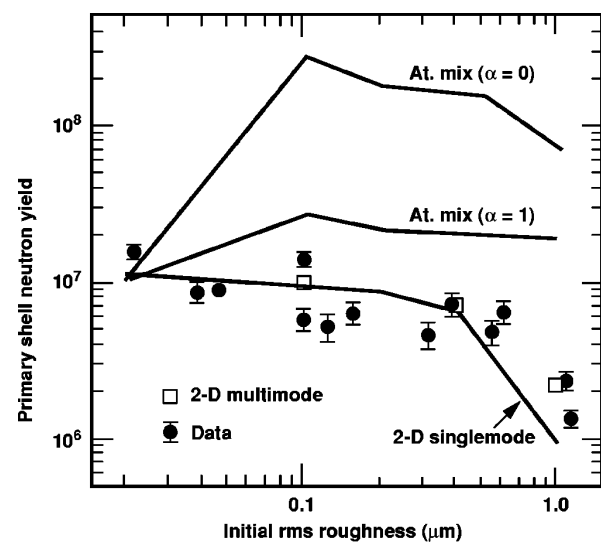
FIG. 7-19. Measured and calculated primary yields for 1.3 at. % Ge-doped deuterated-shell capsules vs initial surface roughness. Solid circles are the data with indicated experimental uncertainties. The middle and top curves are predictions from the 1D atomic mix model with ( \alpha=1 ) and without ( \alpha=0 ) enhanced heat diffusion. The lower curve and squares are predictions from 2D single-mode ( l=24 ) and multimode ( l=2, 4, 6, \dots, 48 ) simulations.
