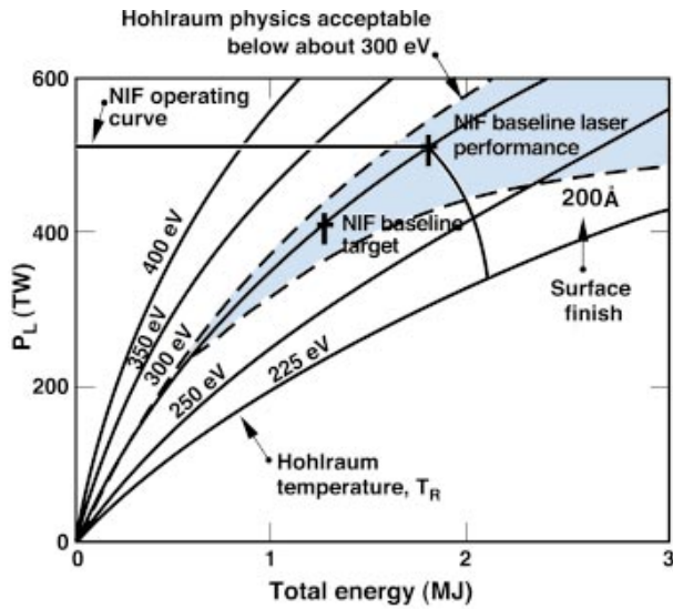
FIG. 1-7. (Color) For laser-driven indirect-drive ignition targets, plasma physics issues constrain the achievable hohlraum temperature and hydrodynamic instabilities (represented here by surface finish) establish the minimum required temperature at a given drive energy. The shaded region constitutes the accessible region in power-energy space where ignition with indirect-direct capsules is predicted. The NIF power-energy operating curve shown here has margin to allow for uncertainty in ignition capsule physics.
