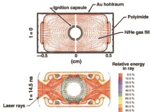
FIG. 2-16. (Color) 2D LASNEX calculations of NIF ignition targets are performed in order to accurately model the laser propagation and collisional absorption, the hohlraum, and the capsule. (a) The initial numerical grid from a typical calculation (Krauser et al. , 1996) of the PT ignition point design. (b) The numerical grid and material boundaries near the peak of the laser pulse. The numerical grid for the interior of the fusion capsule is not shown but is included in the calculation. The color tables for the laser rays indicate the remaining fraction of the incident laser energy. Most of the laser energy is transmitted through the H/He gas fill and is absorbed in the Au wall.
