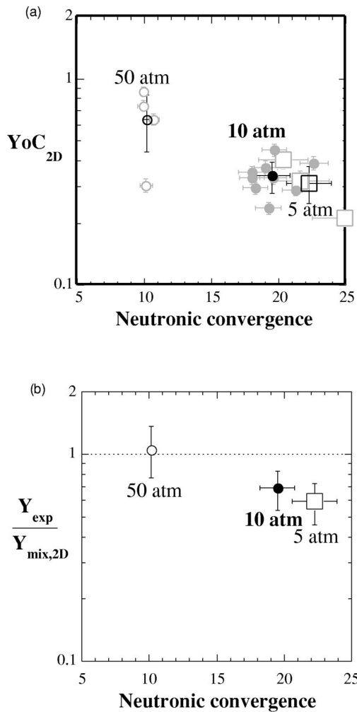
FIG. 7-33. (a) Ratio of measured primary (DD) neutron yield over clean 2D simulated yield vs inferred fuel convergence from secondary (DT) neutrons for 5 atm D 2 -filled capsules (open squares), 10 atm D 2 -filled capsules (filled circles), and 50 atm D 2 -filled capsules (open circles). Bold symbols denote averaging over each target type. (b) Averaged ratio of measured primary (DD) neutron yield to 2D simulated yield with 1D mix model vs inferred fuel convergence from secondary (DT) neutrons.
