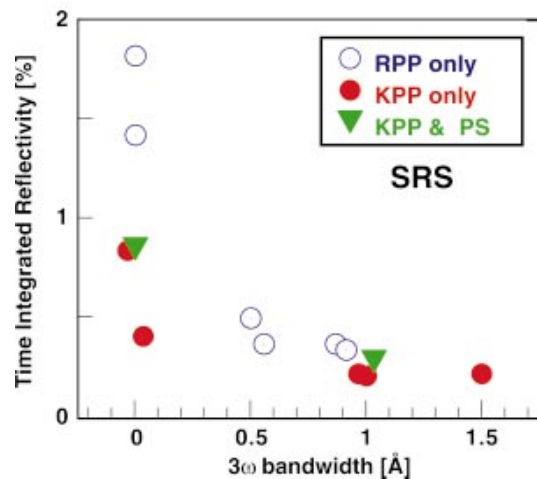
FIG. 3-39. (Color) SBS and SRS from Nova scale-1 hohlraums with NIF-like smoothing using 17 GHz SSD with a KPP. The reflectivities are similar to those from earlier Nova scale-1 hohlraum experiments using 3 GHz SSD and an RPP. Polarization smoothing does not have a significant effect for these plasma and laser conditions [S. H. Glenzer et al. , Phys. Plasmas 8 , 1692 (2001)].
