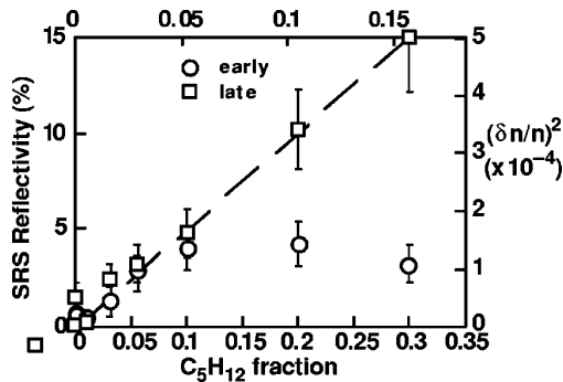
FIG. 3-27. SRS reflectivities from Xe-filled gasbag targets averaged over the “early period” and the “late period” are shown vs C_5H_{12} concentration. The calculated ion-wave damping is proportional to the C_5H_{12} concentration. The square of the fluctuation amplitude is estimated from the reflectivity [R. K. Kirkwood et al. , Phys. Rev. Lett. 77 , 2706 (1996)].
