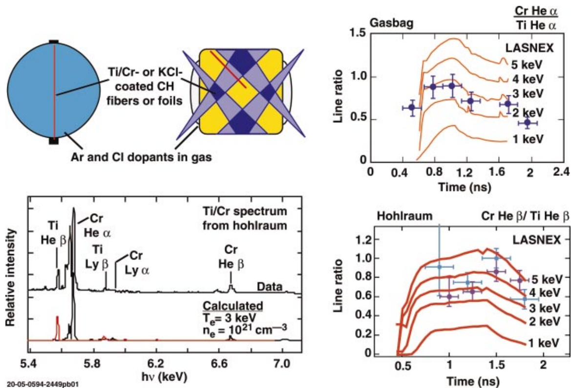
FIG. 3-17. (Color) X-ray spectroscopy indicates T_e \approx 3 keV for both open and closed geometries designed to approach NIF low-Z inner beam conditions on Nova. The theoretical time history of the line ratios for the gasbags and hohlraums is calculated for plasmas with the peak temperature indicated and with a time history of the temperature from LASNEX calculations. The nominal LASNEX calculations predict peak temperatures of slightly more than 3 keV.
