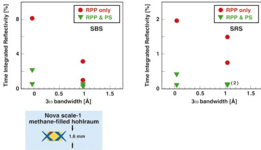
FIG. 3-40. (Color) Scale-1 hohlraum experiments at 4 \times 10^{15} W/cm 2 using 17 GHz SSD and an RPP were designed to stress LPI for the outer NIF beams. The experiments simulate conditions for the NIF outer beams in a 350 eV hohlraum. The SBS and SRS are still low with SSD, and the addition of polarization smoothing has a clear impact [S. H. Glenzer et al. , Phys. Plasmas 8 , 1692 (2001)].
