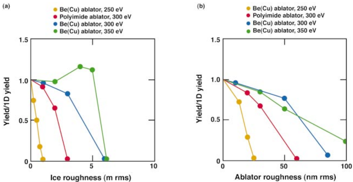
FIG. 2-13. (Color) For the current designs, tolerance to RT instability is a strong function of peak-drive temperature and capsule ablator material.
