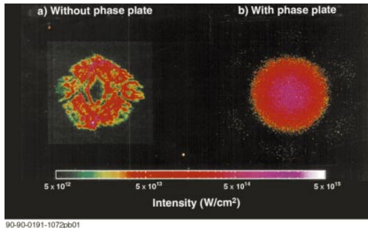
FIG. 3-5. (Color) Two laser beam spots with the same spot-averaged intensity are shown. On the left-hand side is an f/4 Nova spot 1 mm past best focus, typical of the unsmoothed beam in Nova hohlraums at the LEH. On the right-hand side is an RPP-smoothed beam. A phase plate produces a more uniform focal spot distribution and smaller speckle sizes for the same spot-averaged intensity.
