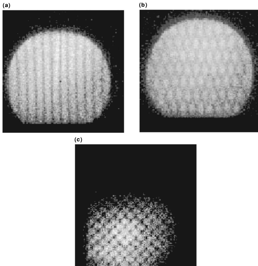
FIG. 6-13. Images from the 3D single-mode Nova experiments are shown in (a)–(c). The perturbations correspond to (a) 2D \lambda = 50 \mu\text{m} , \eta_0 = 2.5 \mu\text{m} , (b) 3D k_x = 3k_y : \lambda_x = 53 \mu\text{m} , \lambda_y = 158 \mu\text{m} , \eta_0 = 2.4 \mu\text{m} , and (c) 3D k_x = k_y , \lambda_x = \lambda_y = 71 \mu\text{m} , \eta_0 = 2.7 \mu\text{m} .
