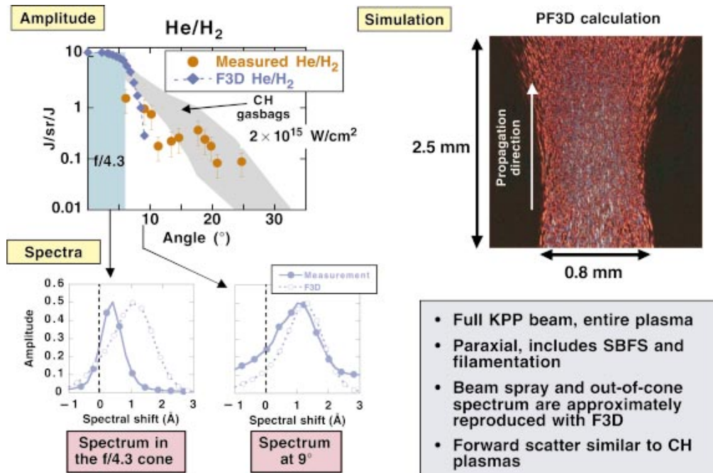
FIG. 3-30. (Color) Calculations of the forward scatter from the HeH experiments using the parallel F3D code. These results are in good agreement with the observed scattering out to about 10°. The experiments show somewhat more scattering at larger angles where the calculations have poor statistics [J. D. Moody et al. , “First measurement of backscatter dependence on ion acoustic damping in a low-Z, high density laser-plasma,” Phys. Rev. Lett. (submitted)].
