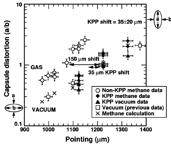
FIG. 5-24. X-ray image distortion vs laser pointing for standard capsule implosions in methane-filled hohlraums for smoothed and unsmoothed beams. LASNEX calculations and data for vacuum hohlraums are also shown. The smoothed beam data set gives a shift of 35 \mu\text{m} from the LASNEX results, while the unsmoothed data set gives a shift of 150 \mu\text{m} .
