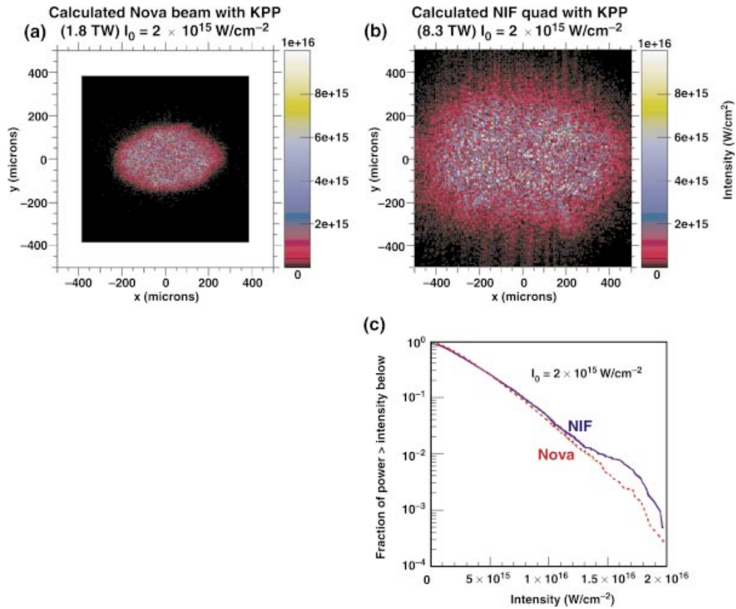
FIG. 3-14. (Color) A kinoform phase plate (KPP) is used to produce a focal spot for experiments at Nova and Omega (upper left-hand side) and NIF (upper right-hand side) with an intensity distribution (lower right-hand side) similar to that planned for NIF.
