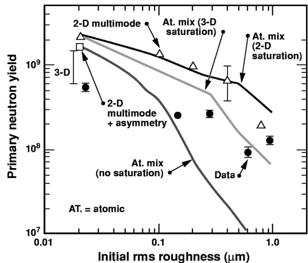
FIG. 7-16. Measured and calculated primary neutron yields for 1.3 at. % Ge-doped capsules vs initial surface roughness. Solid circles are averaged data points from Fig. 7-22. Solid curves are predictions from the atomic mix model with no saturation, with 2D saturation, and with a 3D saturation prescription. The square and the triangles are predictions from 2D multimode simulations with and without intrinsic long-wavelength hohlraum flux nonuniformities. The vertical line at the upper left-hand side represents the range of yields calculated by the 3D HYDRA code for a smooth capsule by varying the relative orientation between low-order capsule and radiation flux nonuniformities.
