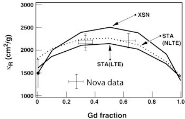
FIG. 4-8. (Color) Burnthrough measurements have shown that cocktails decrease wall losses and have a Rosseland mean opacity that depends on composition as predicted by STA models.
