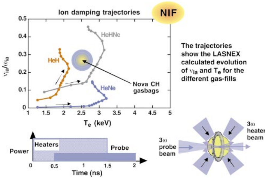
FIG. 3-28. (Color) Three mixtures of He, H, and Ne gas provided ion damping and electron temperature scaling in a NIF-like composition low-Z plasma. The dots along the curves represent 100 ps intervals in time along the 1.5 ns heater pulse [J. D. Moody et al. , “First measurement of backscatter dependence on ion acoustic damping in a low-Z, high density laser-plasma,” Phys. Plasmas (to be submitted)].
