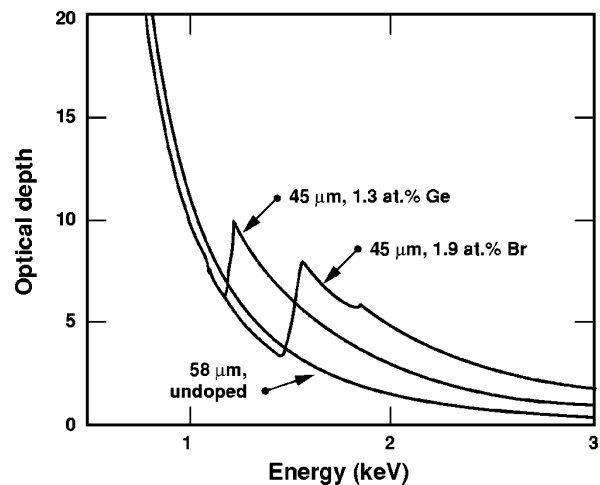
FIG. 7-10. Initial capsule ablator opacity vs photon energy for 58 \mu\text{m} thick undoped plastic ablators and for 45 \mu\text{m} thick ablators doped with either 1.3 at. % Ge or 1.9 at. % Br.
