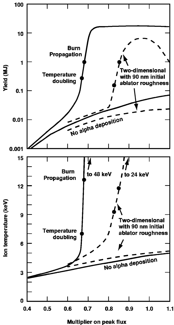
FIG. 2-5. Ignition could be diagnosed as a rapid increase in yield and neutron-width burn temperature as drive is varied. The horizontal axis is a multiplier on the peak drive, with the first 13 ns of the pulse unchanged, and the flux smoothly interpolated between 13 ns and the multiplied flux for times 14 ns and greater. Solid lines show one-dimensional simulations, and dashed lines show a heavily perturbed two-dimensional simulation. (The 90 nm initial roughness in the 2D simulations is about four times the surface roughness specification.) Temperature doubling, above what would occur without bootstrapping via \alpha deposition, occurs at a yield of a few hundred kJ, and yields above about 1 MJ require propagation of the burn into the main fuel region. The appearance of ignition as a threshold in yield and ion temperature is similar in 1D and 2D, although in 2D the capsule has less margin and lower yields.
