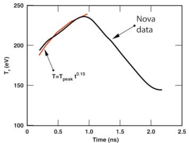
FIG. 4-4. (Color) Radiation-temperature profile obtained from soft x-ray diode measurements for a Au hohlraum driven by a 1 ns, constant-power laser pulse. The theoretical curve in red with T = T_{\text{peak}} t^{0.15} requires a conversion efficiency \eta = 0.7t^{0.12} .
