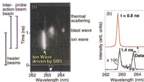
FIG. 3-42. (Color) (a) Time-resolved Thomson scattering spectrum showing coherent scattering on ion waves driven by SBS, scattering on the blast wave, and thermal incoherent scattering at late times. The time sequence of the laser beams is indicated on the left. (b) Lineouts at t = 0.8 ns and t = 1.4 ns. The earlier lineout shows 2 orders of magnitude enhanced scattering compared to the spectrum at later times. The latter is fit with the theoretical TS form factor for a gas fill CO 2 plus 1% Ar.
