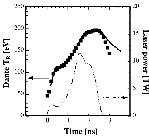
FIG. 7-31. Measured (filled squares) and simulated (solid line) Dante drive temperature vs time for the Omega high convergence implosions done in 2000–2001; laser power history (dashed–dotted) vs time.
