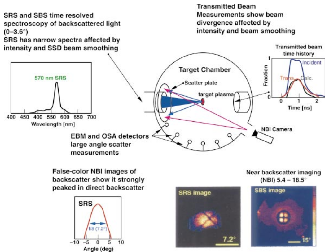
FIG. 3-11. (Color) Several diagnostics were implemented on Nova to study scattered light over a wide range of angles and frequencies. Also used but not shown on this schematic is Thomson scattering.
