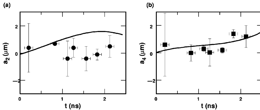
FIG. 5-32. Foam ball distortions from Omega multiple ring illumination in cylindrical hohlraums driven by PS26. (a) Foam ball second-order and (b) fourth-order Legendre distortions. Curves are code simulations of expected distortions.
