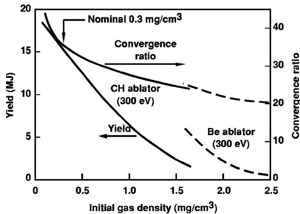
FIG. 2-14. Capsule gas fill provides direct control of convergence ratio. Increasing the initial gas fill reduces convergence ratio (and yield). However, ignition margin also decreases as gas fill increases. The higher-fill-pressure capsules are more sensitive to asymmetry and instability even though they have lower convergence.
