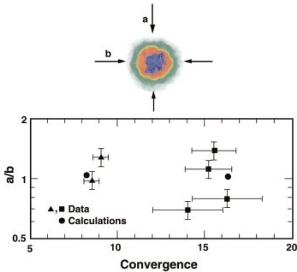
FIG. 5-27. (Color) Capsule distortion from Omega experiments using a NIF-like multiple-ring geometry with inner and outer rings well separated. The results shown are for optimal symmetry and are discussed further in Sec. VII for the HEP4-5 results.
