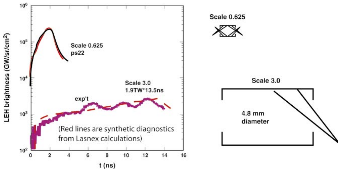
FIG. 4-15. (Color) When drive is measured through the LEH, detailed, quantitative modeling spans two orders of magnitude in radiation flux/cm 2 . The experiment is shown in black and blue. LASNEX results are in the red solid and dashed lines.
