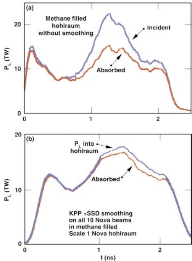
FIG. 4-12. (Color) Smooth beams are required for high absorption in gas-filled hohlraums. Similar smoothing is planned for NIF. Absorption (a) without smoothing and (b) with smoothing.
