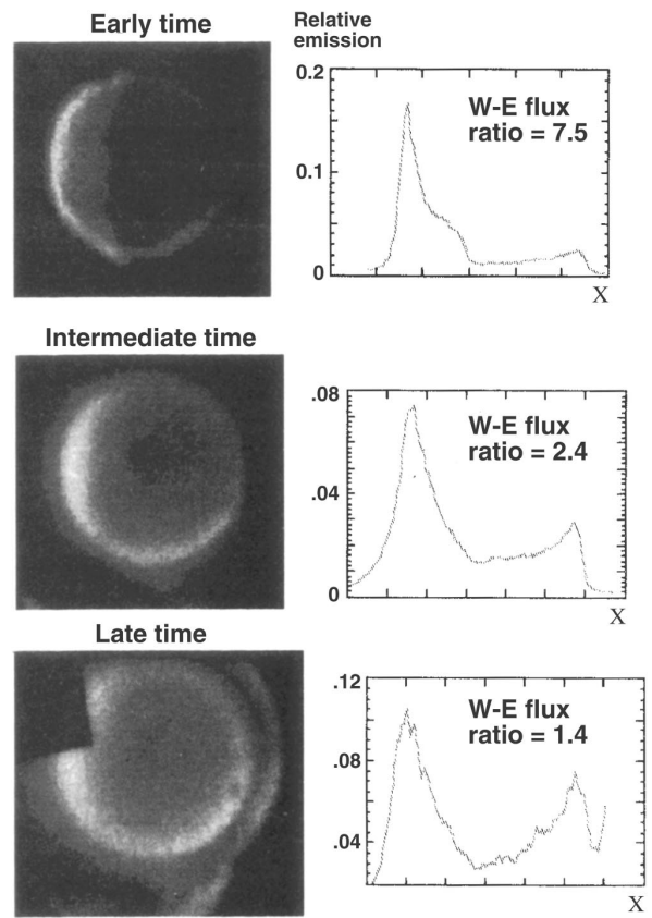
FIG. 5-10. Evolution of hohlraum environment with an intentionally imposed (east-west) laser beam imbalance of 1:2. The lineouts for each frame are taken horizontally through the center of the re-emission ball. The top frame is taken about 200 ps after the rise of a 1 ns laser drive pulse; the middle is about 400 ps after the rise and the lower about 800 ps.
