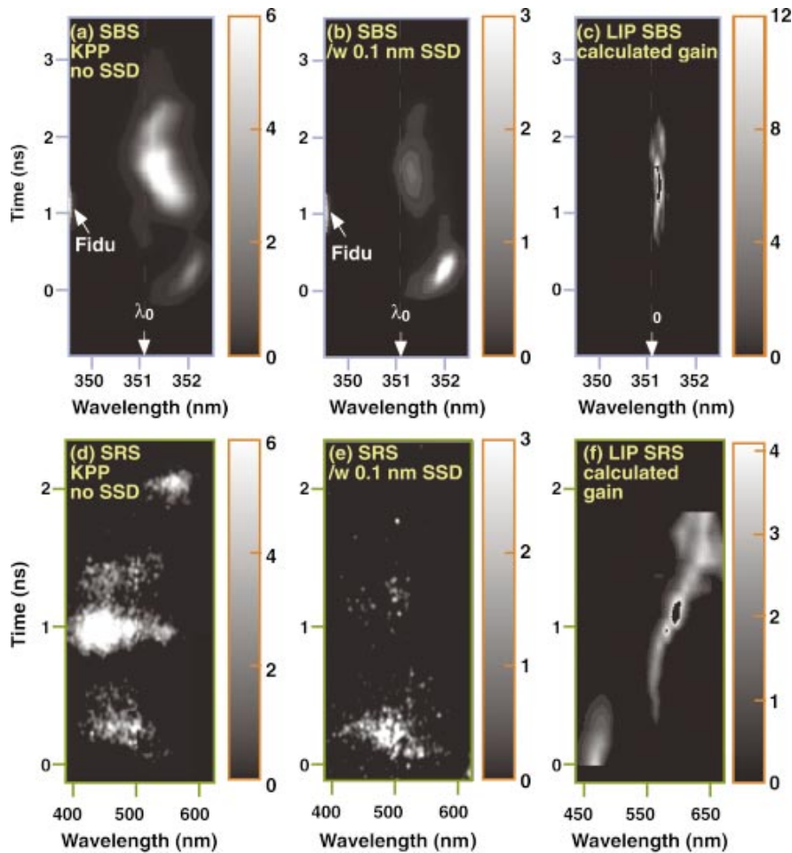
FIG. 3-36. (Color) The SBS and SRS spectrum vs time from a scale-1 Nova hohlraum without SSD (a) and (d), with SSD (b) and (e), and the calculated SBS (c) and SRS (f) gain. The SBS signal with SSD is difficult to discern but peaks at 1.5 ns and is narrower than without SSD. The spectral shift and time history agree with the SBS linear gain calculated with LIP using the mean laser intensity and LASNEX-calculated plasma parameters. The SRS spectrum is much narrower and reduced with SSD than without. It peaks at 1 ns when the calculated gain peaks. However, the SRS peaks at a shorter wavelength than the calculated gain. The late-time SRS gain arises from high-density plasma where it might be reabsorbed or inhibited by SBS competition [S. H. Glenzer et al. , Phys. Plasmas 8 , 1692 (2001)].
