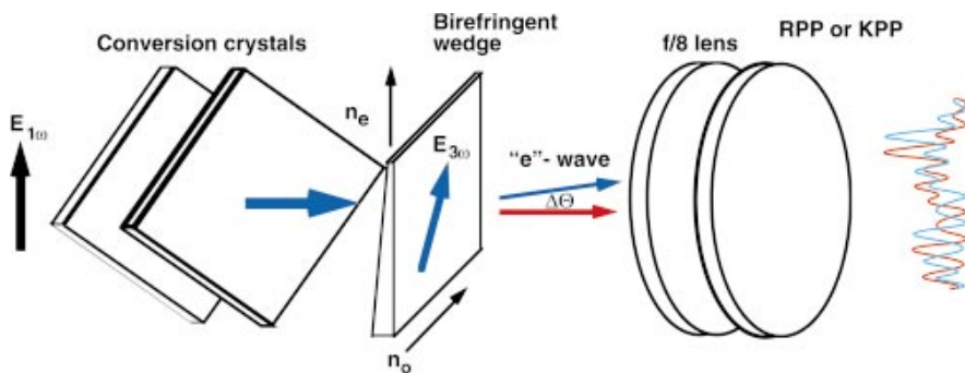
FIG. 3-15. (Color) Polarization smoothing was introduced through the use of a birefringent wedge.
