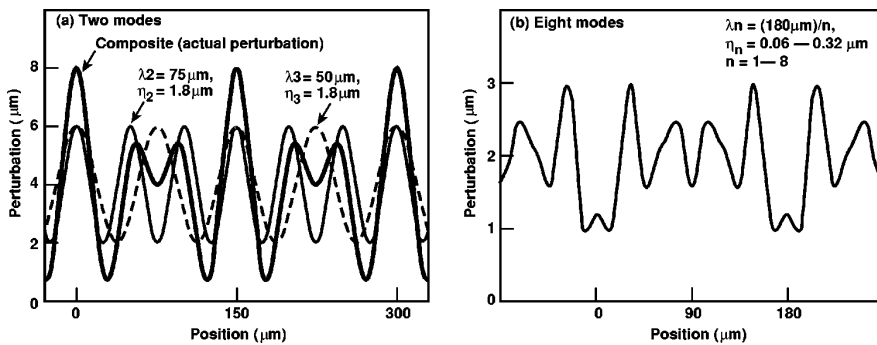
FIG. 6-11. The multimode perturbation patterns investigated are shown. (a) The curves correspond to \lambda_2 = 75 \mu\text{m} , \eta_2 = 2 \mu\text{m} (dashed), \lambda_3 = 50 \mu\text{m} , \eta_3 = 2 \mu\text{m} (dotted), and their superposition (solid), which represents the actual perturbation. (The actual measured amplitudes were \eta_{2,3} = 1.8 \mu\text{m} .) (b) The 8-mode perturbation is given by the solid curve and corresponds to the sum of wavelengths \lambda_n = (180 \mu\text{m})/n , n = 1 - 8 .
