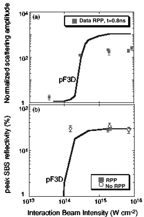
FIG. 3-43. (a) Scattering amplitude of the blueshifted ion acoustic wave normalized to the intensity of the redshifted thermal peak for various interaction beam intensities. Amplitudes are for t = 0.8 ns. (b) SBS reflectivity for no RPP data is observed to saturate at the 30% level. In both (a) and (b), the pF3D curves represent modeling.
