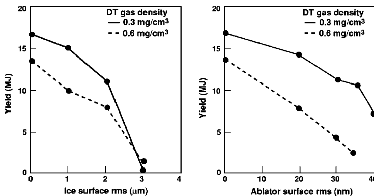
FIG. 2-15. The central gas density must be optimized in coordination with target fabrication. DT layer quality from \beta -decay is better at 0.5 K below the triple point than at 1.5 K below the triple point. However, the higher fill density of 0.6 \text{mg}/\text{cm}^3 near the triple point also increases sensitivity to ice roughness. Supplementing the \beta -decay heating with an external IR source results in improved layer smoothness at lower temperatures and lower gas vapor pressures.
