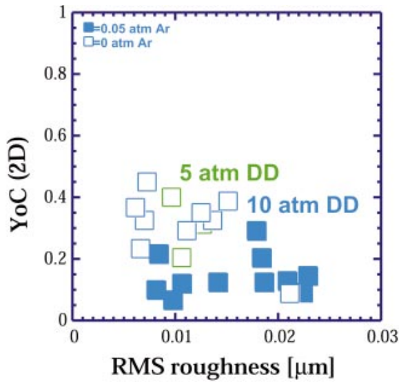
FIG. 7-30. (Color) Yield over clean (2D) DD neutron yield vs rms surface roughness for 5 atm (green) and 10 atm (blue) fill with (solid squares) and without (open squares) 0.05 atm Ar dopant for Omega HEP5 targets fielded in 2000–2001.
