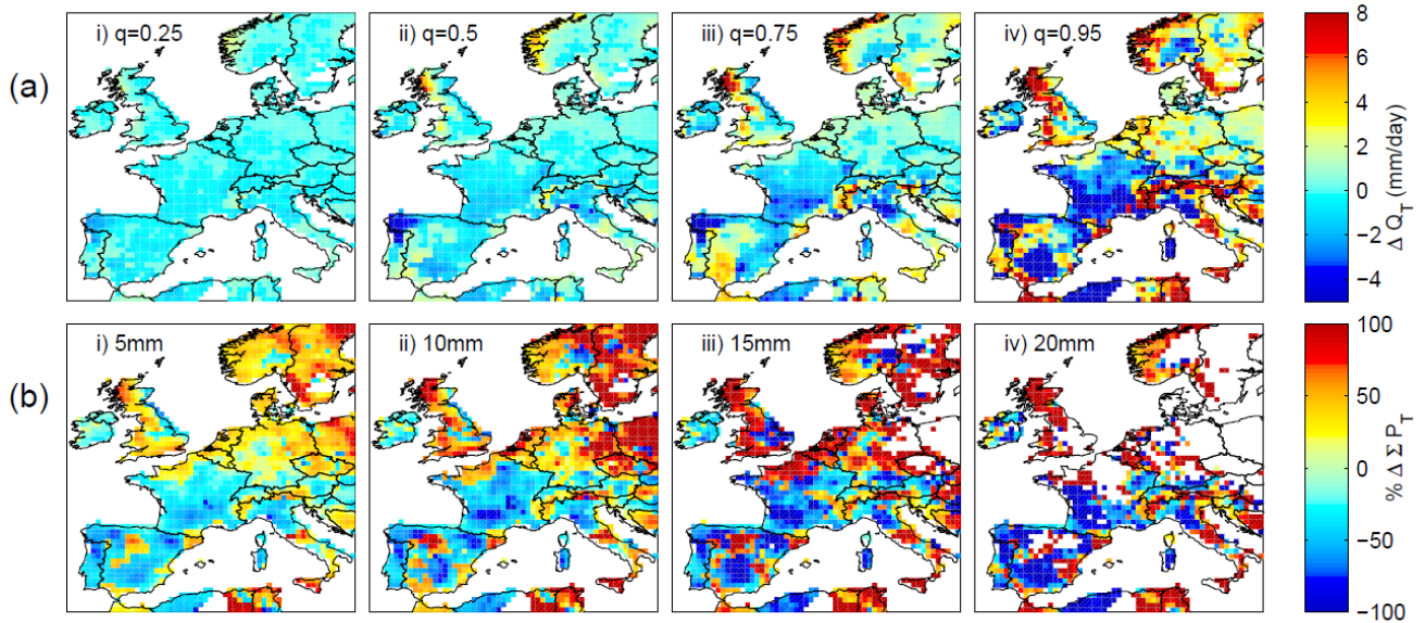
SI Figure 4: Largest non-parametric changes in European precipitation. As Figure 3 but showing the largest (see Appendix) identified changes.
