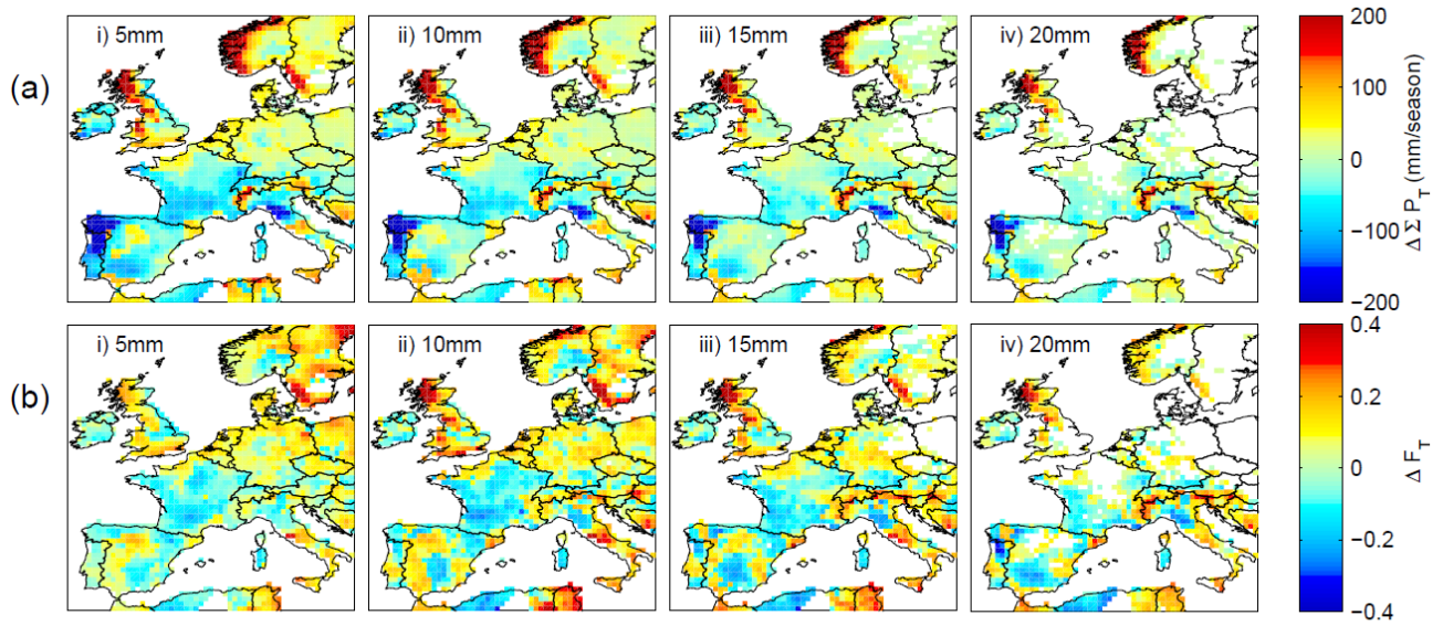
SI Figure 5: Largest non-parametric changes in European precipitation. As SI Figure 3 but showing the largest (see Appendix) identified changes.
