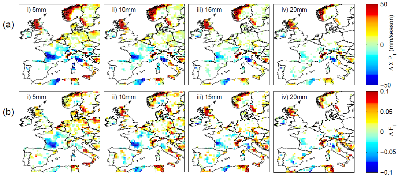
SI Figure 3: Non-parametric identifiable changes in European precipitation. As figure 3 but for the climate change descriptors (a) change in total seasonal precipitation above a threshold, \Delta\Sigma P_T and (b) change in the fraction of total seasonal precipitation that falls on days wetter than the threshold, \Delta F_T . The thresholds are 5, 10, 15 and 20 mm/day.
