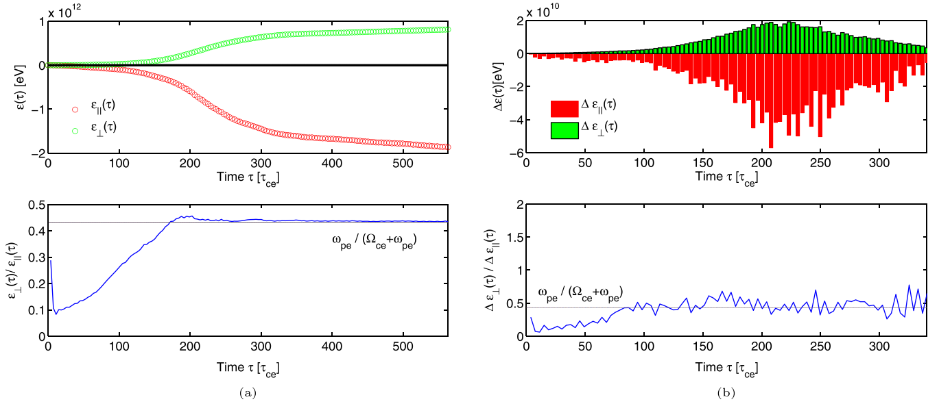
FIG. 10. Energy flow in the perpendicular and parallel directions, over time. (a) Top panel shows the history of \epsilon_{||}(\tau) (red) and \epsilon_{\perp}(\tau) (green) computed by following the trajectories of all the tail electrons throughout the simulation. Bottom panel plots the ratio |\epsilon_{\perp}(\tau)/\epsilon_{||}(\tau)| , the horizontal line marks the value \omega_{pe}/(\Omega_{ce} + \omega_{pe}) . (b) Top panel shows \Delta\epsilon_{||}(\tau, \Delta\tau) (red) and \Delta\epsilon_{\perp}(\tau, \Delta\tau) (green) at different times, where \Delta\tau is the time interval between data dumps which in this case is 3.78\tau_{ce} . Bottom panel shows the ratio |\Delta\epsilon_{\perp}/\Delta\epsilon_{||}| at each data dump, the horizontal line marks the value \omega_{pe}/(\Omega_{ce} + \omega_{pe}) . An initially flat tail distribution with \xi = 0.06 , \Omega_{ce}/\omega_{pe} = 1.31 and v_M \approx 17v_B is used.
