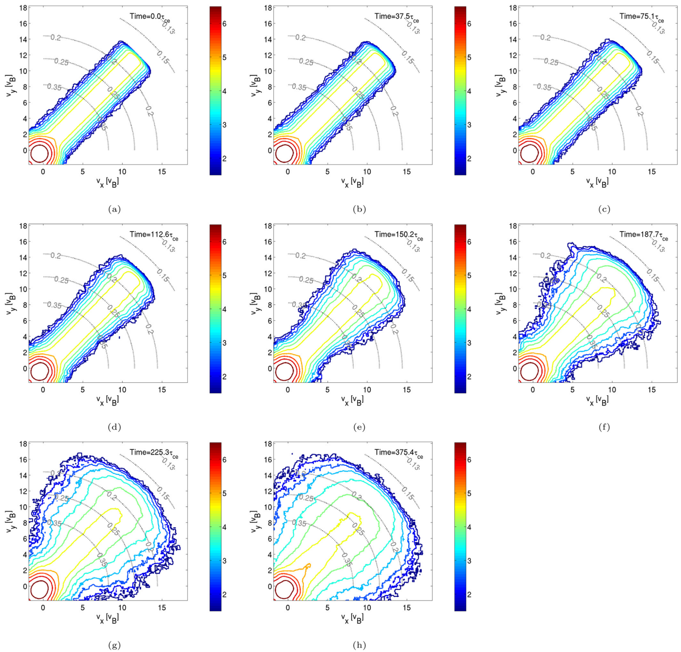
FIG. 2. Self-consistent spreading of the high energy tail of an electron distribution undergoing ADI, orientated at 45^\circ to the magnetic field direction. Constant- f contour plots of the time evolution of an electron distribution with \xi = 0.08 of the population in an initially flat tail in (v_x, v_y) phase space; velocities are in units of thermal velocity. Here \Omega_{ce}/\omega_{pe} = 1.31 , and the tail model in Eq. (6) is used, with v_M/v_B = 17 . The colour density is in logarithmic scale with overlaying dash lines that represent the constant v surfaces with normalised wavenumber kv_B/\omega_{pe} inferred from Eq. (3). Panels (a) to (h) show snapshots from initial setup, through linear instability, to the nonlinear phase of the ADI: t = (a) 0.0 \tau_{ce} , (b) 37.5 \tau_{ce} , (c) 75.1 \tau_{ce} , (d) 112.6 \tau_{ce} , (e) 150.2 \tau_{ce} , (f) 187.7 \tau_{ce} , (g) 225.3 \tau_{ce} and (h) 375.4 \tau_{ce} , where \tau_{ce} is the electron cyclotron period, \tau_{ce} = 2\pi/\Omega_{ce} . Panels (a) to (g) are separated by equal time intervals, 37.5 \tau_{ce} , where the last two panels are separated by a longer time interval, 150.1 \tau_{ce} . This is to reflect the relatively slow evolution of the electron distribution in the later stage of the simulation. Different phases of the ADI are identified from the electric field amplitude in Fig. 7, where the linear and nonlinear phases correspond to the exponential growth and saturation phases of the electric field amplitude, respectively. The electron distributions are first binned at a resolution of \Delta v \approx 0.04v_B and then smoothed using averaging over four nearest neighbours.
