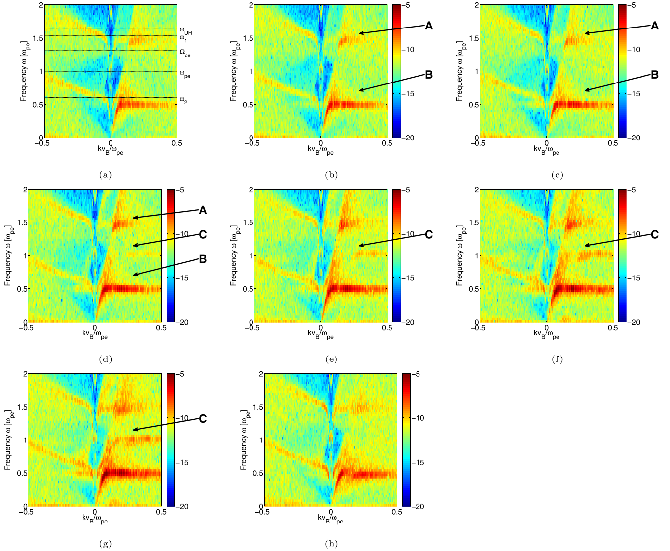
FIG. 3. Time evolution of electrostatic field amplitude, plotted as a function of \omega , k using a logarithmic scale, which is consistent with the electron distribution of Fig. 2. The frequency axis is normalised in units of \omega_{pe} and the wavenumber axis is represented in units of kv_B/\omega_{pe} . Panel (a) is constructed by short-time Fourier transforming over the time interval between panels (a) and (b) in Fig. 2, and so on successively for panels (b) to (g), while (h) corresponds to the time interval from 337.9 \tau_{ce} to 375.4 \tau_{ce} . The duration of the Fourier transform time window is the same for all panels in this figure. Panels (a) to (g) correspond to the linear phase of the ADI, see Fig. 6, whereas (h) corresponds to the nonlinear regime. In the upper left panel, the horizontal lines show natural frequencies of the plasma: from top, upper hybrid frequency, higher frequency electrostatic normal mode, electron cyclotron frequency, electron plasma frequency, lower frequency electrostatic normal mode. A, B, and C mark the dominant forward propagating modes in panels (b)-(g). The same colour scale has been adopted in each plot to assist comparison.
