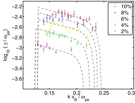
FIG. 6. Comparison between analytical expressions and the growth rates inferred from PIC simulations in their linear regime for flat tails with concentrations \xi of 2% (pink), 4% (green), 6% (yellow), 8% (blue), and 10% (red). The dashed lines represent the corresponding linear analytical growth rates computed using Eqs. (A3)–(A7). Parameters other than \xi are the same for all simulations: an initially flat tail with v_M = 5.0 \times 10^7 \text{ ms}^{-1} , \Omega_{ce}/\omega_{pe} = 1.31 .
