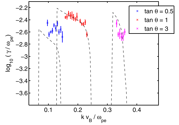
FIG. 8. Dependence of linear-stage growth rate on mode propagation angle with respect to the magnetic field. Coloured points denote linear growth rates of the most strongly growing k -modes inferred from PIC simulations for \Omega_{ce}/\omega_{pe} = 1.31 . A flat tail with \xi = 0.1 and v_M \approx 17v_B is used. Dashed lines show analytical linear growth rates for this model, calculated from Eqs. (A3)–(A7).
