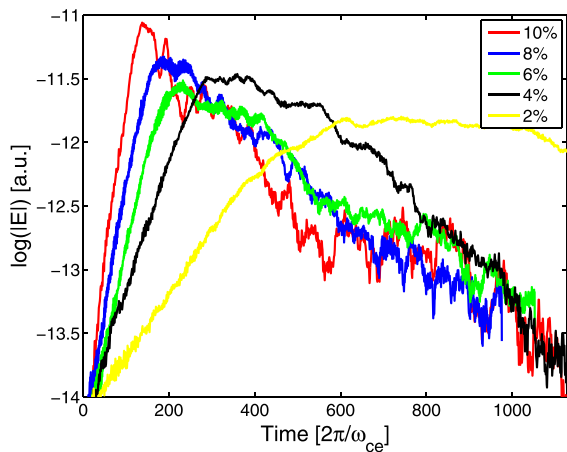
FIG. 7. Temporal evolution of electric field amplitude |\mathbf{E}_k(t)| of a specific wave-number mode kv_B/\omega_{pe} = 0.20 , for different flat tail concentrations \xi spanning 2% to 10%. The traces of |\mathbf{E}_k(t)| are shifted in time such that |\mathbf{E}_k(t)| for different tail concentrations starts at the same time zero.
