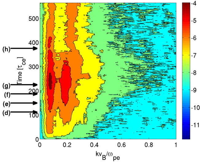
FIG. 4. Growth of dominant modes in k -space. Contour plot showing the temporal evolution of the dominant electrostatic component of electric field amplitude in (k, t) space, identified from Fig. 3, in logarithmic scale. (d)–(h) label the corresponding times of panels (d)–(h) in Fig. 2. The signal |\mathbf{E}(k, t)| is smoothed by averaging over four nearest neighbours.
