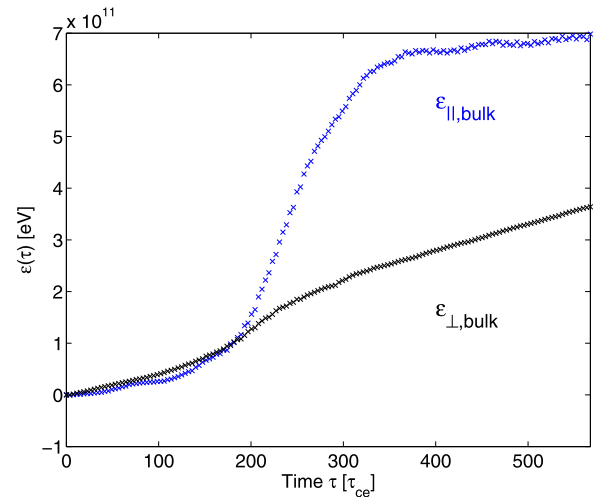
FIG. 9. History of \epsilon_{\parallel} (blue) and \epsilon_{\perp} (black) for bulk electron population, computed by following the trajectories of all the bulk electrons throughout the simulation for a flat tail distribution with \xi = 0.06 , \Omega_{ce}/\omega_{pe} = 1.31 and v_M \approx 17v_B . Both components of \mathbf{j} \cdot \mathbf{E} are positive throughout the simulation.
