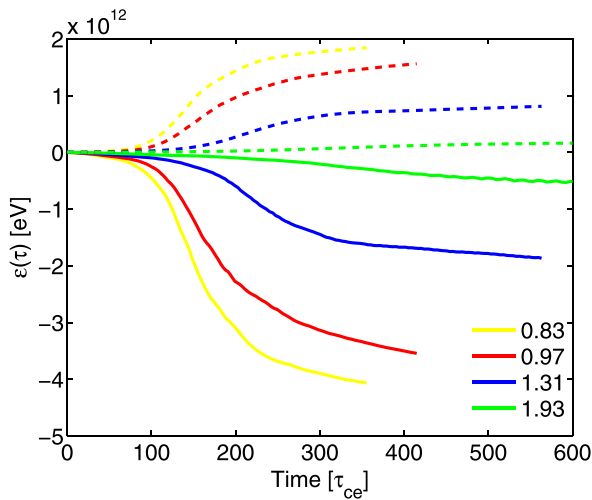
FIG. 11. Time evolution of perpendicular and parallel components of \mathbf{j} \cdot \mathbf{E} of the tail electrons, for different values of \Omega_{ce}/\omega_{pe} . The history of \epsilon_{||}(\tau) (solid lines) and \epsilon_{\perp}(\tau) (dotted lines) is computed by following the trajectories of all the tail electrons throughout the simulation for a flat tail distribution with \xi = 0.08 , for four different \Omega_{ce}/\omega_{pe} ratios: 0.83 (yellow), 0.97 (red), 1.31 (blue), and 1.93 (green).
