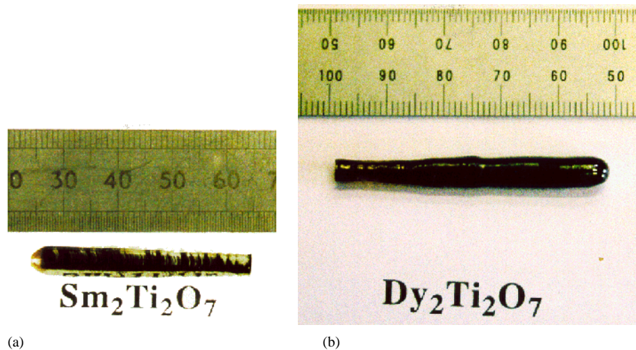
Figure 1. Single crystal of (a) Sm_2Ti_2O_7 and (b) Dy_2Ti_2O_7 grown by the floating zone method, in air, at 6 mm h -1 .
