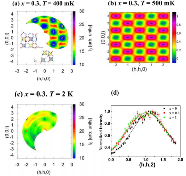
FIG. 3. (Color online) (a) NSF scattering for x=0.3 at 400 mK. The inset shows one of the possible antiferromagnetic configurations ( x-y plane projection and in three dimensions, +/- indicates that the moment is along +z/-z direction) predicted by Ref. 16; (b) MC simulation results using the DSM for x=0.3 at 500 mK; (c) NSF scattering for x=0.3 at 2 K; the low-temperature (400 mK) pattern is not observed at this temperature; (d) cuts along (h,h,2) for different doping levels at low temperature (for x=0, 1, T=30 mK and x=0.3, T=400 mK). The lines are Lorentzian fits.
