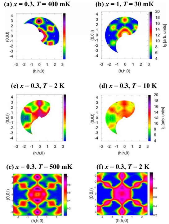
FIG. 1. (Color online) Experimental neutron SF scattering patterns for the \text{Ho}_{2-x}\text{Y}_x\text{Ti}_2\text{O}_7 compounds for (a) x=0.3 at 400 mK, (b) x=1.0 at 30 mK, (c) x=0.3 at 2 K, and (d) x=0.3 at 10 K; MC simulations made using the DSM for (e) x=0.3 at 500 mK and (f) x=0.3 at 2 K.
