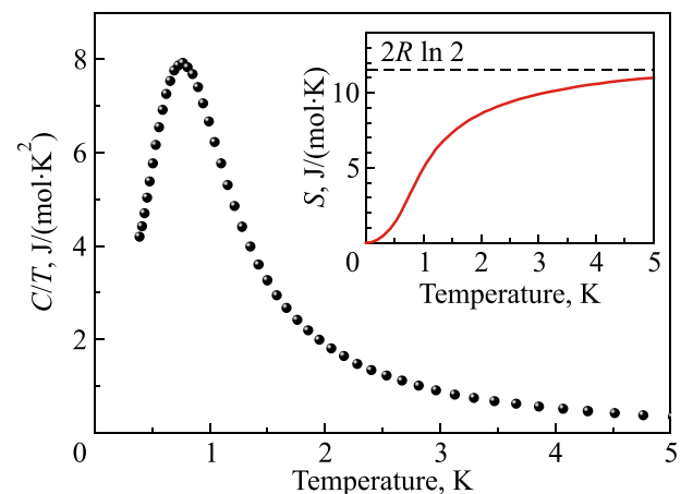
FIG. 5. Temperature dependence of the specific heat divided by temperature of \text{SrDy}_2\text{O}_4 in zero field. The inset shows the temperature dependence of the entropy, S (solid line), calculated as the area under the C(T)/T curve which has been extended linearly down to T = 0 \text{ K} . The dashed line indicates the position of 2R \ln 2 , which corresponds to the magnetic contribution for a system with an effective s = 1/2 . Figure is from Ref. 22.
