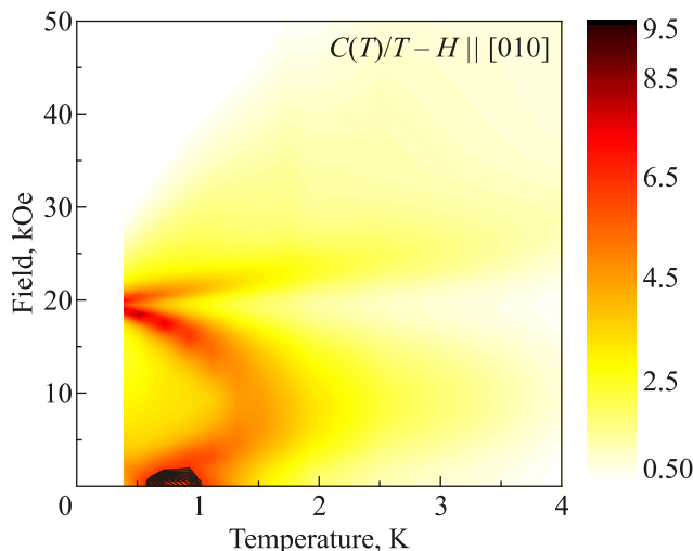
FIG. 7. Magnetic H - T phase diagram of \text{SrDy}_2\text{O}_4 for H \parallel [010] obtained from the heat capacity measurements. Color represents the heat capacity divided by temperature in the units of \text{J}/(\text{mol K}^2) . Figure is from Ref. 22.
