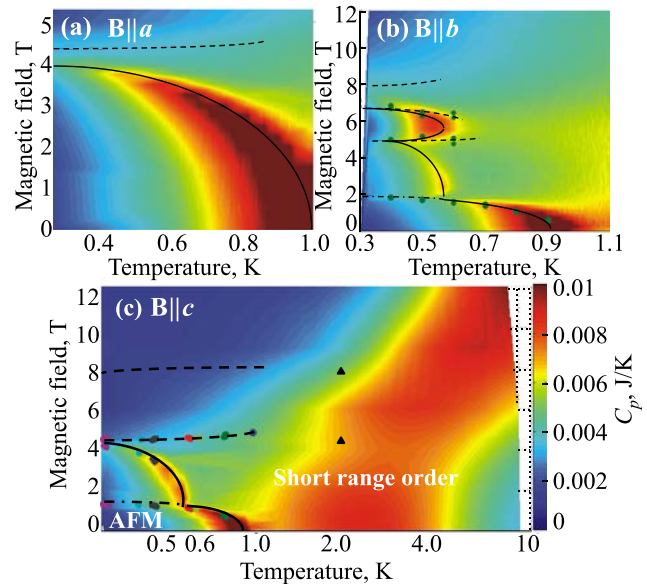
FIG. 9. Magnetic phase diagram of \text{SrYb}_2\text{O}_4 with magnetic field along a (a), b (b), and c (c) axes. The colors indicate the heat capacity in units of \text{J}/\text{K} . The circles indicate the critical fields extracted from magnetocaloric effect measurements and the triangles the critical fields extracted from magnetization measurements. Black solid lines show second-order phase transitions. Dash-dot black lines indicate the transition from the AFM phase to a less ordered one. Dashed black lines show metamagnetic crossovers. For the phase diagram along the c axis, above 4.5 T there are just three heat capacity scans at 6, 9, and 12 T, the colors between them result from the interpolation of the data. Below 4.5 T, the data were collected every 0.2 T. The temperature axis is in logarithmic scale. Figure is from Ref. 12.
