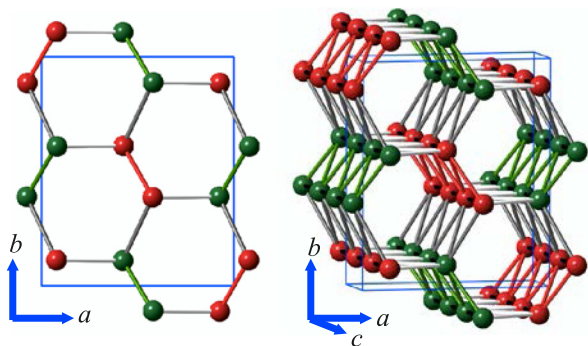
FIG. 1. Positions of the magnetic rare-earth \text{Ln}^{3+} ions within the \text{SrLn}_2\text{O}_4 compounds, with the two crystallographically inequivalent \text{Ln}^{3+} sites shown in different colors. The left-hand panel emphasizes the honeycomb arrangement of the \text{Ln}^{3+} ions when viewed along the c axis, while the right-hand panel demonstrates the formation of zigzag ladders running along the c axis which link the honeycomb layers and give rise to geometric frustration. The blue box represents a crystal unit cell of the Pnam space group.
