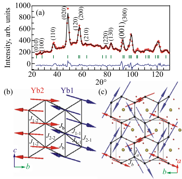
FIG. 8. (a) Magnetic powder pattern of \text{SrYb}_2\text{O}_4 collected on D7 at 30 mK. The magnetic structure where the arrows represent the \text{Yb}^{3+} ions spins (Yb1 blue, Yb2 red) (b) along the zigzag chains and (c) projected onto the ab plane. The \text{Sr}^{2+} and \text{O}^{2-} ions are represented by yellow and red circles, respectively. Figure is from Ref. 12.
