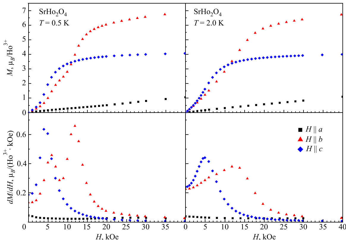
FIG. 6. Field-dependent magnetization curves (top panels) for SrHo 2 O 4 obtained at 0.5 K (left) and 2.0 K (right) in the range of fields 0 to 40 kOe. (Bottom panels) The field derivatives of the magnetization at 0.5 K (left) and 2.0 K (right). Figure is from Ref. 23.
