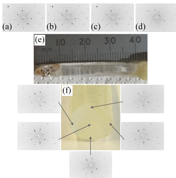
Figure 5. (a–d) X-ray Laue back reflection photographs of one of the facets of a \text{La}_2\text{Zr}_2\text{O}_7 crystal, taken along the crystal length at ~12 mm intervals, between the end (left) and the beginning (right) of the boule. The corresponding Laue patterns taken on the facet at 180 degrees are mirror images of these patterns; (e) Boule of \text{La}_2\text{Zr}_2\text{O}_7 prepared by the floating zone method in air at a growth rate of 15 mm/h; (f) Laue patterns taken of the cross section of the boule at ~15 mm from the beginning of the boule, are consistent with one another at several points covering the entire surface. Five patterns corresponding to scans across the diameter of the boule, taken at ~2 mm intervals, are shown.
