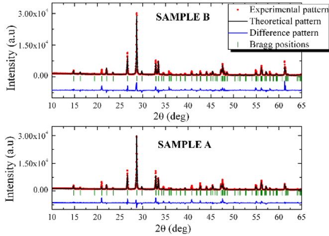
Fig. 3. Simulated diffraction pattern of \text{Ba}_2\text{CuGe}_2\text{O}_7 against experimental XRD data of SAMPLES B (top) and A (bottom).
