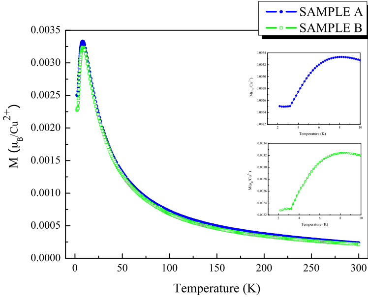
Fig. 6. Magnetization versus temperature of \text{Ba}_2\text{CuGe}_2\text{O}_7 single crystals for a field \mu_0 H = 0.1 \text{ T} applied parallel to the [101] direction.
