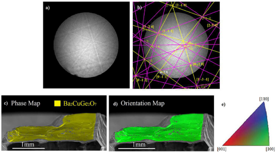
Fig. 4. (a) and (b) Experimental EBSD pattern and indexed pattern. (c) Phase map on the SEM image of a single \text{Ba}_2\text{CuGe}_2\text{O}_7 crystal grown in oxygen (SAMPLE B). The results show that there is only \text{Ba}_2\text{CuGe}_2\text{O}_7 phase on analyzed surface. (d) Map of normal orientation to the crystal surface. The sample is oriented with [100] direction orthogonal. (e) Color key of the orientation map.
