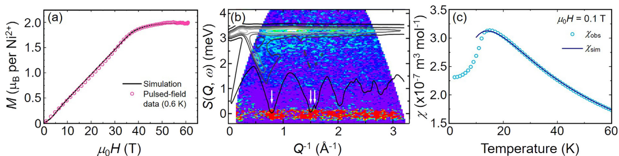
Fig. 2. (a) M(H) and (b) INS data for powder samples of 1 . The simulated traces in (a) and (b) coincide with D = 13.3(1) K, J = 10.4(3) K and J' = 1.4(2) K as described in the text. White arrows in (b) indicate magnetic Bragg peaks arising from the 3D XY-ordered magnetic ground-state. (c) Experimental \chi(T) along with the theoretical curve obtained for D = 11.8 K, J = 10.7 K and J' = 0 . See ref. [33] for details.
