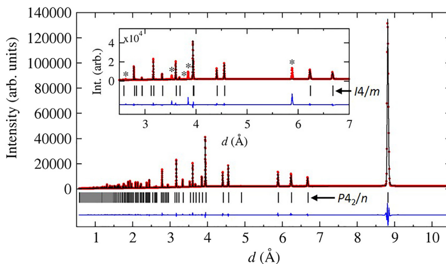
Fig. 9. T = 100 K X-ray powder diffraction data (●) for an as-precipitated sample of 4a comparing Rietveld refinements (—) in space groups P4_2/n (main) and I4/m (inset). Asterisks in the inset plot mark additional peaks, (1 1 1), (2 2 1), (3 1 1), (2 1 2) and (4 2 1) expected for P4_2/n . Difference plots ( I_{\text{obs}} - I_{\text{calc}} ) are shown as blue lines at the bottom. (For interpretation of the references to colour in this figure legend, the reader is referred to the web version of this article.)
