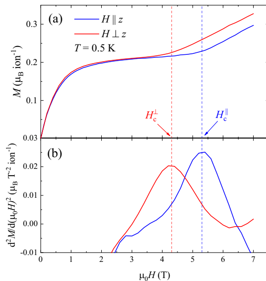
FIG. 3. (a) Single-crystal magnetization measurements performed with magnetic fields parallel ( \parallel ) and perpendicular ( \perp ) to the unique local axis in \text{NiI}_2(3,5\text{-lut})_4 , which coincides with the chain direction. (b) The second derivative of magnetization with respect to field yields the anisotropic critical fields.
