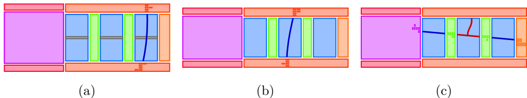
Figure 8.8: t_0 candidates in x (Figure 8.8a), y (Figure 8.8b) and z (Figure 8.8c). The red pattern shown in Figure 8.8c is not a candidate since it is not a unique single track pattern.
