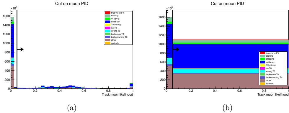
Figure 7.1: Muon PID cut in selection showing cut value and distribution of signal and background muon likelihood (Figure 7.1a) and the same distribution with binning to better illustrate signal survival (Figure 7.1b).
