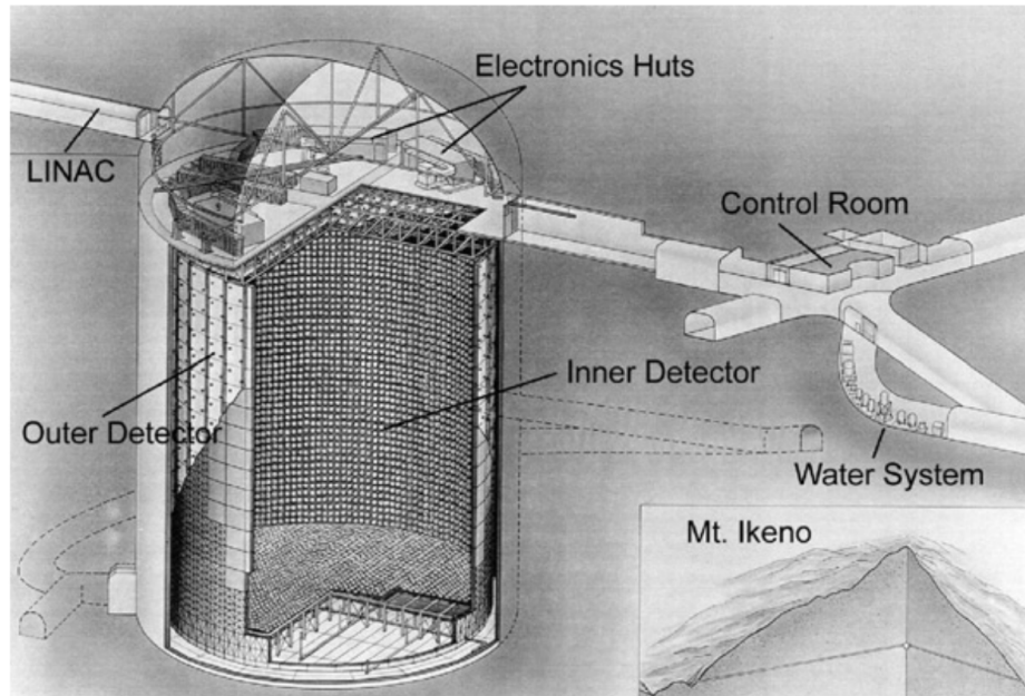
Figure 4.6: The Super-Kamiokande detector, showing the huge volume of the water Čerenkov inner detector, from[151]
