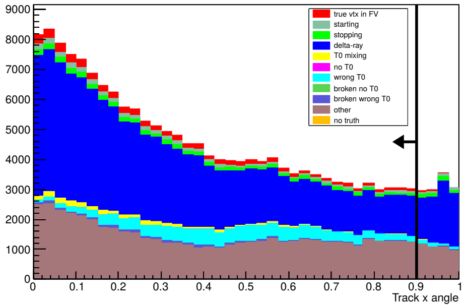
Figure 7.4: x -angle cut in selection showing cut values.
