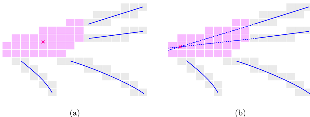
Figure 7.5: Projected vertex position calculation, with tracks illustrated by blue lines and vertex position by a pink star. Default vertex position is shown in Figure 7.5a and projected position is shown in Figure 7.5b.
