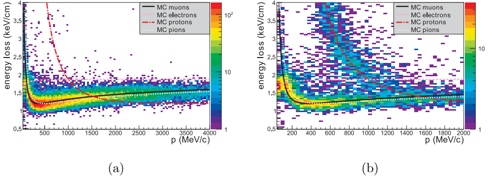
Figure 6.23: Illustration of \frac{dE}{dx} for negatively charged (Figure 6.23a) and positively charged (Figure 6.23b) particles produced by neutrino interactions in the ND280 beam, from [158].
