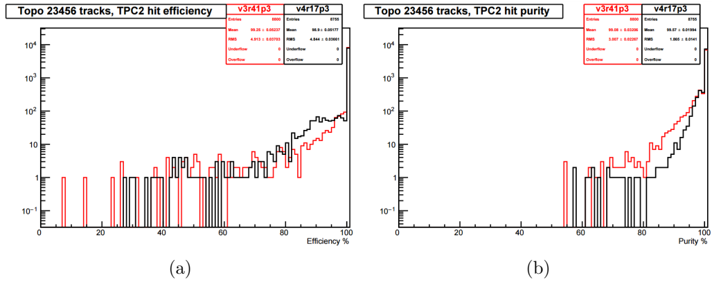
Figure 6.26: Illustration of TREx efficiency (Figure 6.26a) and purity (Figure 6.26b) compared to old TPC reconstruction on beam Monte Carlo. Efficiency for the old reconstruction version (v3r41p3) is in red while TREx software version used for analysis (v4r17p3) is in black.
