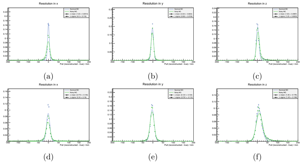
Figure 8.6: Vertex resolution systematic uncertainties for two- (Figure 8.6a, Figure 8.6b, Figure 8.6c) and multi-track (Figure 8.6d, Figure 8.6e, Figure 8.6f) events in the x , y and z directions.
