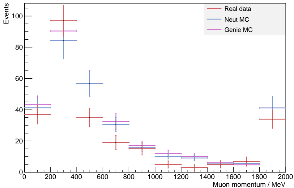
Figure 9.2: Selected muon momentum in real data and Monte Carlo.
