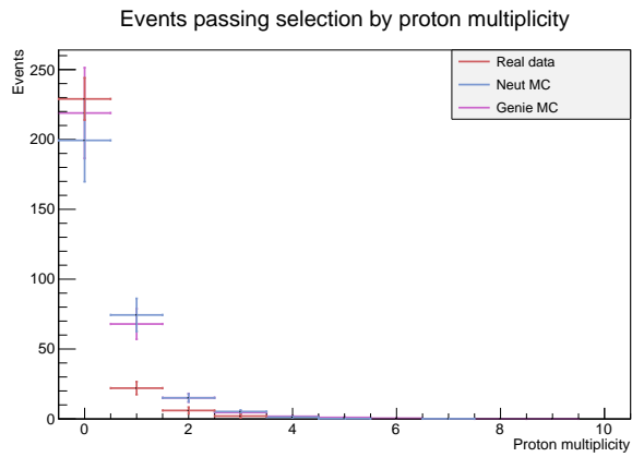
Figure 9.5: Selected vertex multiplicity, counting paths of 100 MeV or more which also have proton PID, in real data and Monte Carlo.
