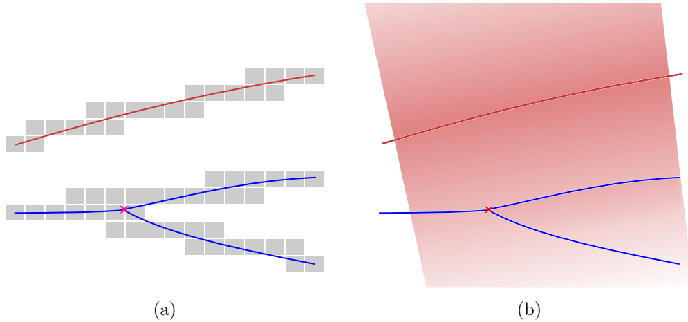
Figure 7.7: Illustration of passing by tracks in the selection. Figure 7.7a shows a phantom vertex candidate produced by two collinear tracks, with the misreconstructed tracks attached to the junction shown in blue and another passing by track in red. Figure 7.7b shows the area excluded for being alongside the second track.
