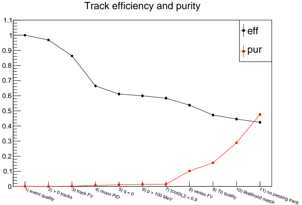
Figure 7.8: Efficiency and purity of selection cuts.
