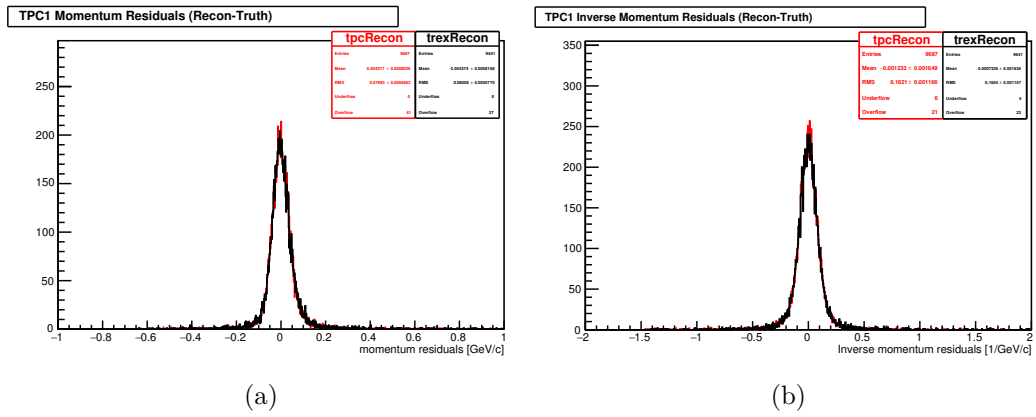
Figure 6.29: Momentum residual distributions for old reconstruction and TREx covering both momentum Figure 6.29a and inverse momentum Figure 6.29b.
