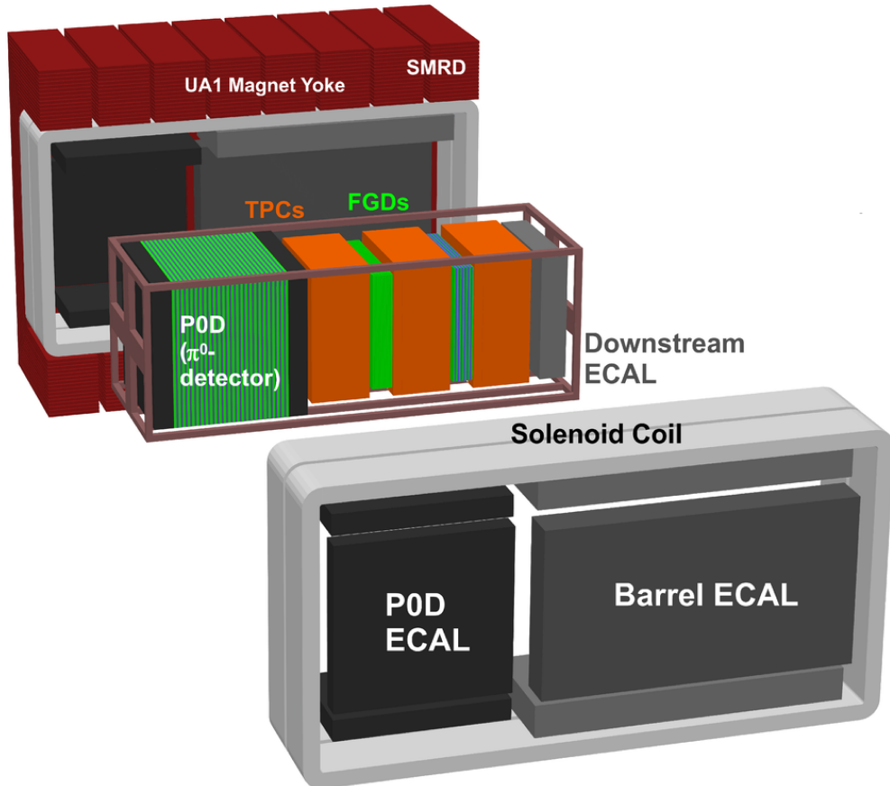
Figure 4.9: The ND280 off-axis near detector.
