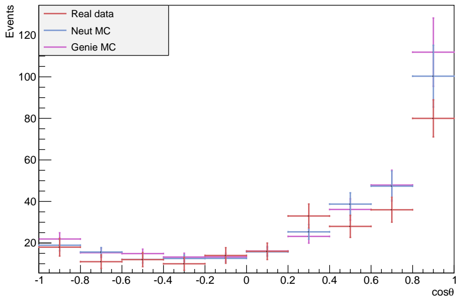
Figure 9.3: Selected muon angle relative to the beam axis in real data and Monte Carlo.
