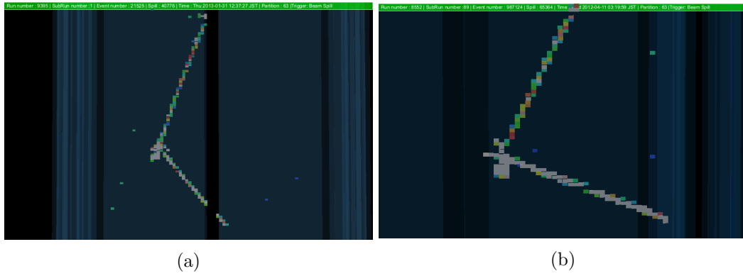
Figure 9.23: Hand scan signal events with high vertex activity. Figure 9.23a was counted as having one secondary particle and Figure 9.23b as two.
