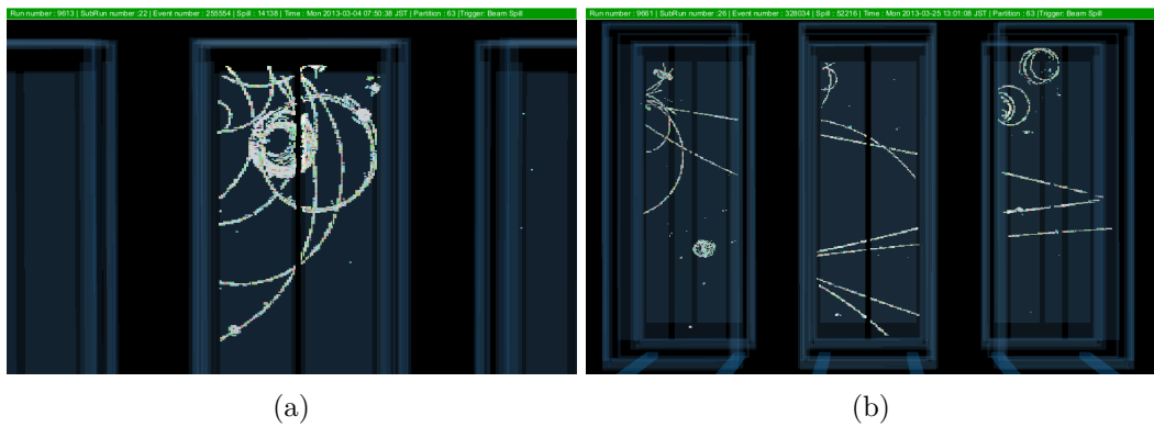
Figure 9.14: Hand scan background events with messy out of fiducial volume interactions.
