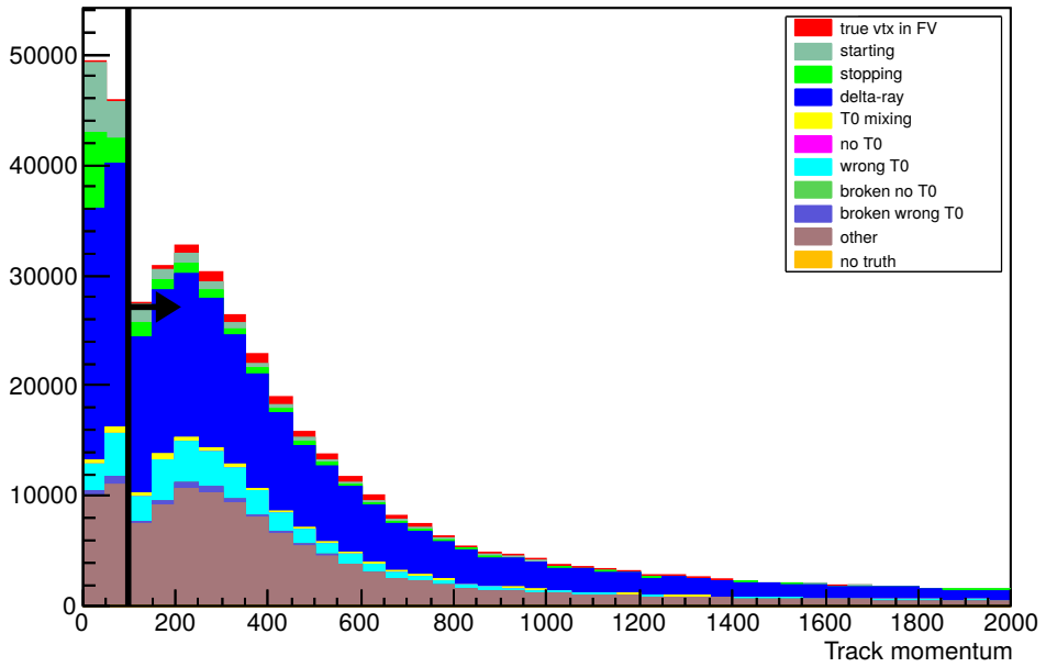
Figure 7.3: Momentum cut in selection showing cut values.
