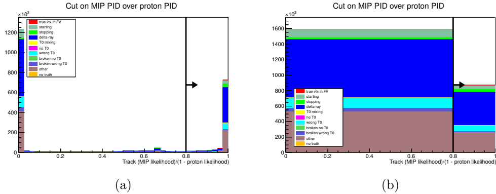
Figure 7.2: MIP PID cut in selection showing cut value and distribution of signal and background MIP likelihood values (Figure 7.2a) and the same distribution with binning to better illustrate signal survival (Figure 7.2b).
