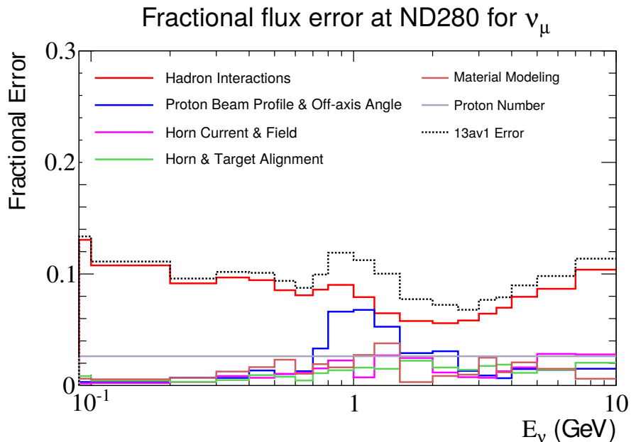
Figure 8.2: T2K fractional flux uncertainties for \nu_\mu [184]. 13av1 is the flux tuning used for this analysis — its total fractional uncertainty is shown by the dashed line.
