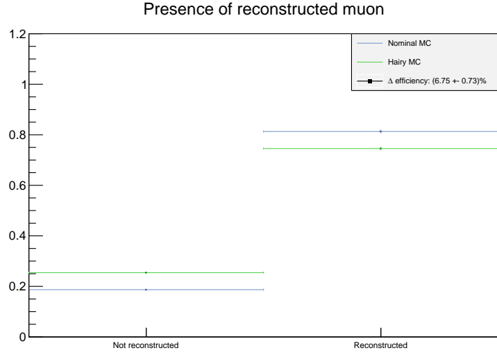
Figure 8.12: Hairy track muon efficiency for nominal and hairy Monte Carlo, with the resulting systematic shown.
