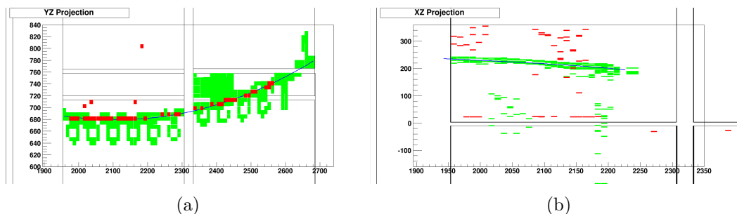
Figure 8.10: Two hairy events; a ‘chainsaw’ event (Figure 8.10a) and a ‘low charge shadow’ event (Figure 8.10b). In each case green and red blocks represent used and unused hits respectively and blue lines represent reconstructed tracks (the single blue line in Figure 8.10a is partially obscured by unused hits).
