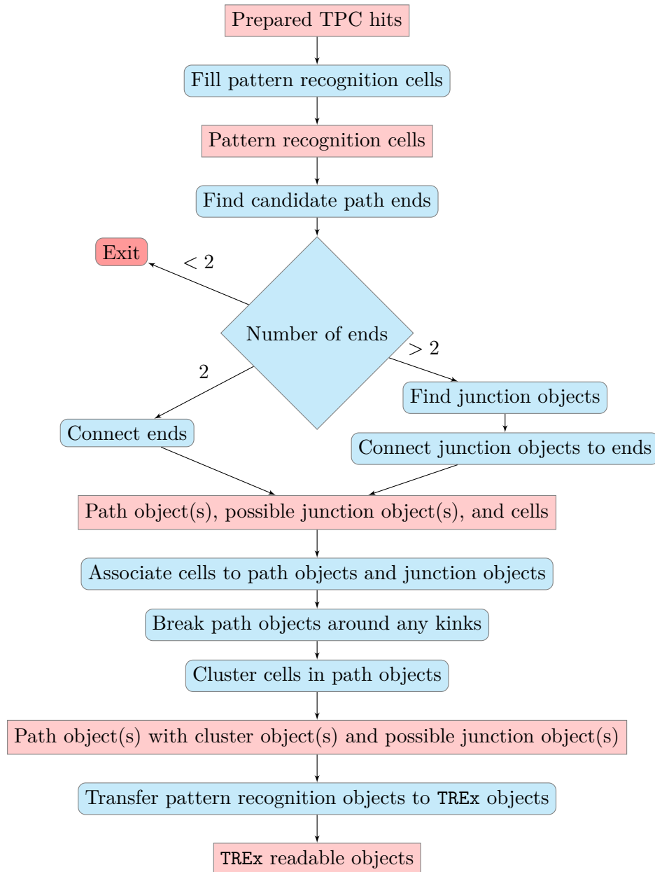
Figure 6.3: Overview of the main TREx pattern recognition steps. A number of more minor intermediate steps have been skipped for the purpose of this illustration.
