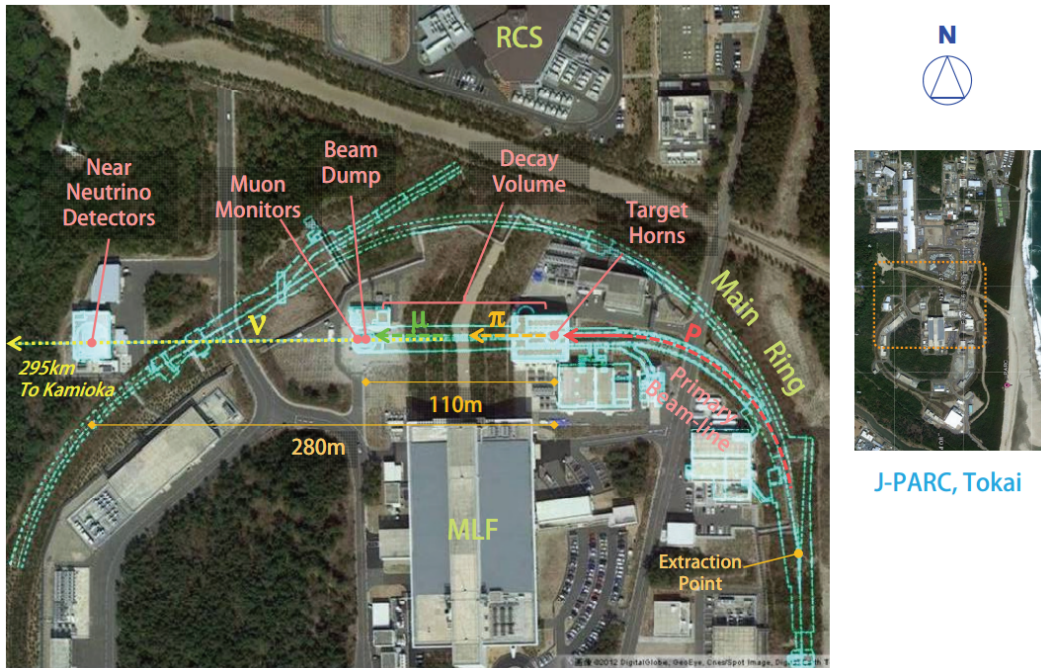
Figure 4.5: The geographical location of the J-PARC neutrino beam production facility used by T2K relative to the main ring, from [124].
