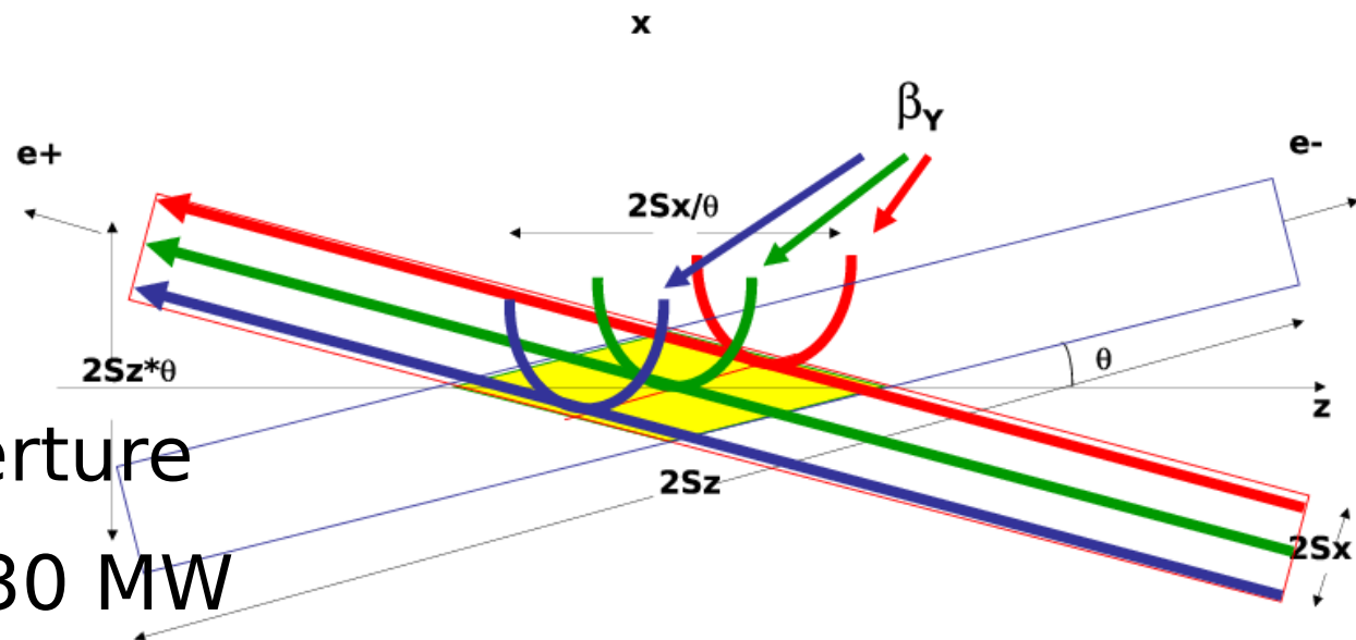
Crabbed waist scheme
