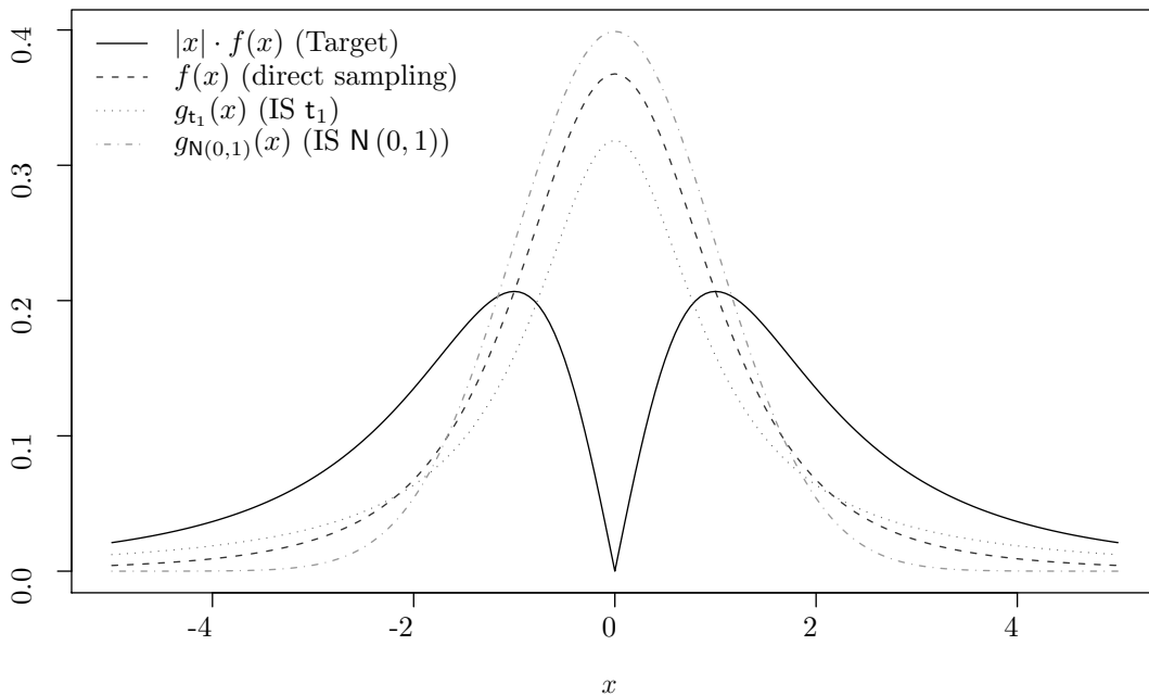
Fig. 2.4. Illustration of the different instrumental distributions in Example 2.5.
