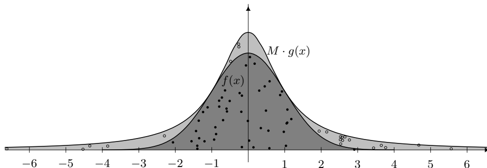
Fig. 2.3. Illustration of example 2.3. Sampling from the area under the density f(x) (dark grey) corresponds to sampling from the \mathcal{N}(0, 1) density. The proposal g(x) is a Cauchy (0, 1) .
