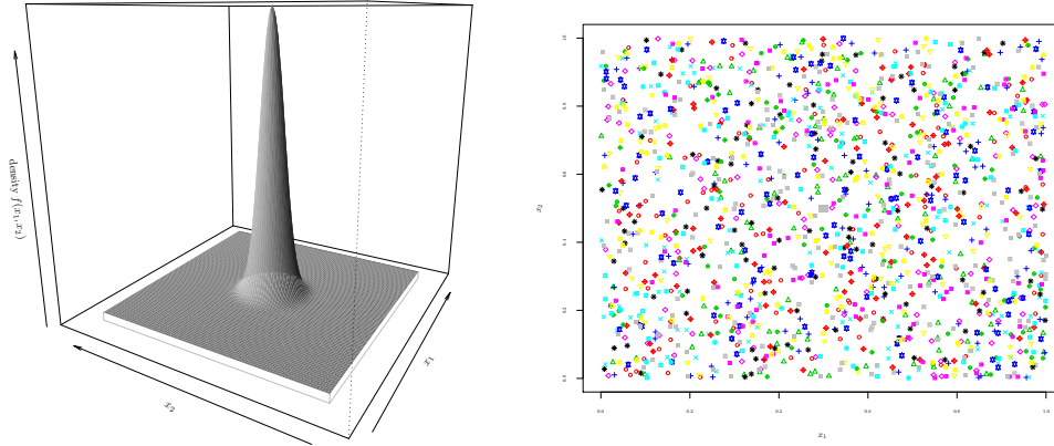
(b) First 100 values from 15 samples using different starting values. ( \delta = 10^{-3} , \mu = (0.5, 0.5)' , and \sigma = 10^{-5} )
