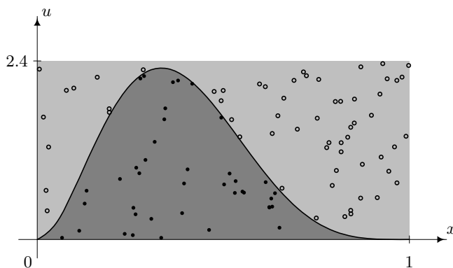
Fig. 2.2. Illustration of example 2.3. Sampling from the area under the curve (dark grey) corresponds to sampling from the Beta(3, 5) density. In Example 2.3 we use a uniform distribution over the light grey rectangle as as proposal distribution. Empty circles denote rejected values, filled circles denote accepted values.
