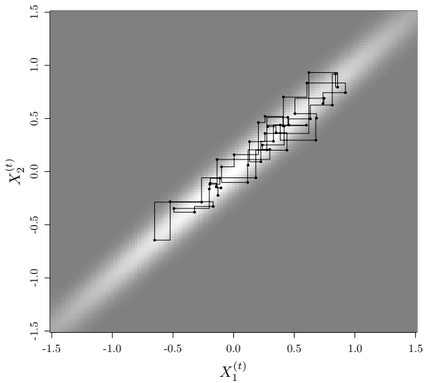
(a) First 50 iterations of (X_1^{(t)}, X_2^{(t)})
