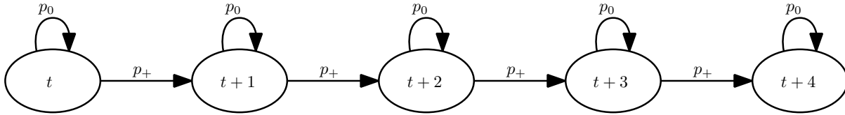
Fig. A.4. A random walk on the positive integers.
