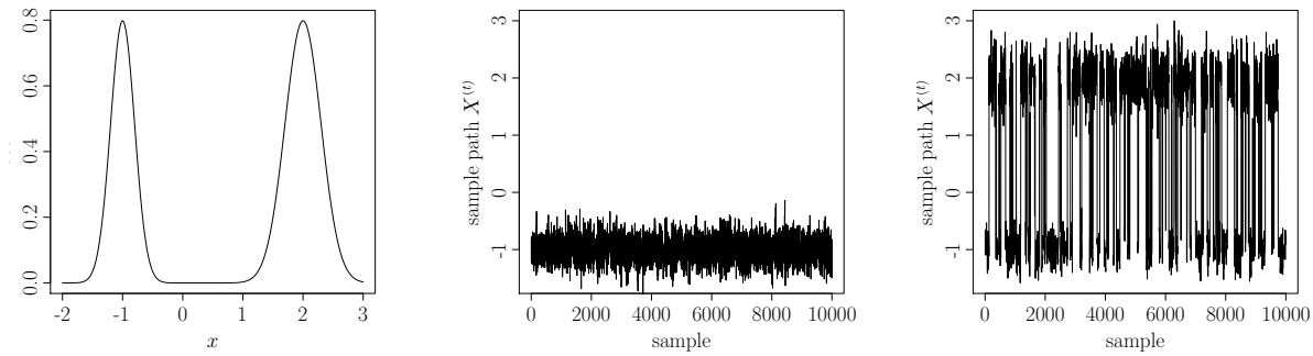
(a) Density f(x) (b) Sample path of a random walk Metropolis algorithm with proposal variance \text{Var}[\varepsilon] = 0.4^2 (c) Sample path of a random walk Metropolis algorithm with proposal variance \text{Var}[\varepsilon] = 1.2^2
