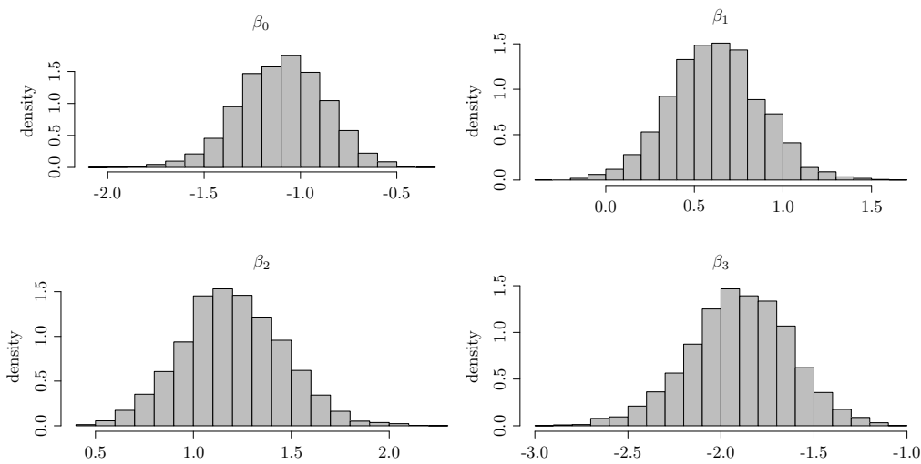
(c) Posterior distributions of the \beta_j
