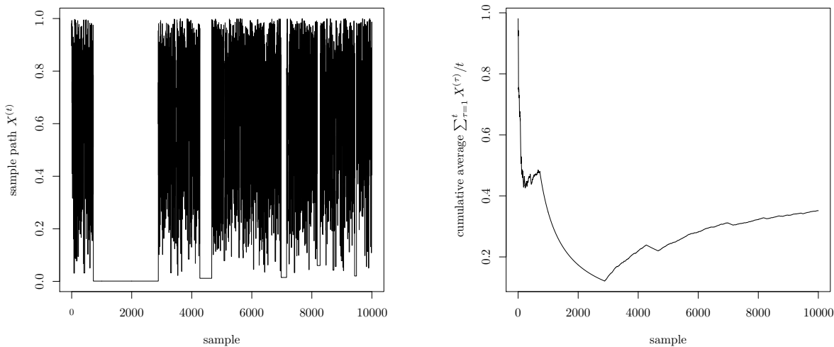
(a) Sample path X^{(t)} (b) Cumulative means \sum_{\tau=1}^t X^{(\tau)}/t
