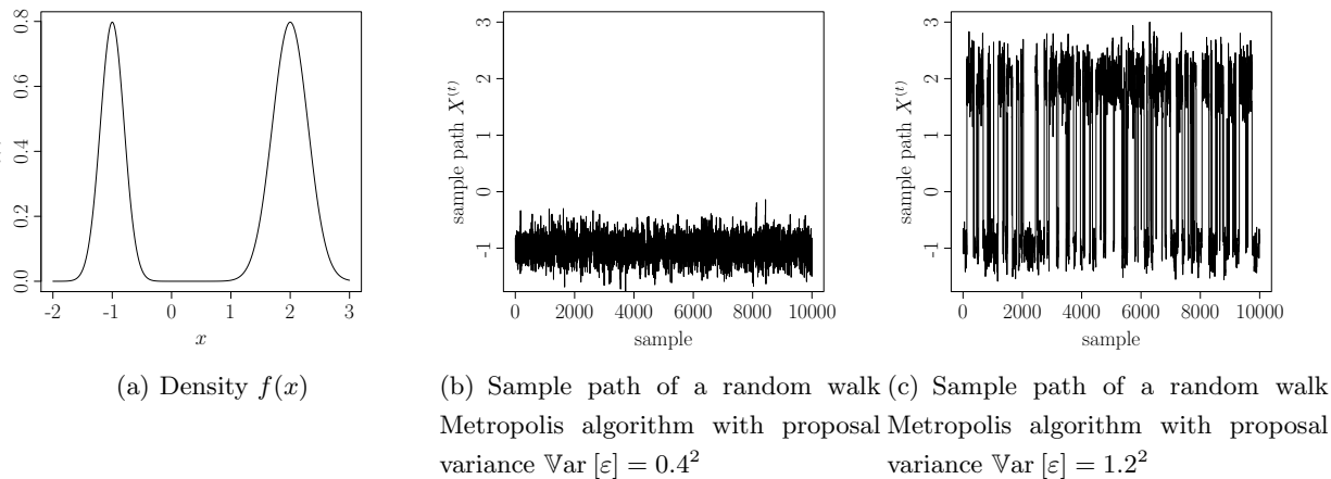
Fig. 3.11. Density of the mixture distribution with two random walk Metropolis samples using two different variances \text{Var}[\varepsilon] of the proposal.
