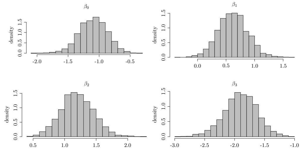
(c) Posterior distributions of the \beta_j
