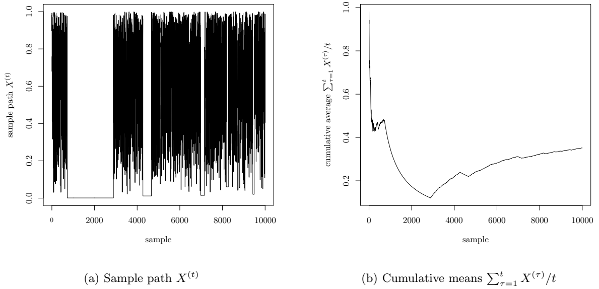
Fig. 3.12. Sample paths and cumulative means obtained for the pathological Beta generator.
