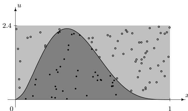
Fig. 2.2. Illustration of Example 2.3. Sampling from the area under the curve (dark grey) corresponds to sampling from the \text{Beta}(3, 5) density. In Example 2.3 we use a uniform distribution over the light grey rectangle as as proposal distribution. Empty circles denote rejected values, filled circles denote accepted values.
