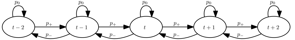
Fig. A.2. A random walk on \mathbb{Z} with K_{tt} > 0 .
