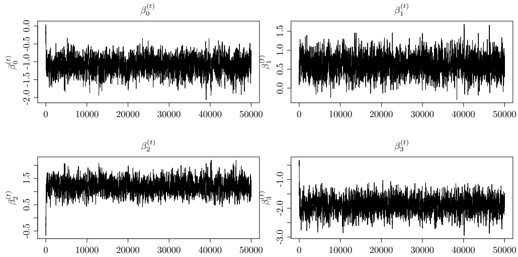
(a) Sample paths of the \beta_j^{(t)}
