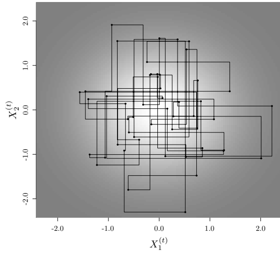
(a) First 50 iterations of (X_1^{(t)}, X_2^{(t)})
