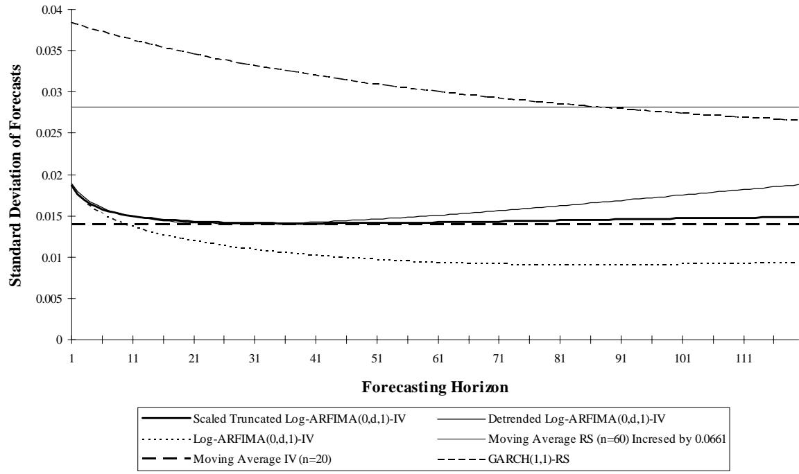
Figure 2B Standard Deviation of Forecasts of GARCH(1,1)-RS, Log-ARFIMA(0,d,1)-IV, Detrended Log-ARFIMA(0,d,1)-IV, Scaled Truncated Log-ARFIMA(0,d,1)-IV, Average RS, and Average IV British Steel Plc
