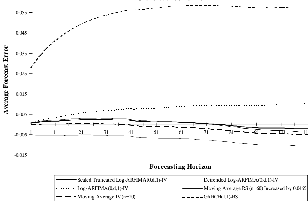
Figure 3A Average Forecast Error of GARCH(1,1)-RS, Log-ARFIMA(0,d,1)-IV, Detrended Log-ARFIMA(0,d,1)-IV, Scaled Truncated Log-ARFIMA(0,d,1)-IV, Averaged RS, and Averaged IV Glaxo Wellcome Plc
